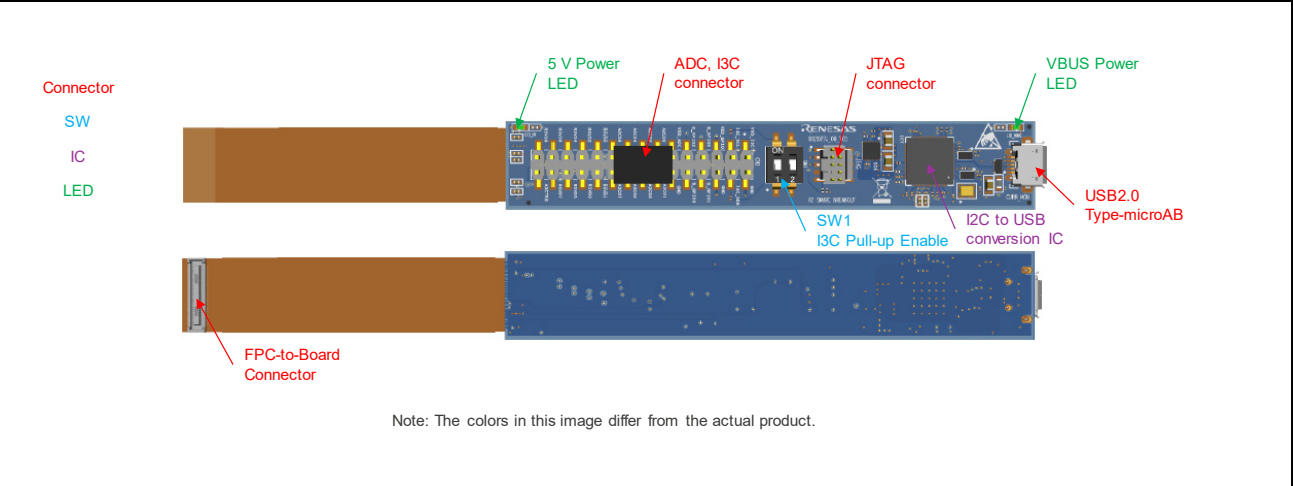
Figure 3.9 SMARC Breakout Adaptor Top and Bottom View
