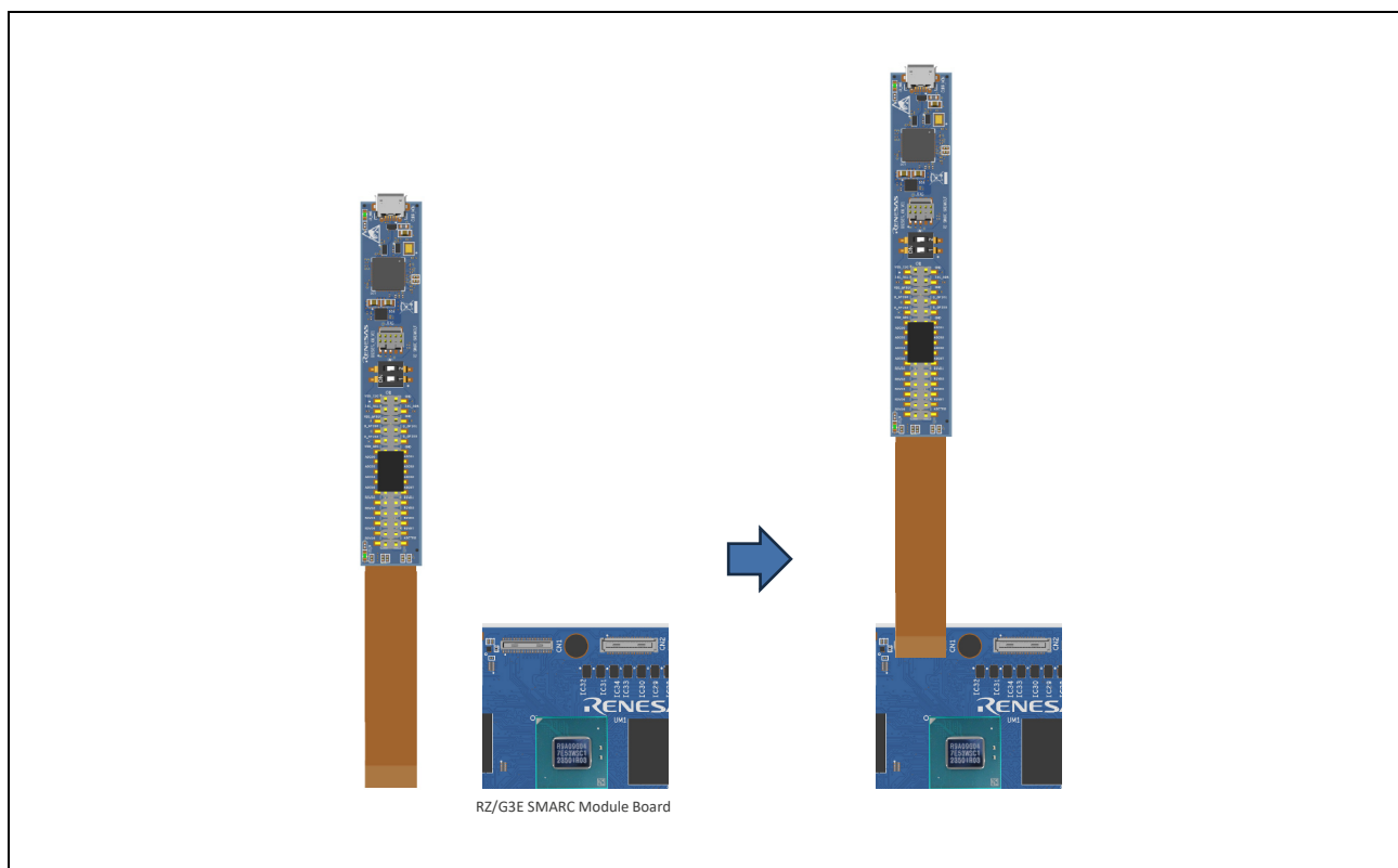
Figure 3.8 SMARC Breakout Adaptor Connection
