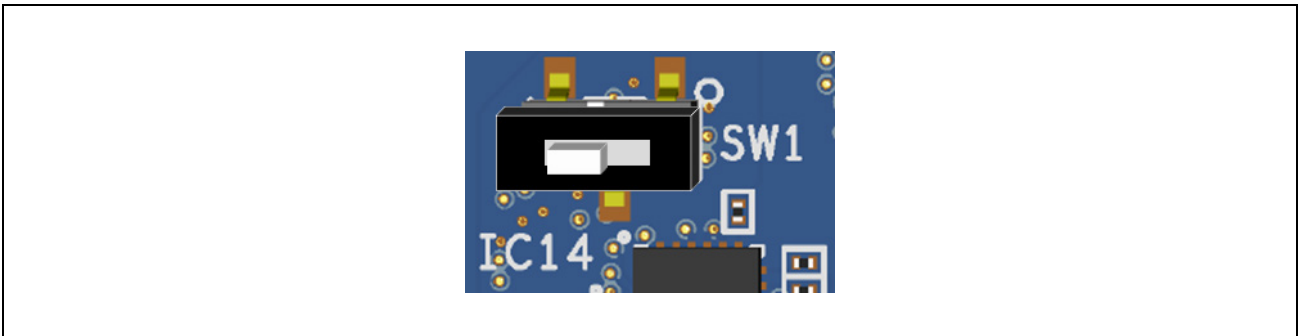
Figure 2.6 The Location and the Default Setting of SW1
