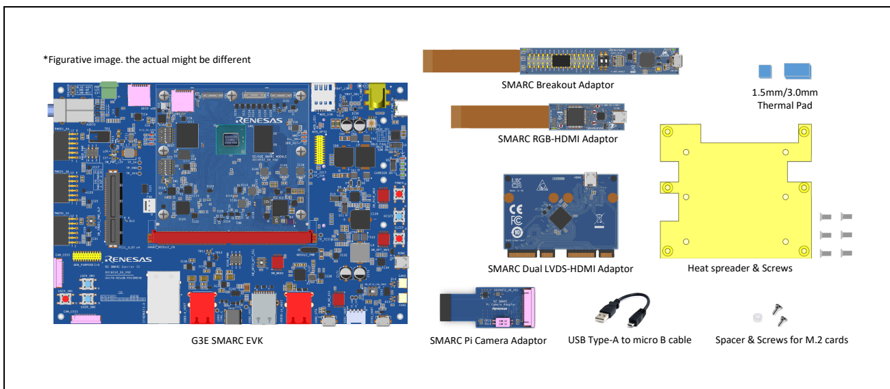
Figure 1.2 RZ/G3E SMARC Evaluation Board Kit Contents
