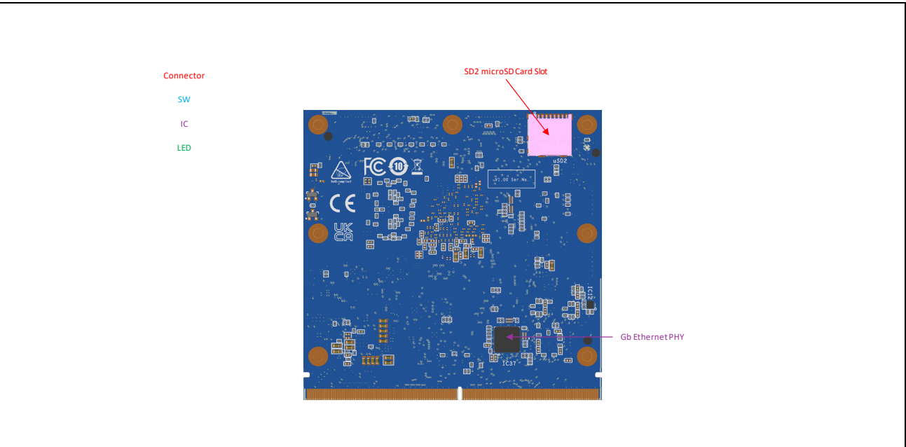
Figure 2.2 RZ/G3E SMARC Module Board Bottom View
