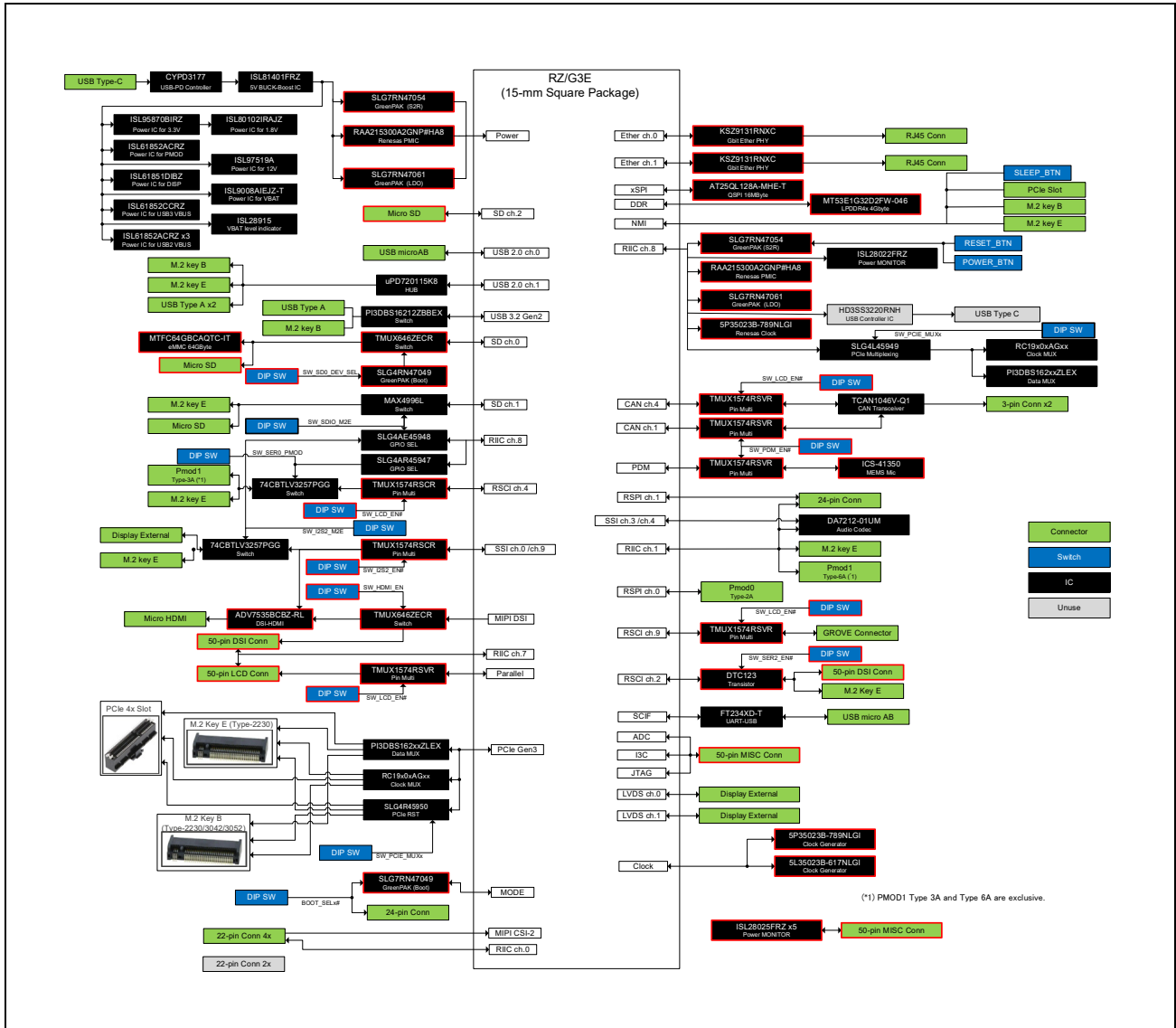
Figure 2.3 G3E SMARC EVK Block Diagram
