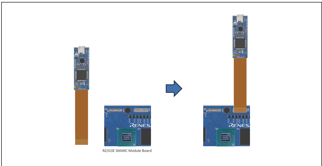
Figure 3.11 SMARC RGB-HDMI Adaptor Connection
