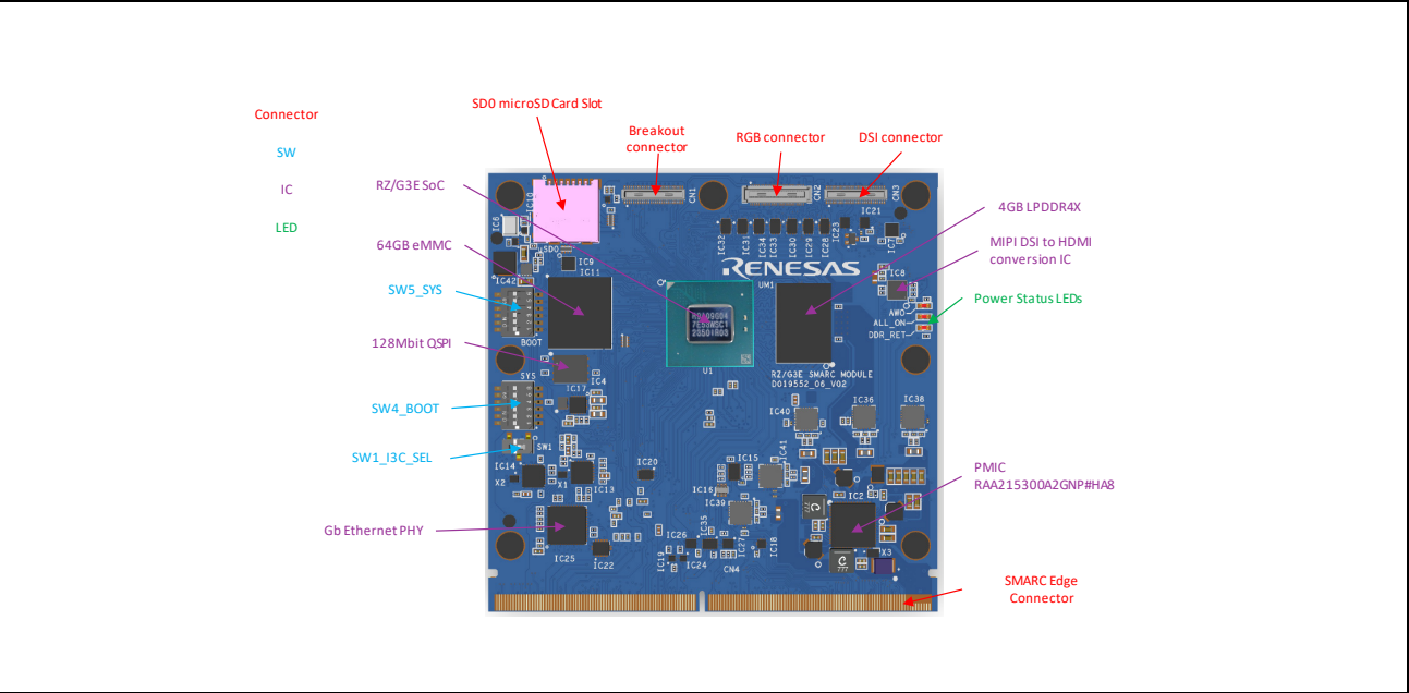
Figure 2.1 RZ/G3E SMARC Module Board Top View
