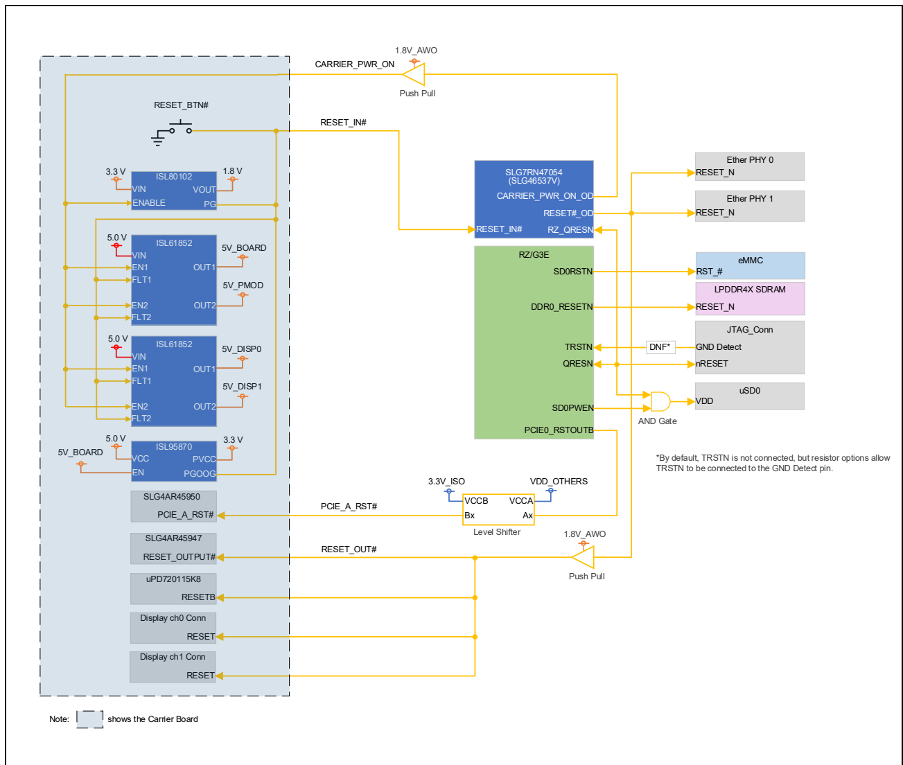
Figure 3.5 Reset Architecture of G3E SMARC EVK
