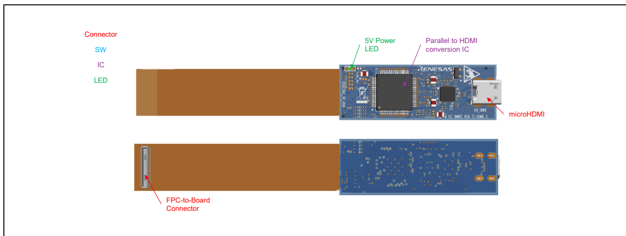
Figure 3.12 SMARC RGB-HDMI Adaptor Top and Bottom View
