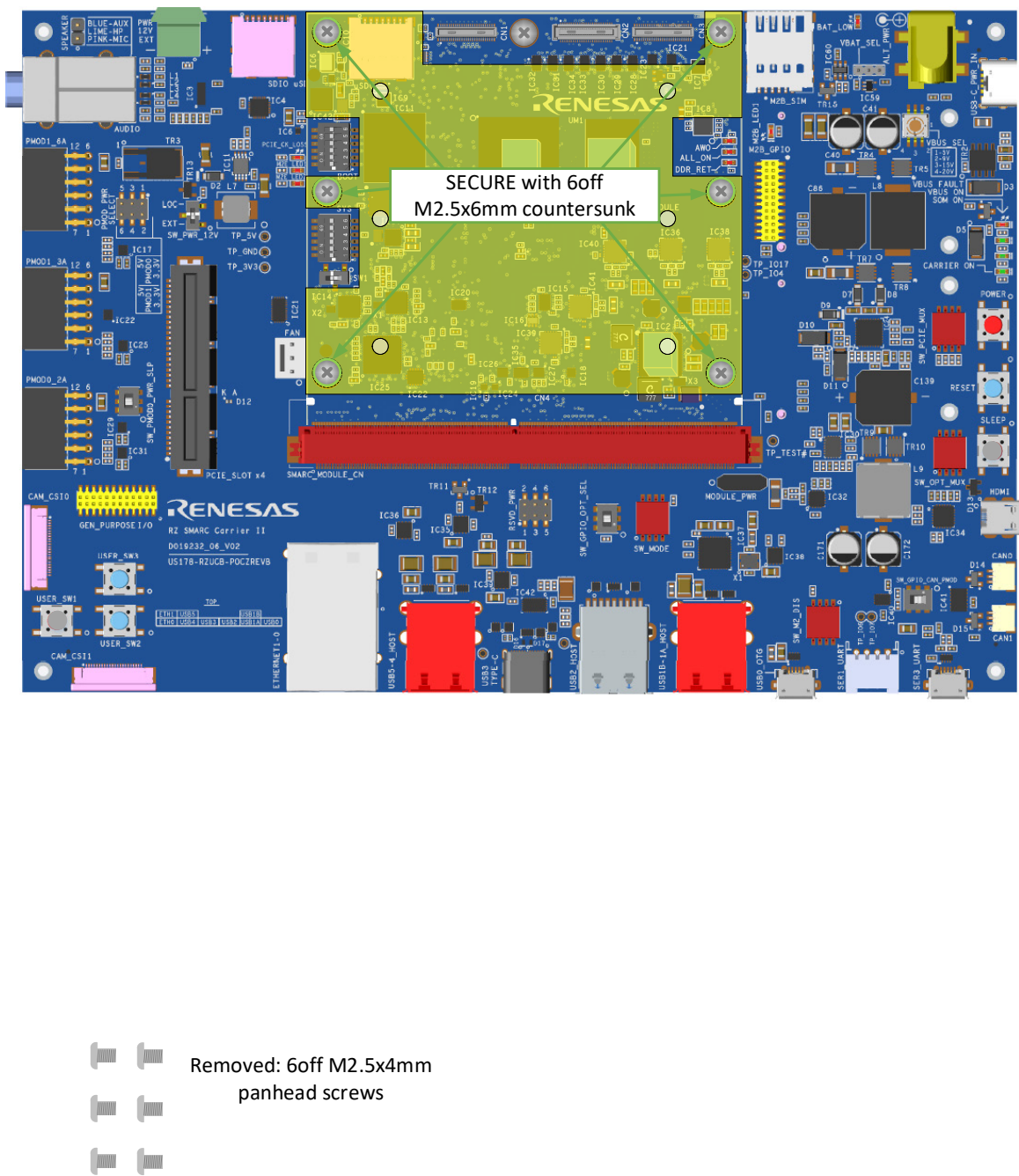
Figure A.4 How to Secure the Heat Spreader
