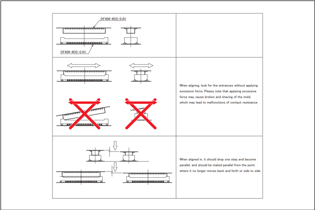
Figure B.2 Caution when Mating Breakout and RGB-HDMI Adaptor to Connector
