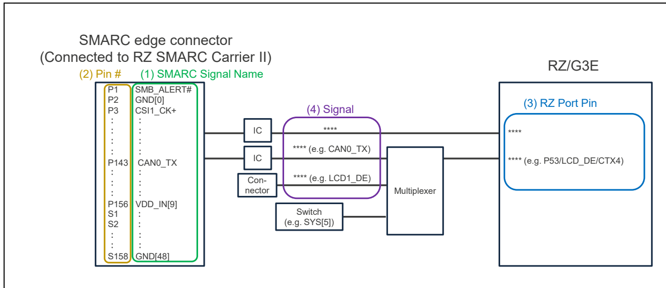
Figure 3.14 Signal Connections on the G3E SMARC Module among “SMARC Signal Name”, “Pin #”, “RZ Port Pin”, and “Signal”
