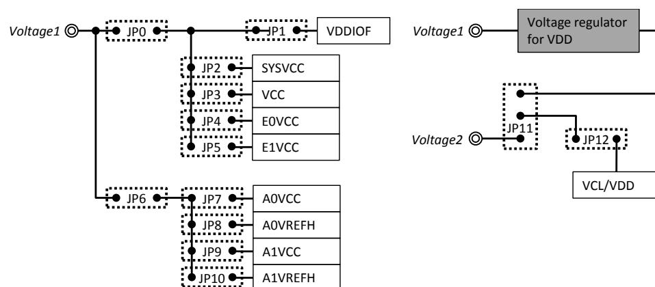
Figure 4 Voltage Distribution on the PiggyBack Board
