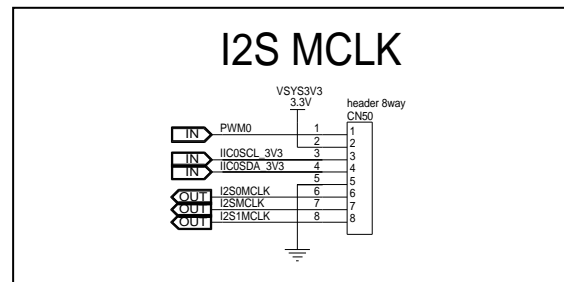
Figure 5.68 Connector for master clock generation
