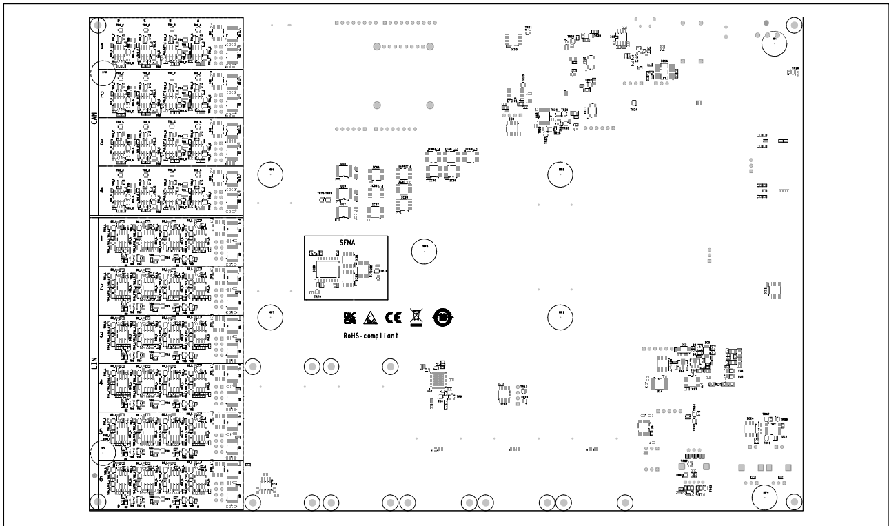
Figure 2.1 Placement of switches, connectors and LEDs on bottom side of board version D019712_06_V01
