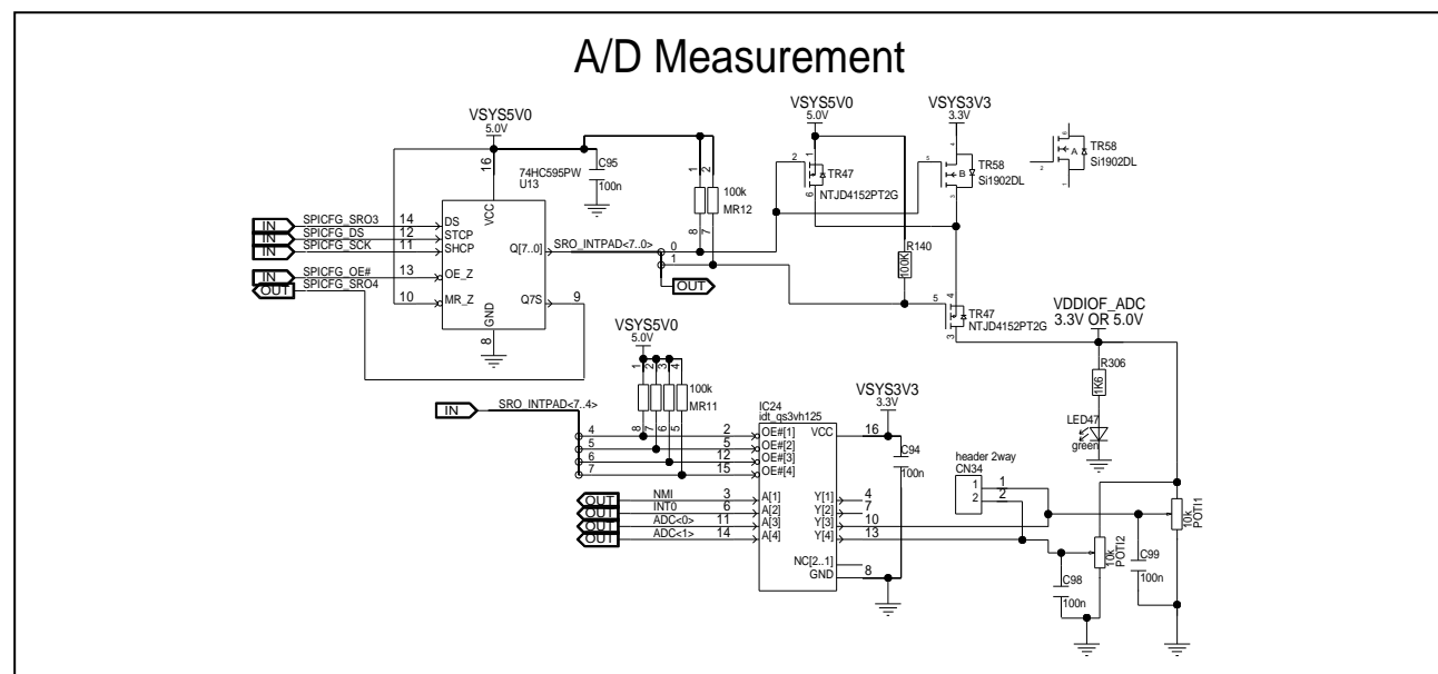
Figure 5.66 A/D measurements of board version D019712_06_V02 and later
