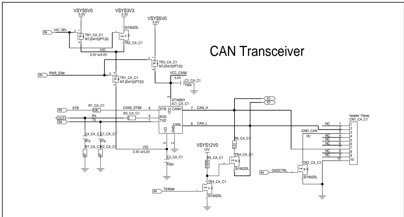
Figure 5.7 Circuit diagram CAN transceiver of board version D019712_06_V02 and later
