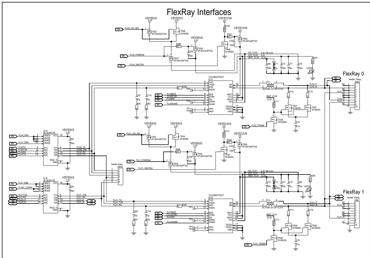
Figure 5.18 FlexRay interface circuit diagram of board version D019712_06_V04 and later
