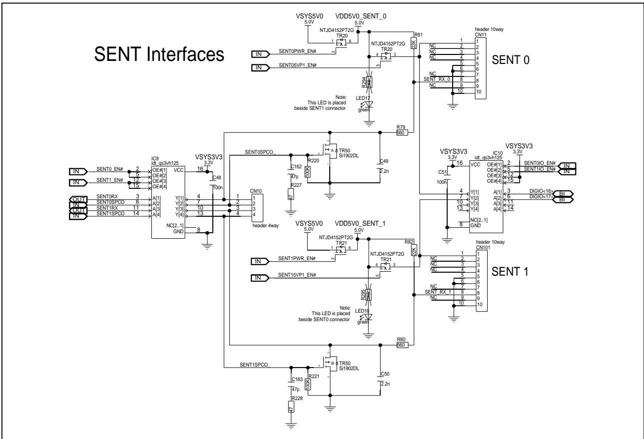
Figure 5.33 SENT interfaces of board version D019712_06_V02
