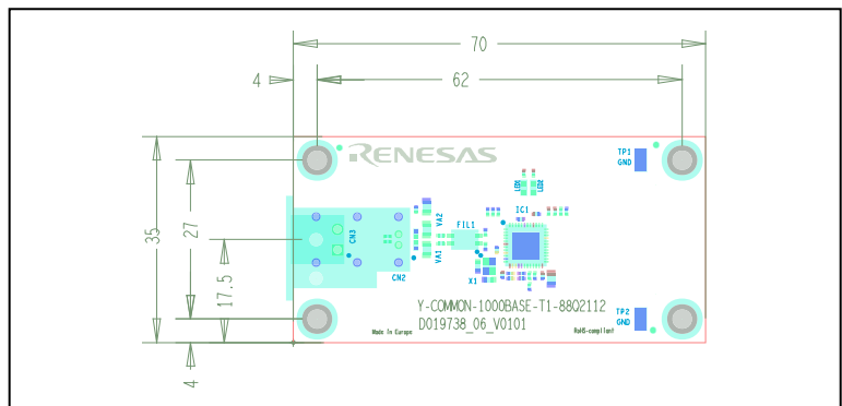
Figure 5.25 Y-COMMON-1000BASE-T1-88Q2112 dimensions
