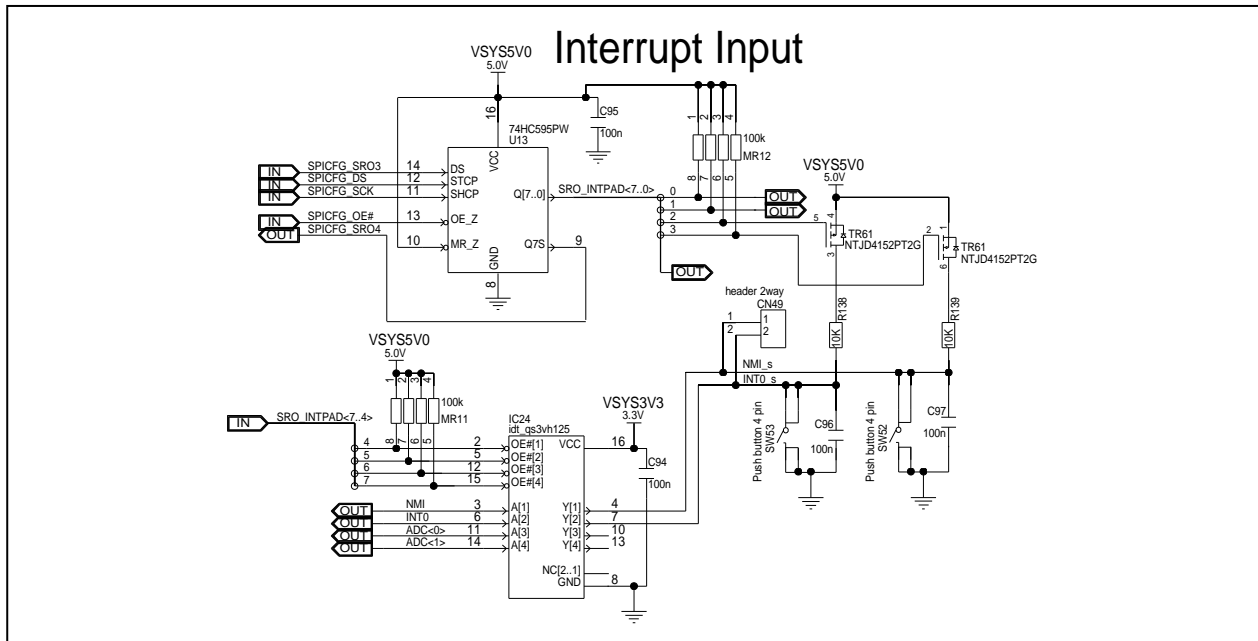
Figure 5.64 Interrupts push buttons
