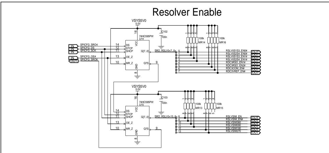
Figure 5.60 Resolver enable signals of board version D019712_06_V01 and D019712_06_V02
