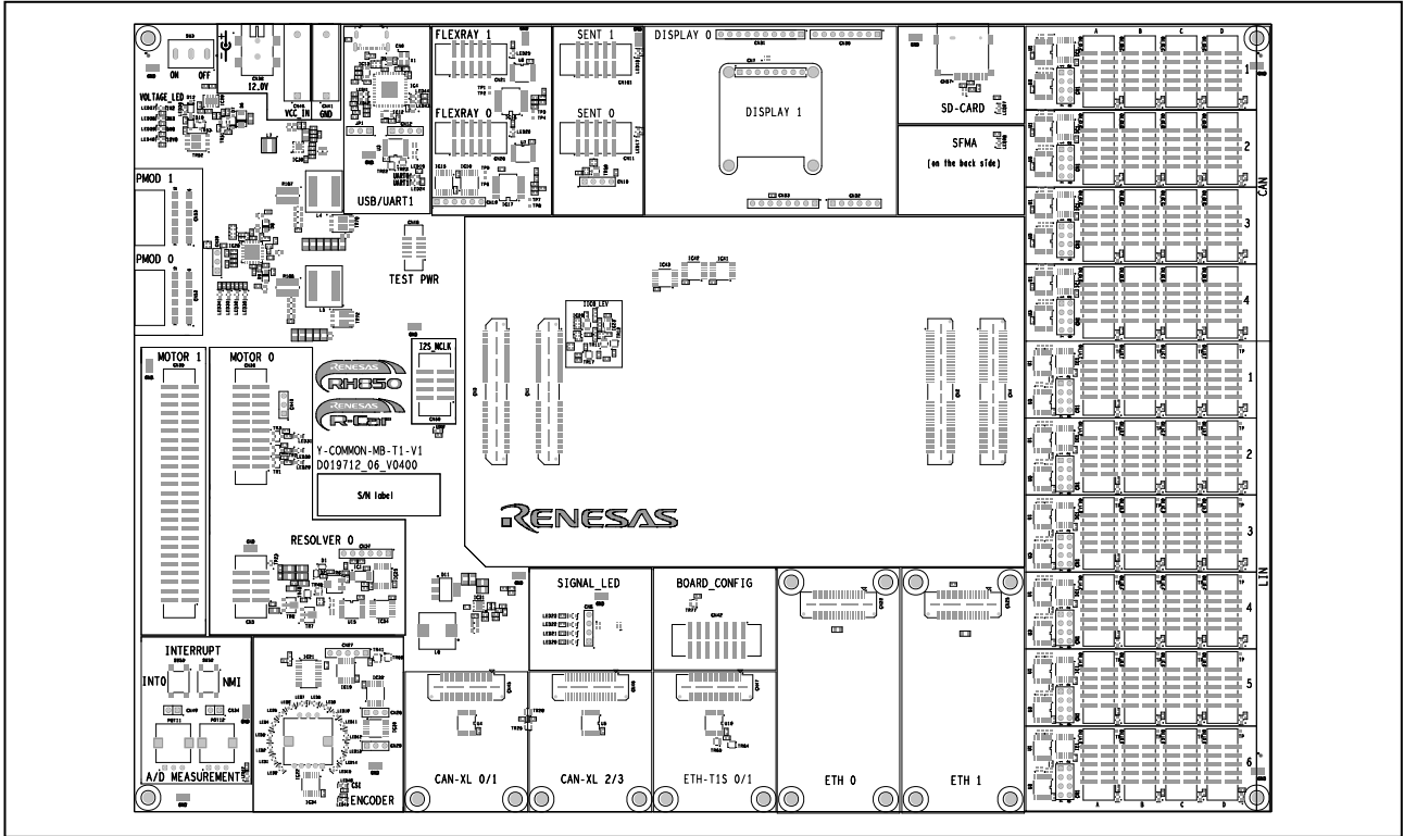
Figure 2.7 Placement of switches, connectors and LEDs on bottom side of board version D01912_06_V04
