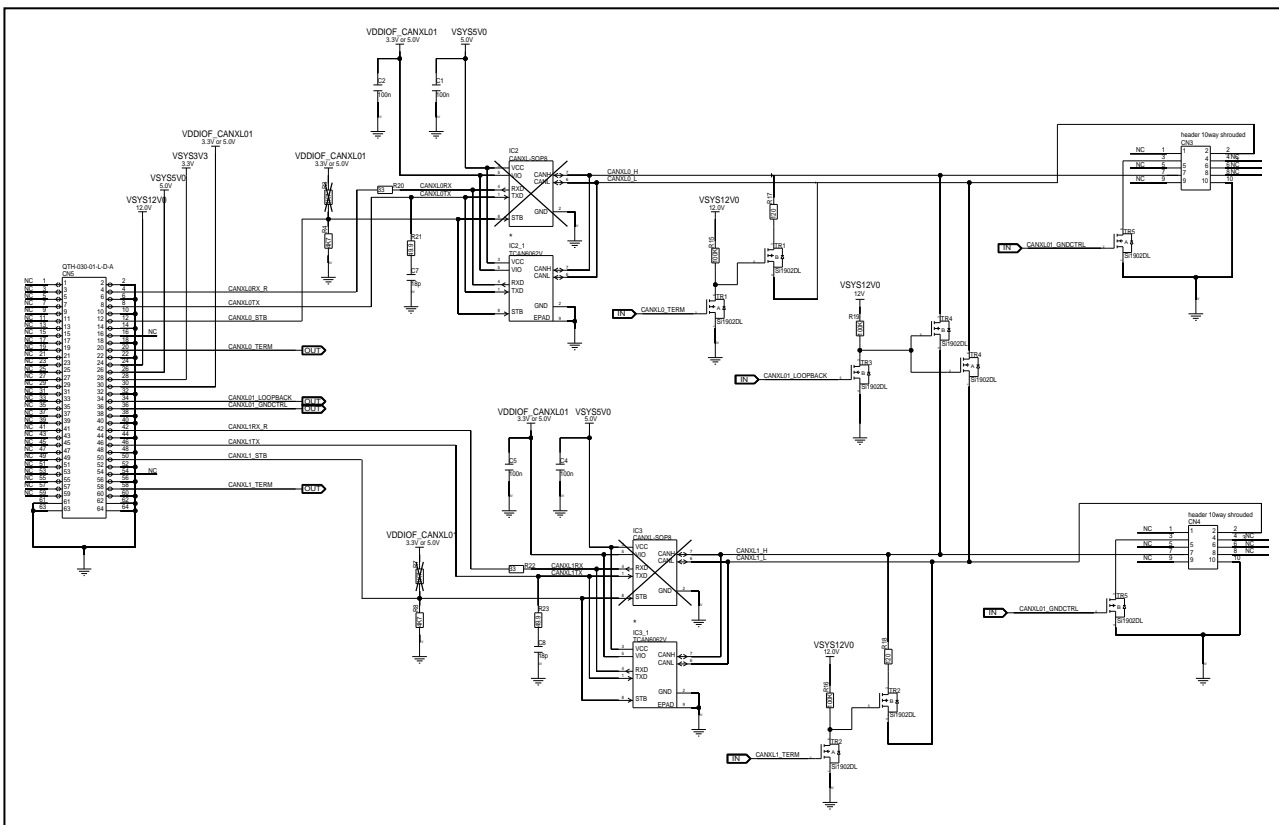
Figure 5.11 Y-COMMON-CANXL-TCAN6062V board circuit diagram
