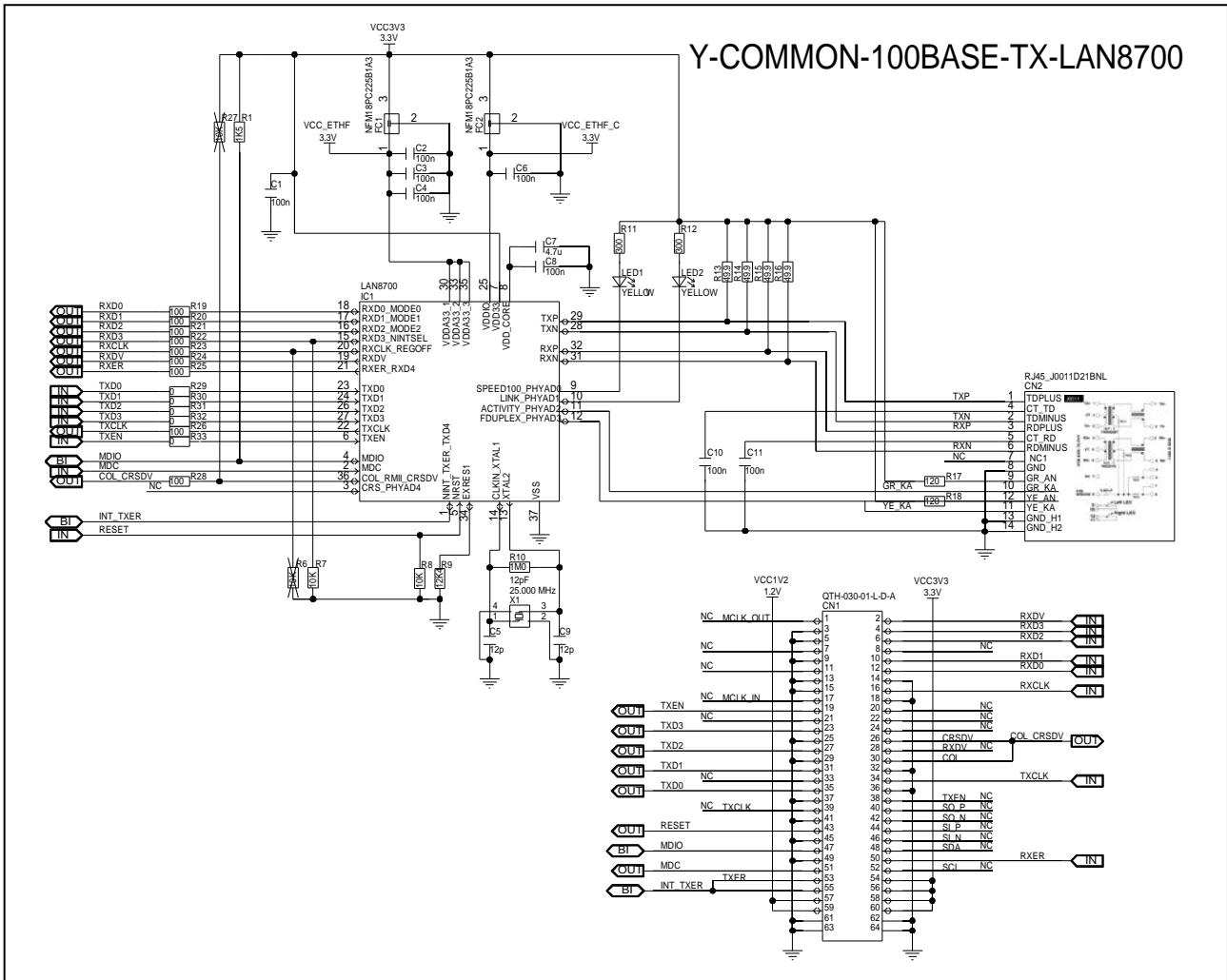
Figure 5.22 Circuit diagram of Renesas Ethernet board Y-COMMON-100BASE-TX-LAN8700 Figure 5.23 Y-COMMON-100BASE-TX-LAN8700 dimensions
