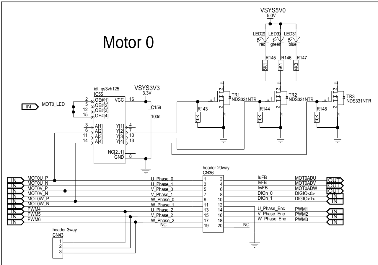
Figure 5.58 Motor control circuit Motor 0 of board versions D019712_06_V03 and later
