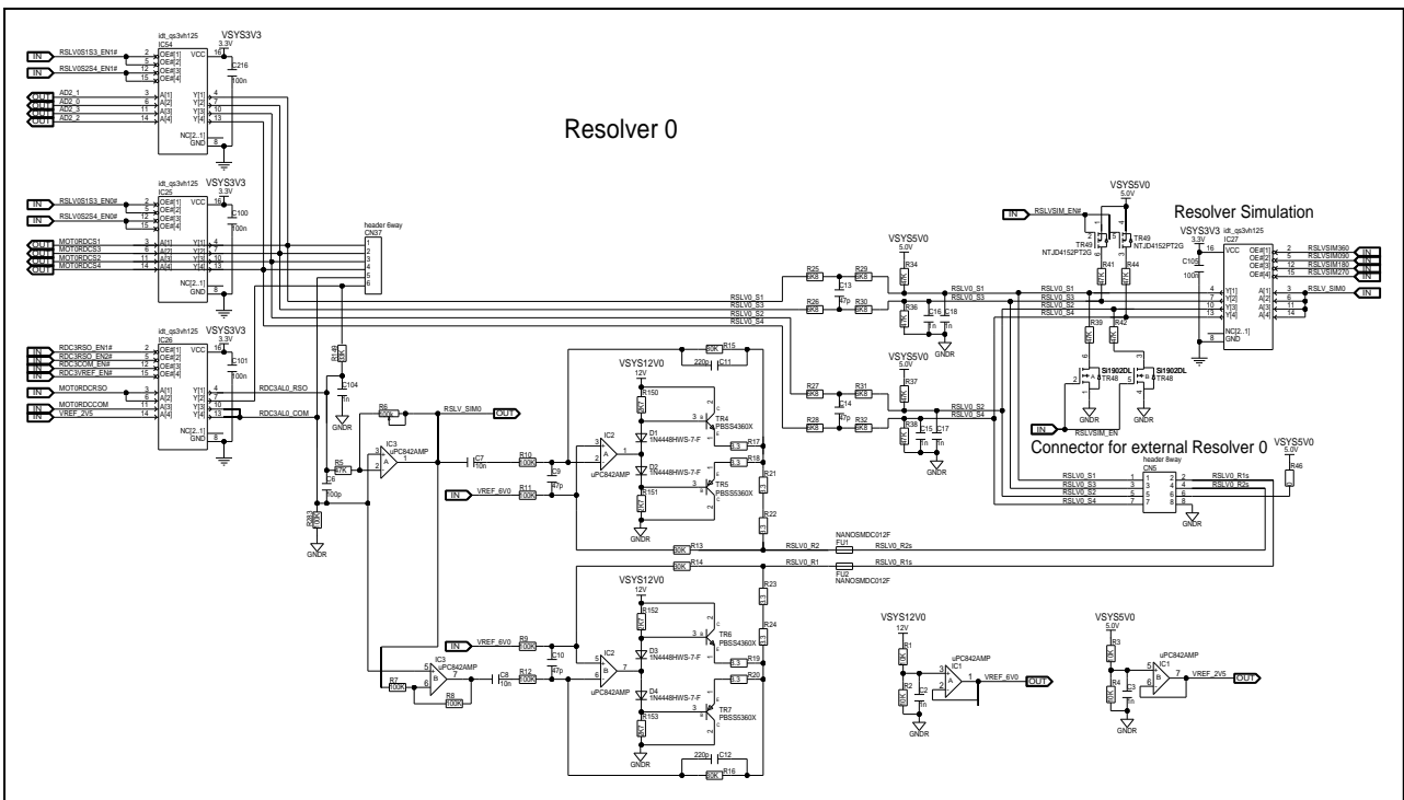
Figure 5.63 Circuit diagram resolver circuit of board version D019712_06_V03
