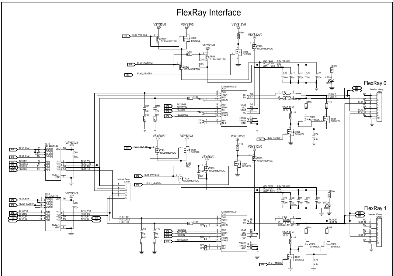
Figure 5.16 FlexRay interface circuit diagram of board version D019712_06_V02
