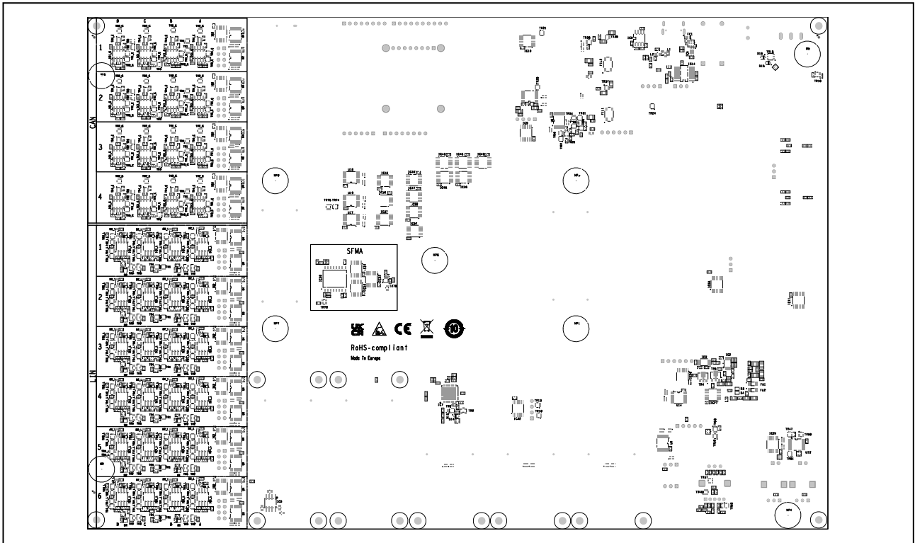
Figure 2.8 Placement of switches, connectors and LEDs on top side of board version D01912_06_V04
