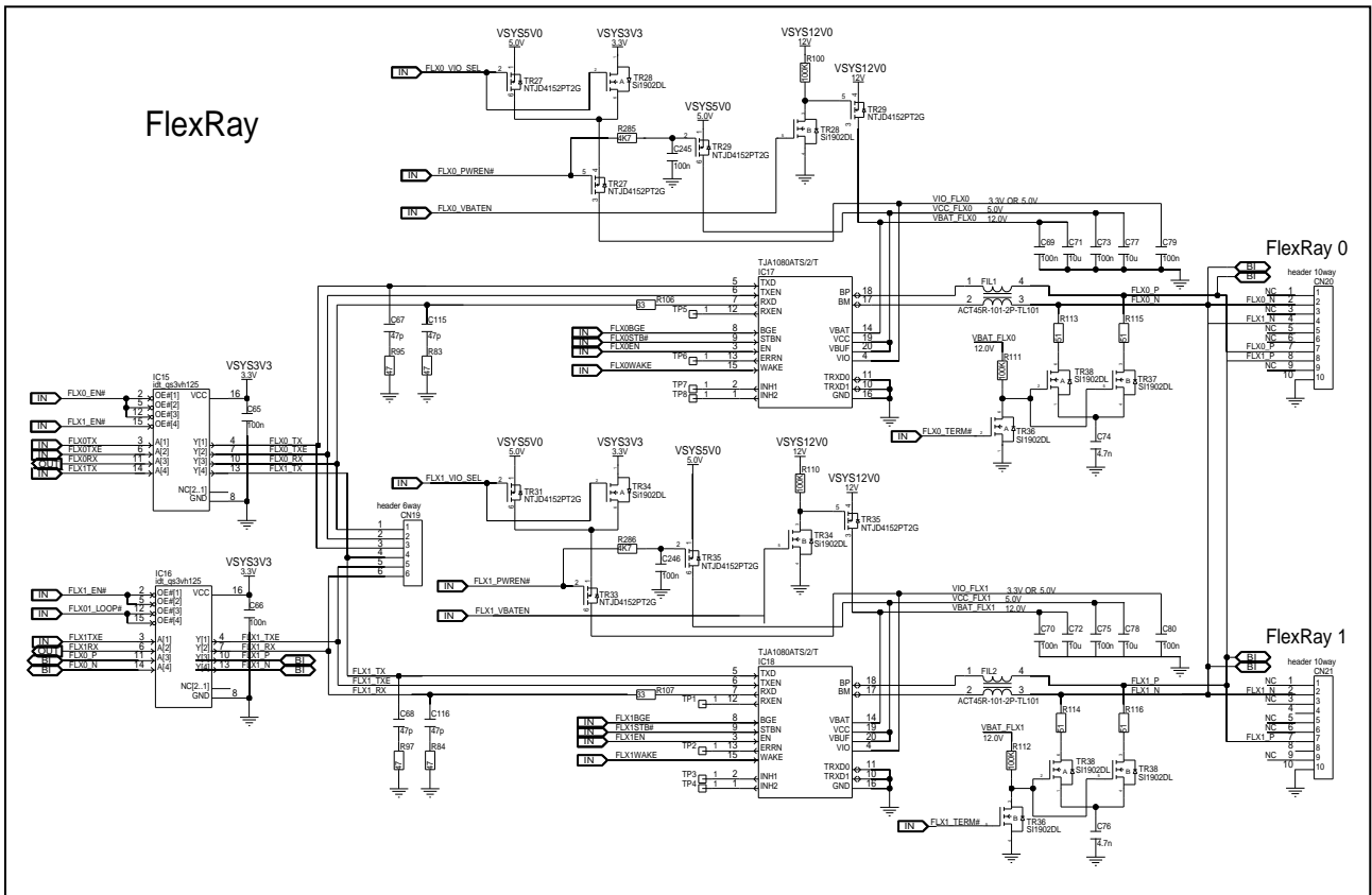
Figure 5.15 FlexRay interface circuit diagram of board version D019712_06_V01
