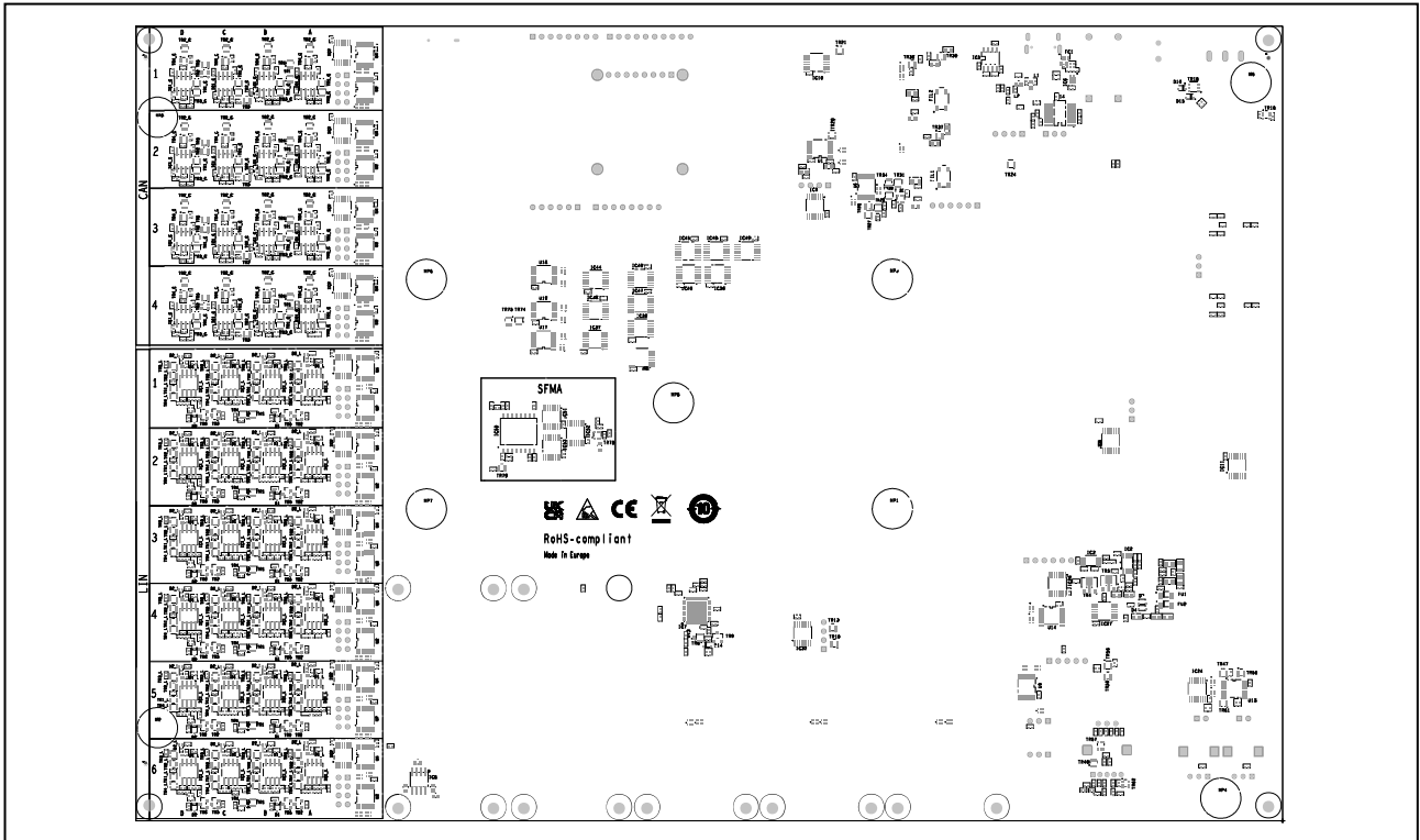
Figure 2.5 Placement of switches, connectors and LEDs on top side of board version D019712_06_V03
