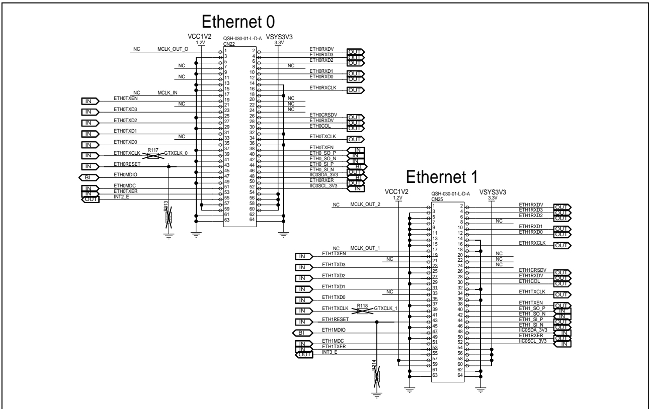
Figure 5.21 Ethernet module connector circuit for MII/SGMII compliant Ethernet modules of board version D019712_06_V03 and later
