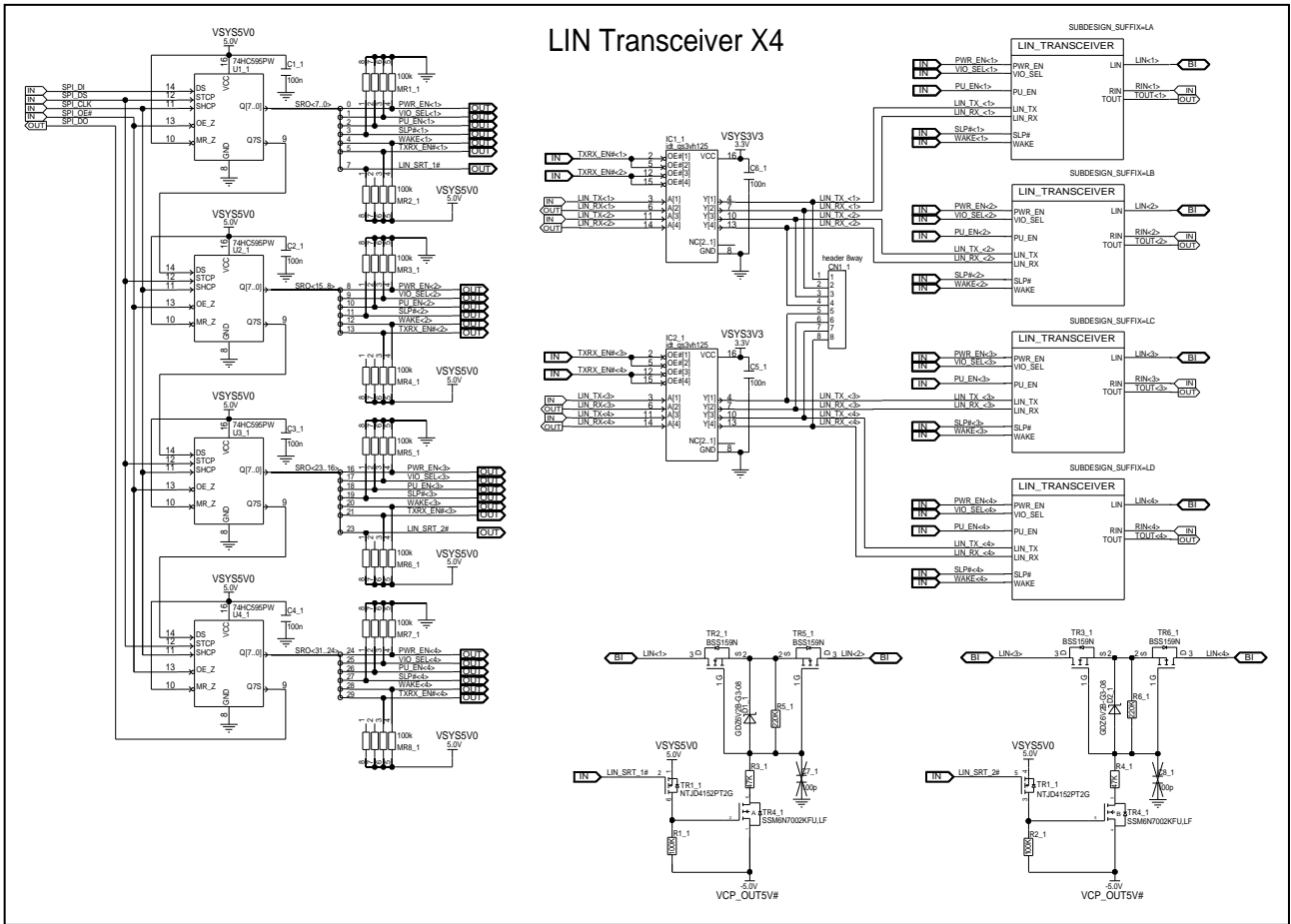
Figure 5.3 Circuit diagram LIN transceiver block X4
