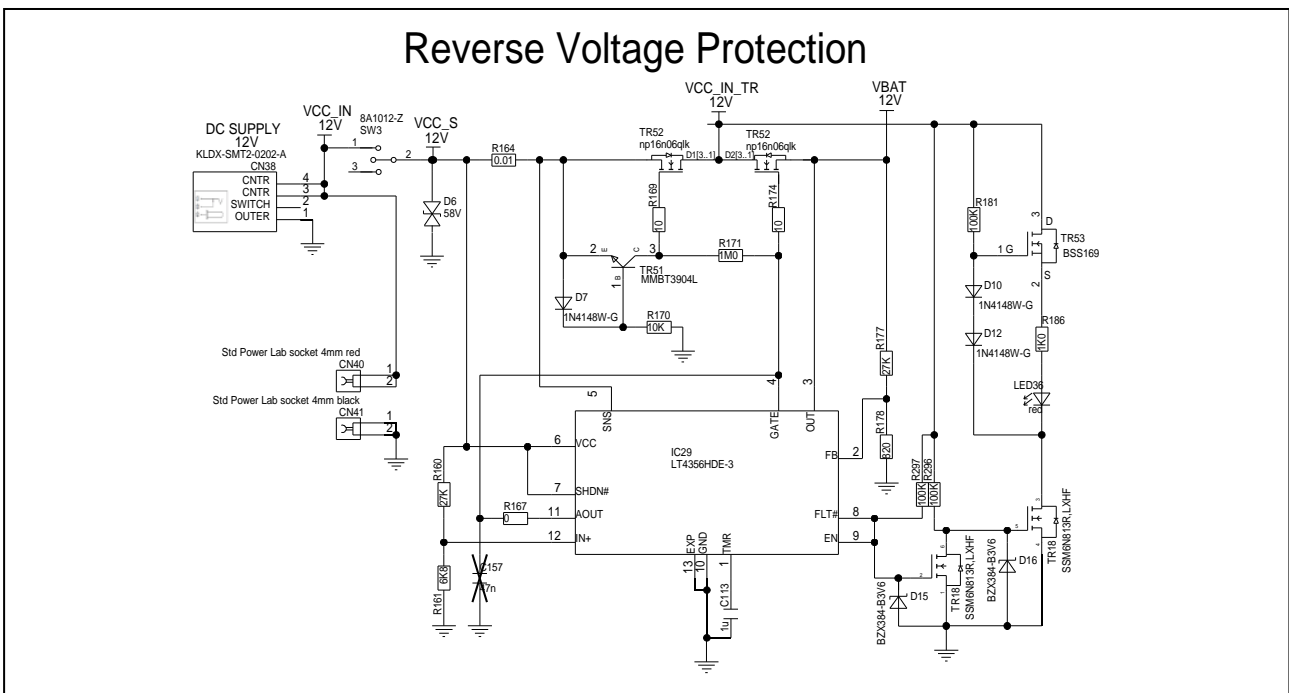
Figure 3.3 Connection of power supply and board protection circuit of board version D019712_06_V02 and later
