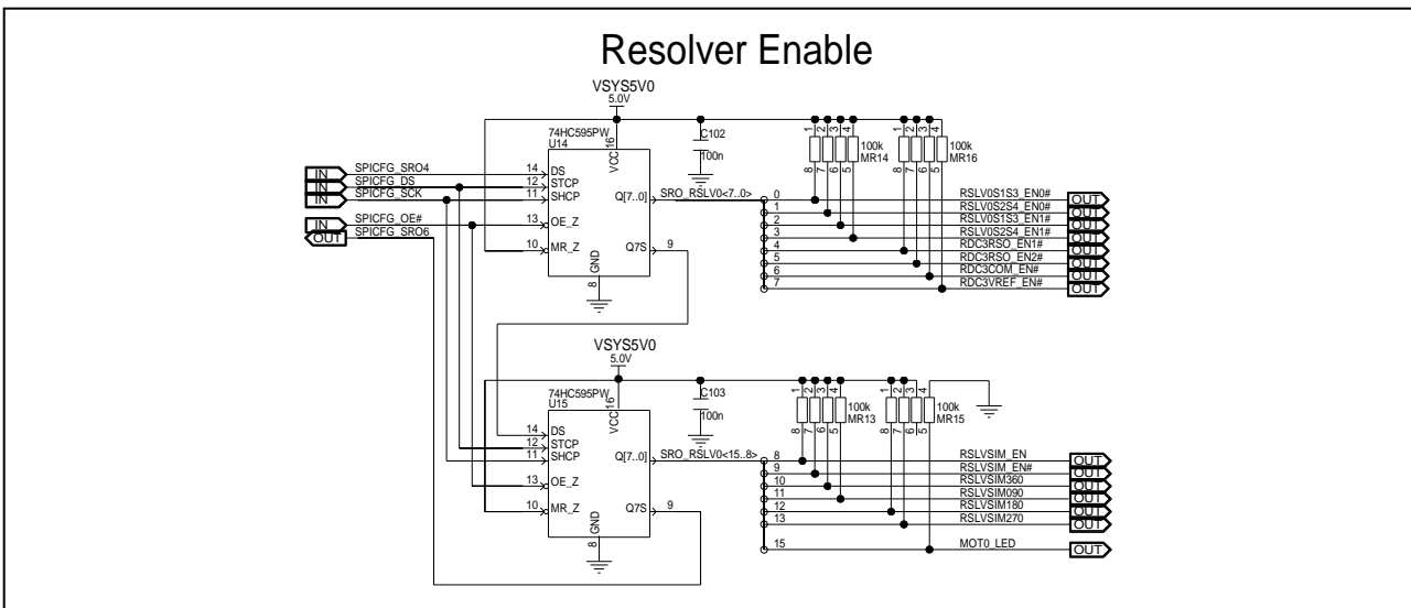
Figure 5.61 Resolver enable signals of board version D019712_06_V03
