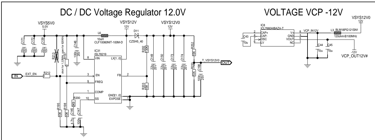
Figure 3.5 Voltage regulator +- 12.0V
