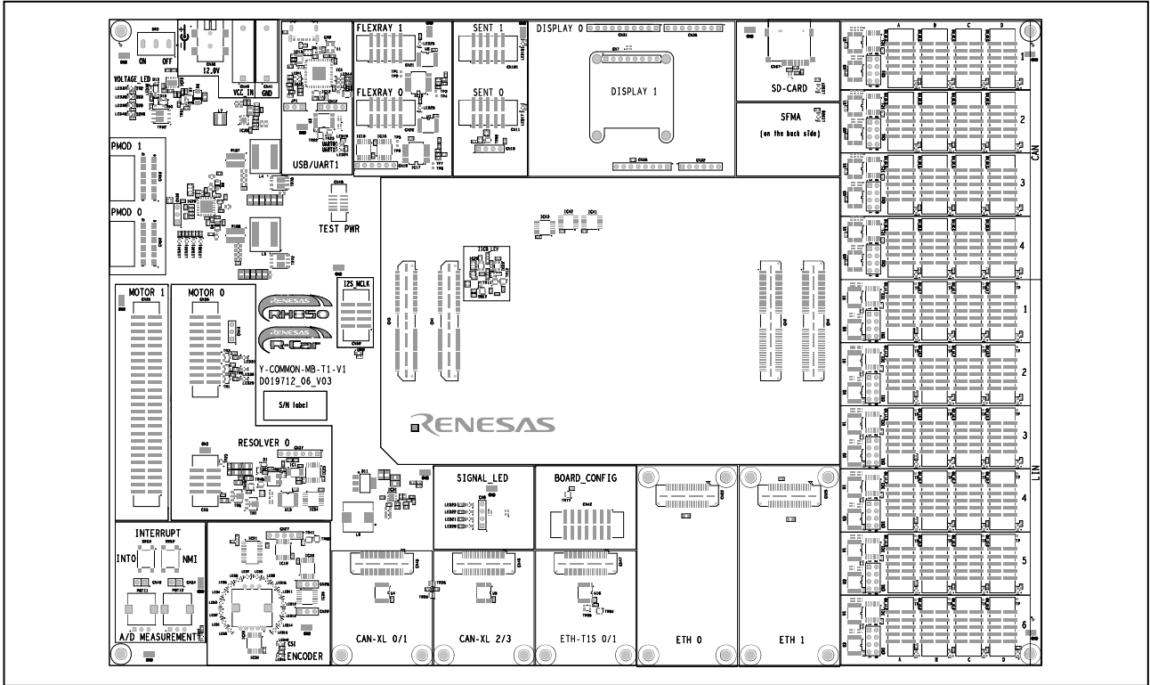
Figure 2.6 Placement of switches, connectors and LEDs on bottom side of board version D019712_06_V03
