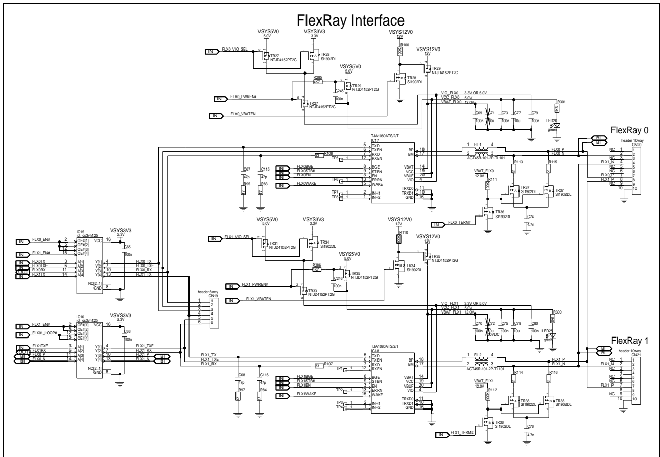
Figure 5.17 FlexRay interface circuit diagram of board version D019712_06_V03
