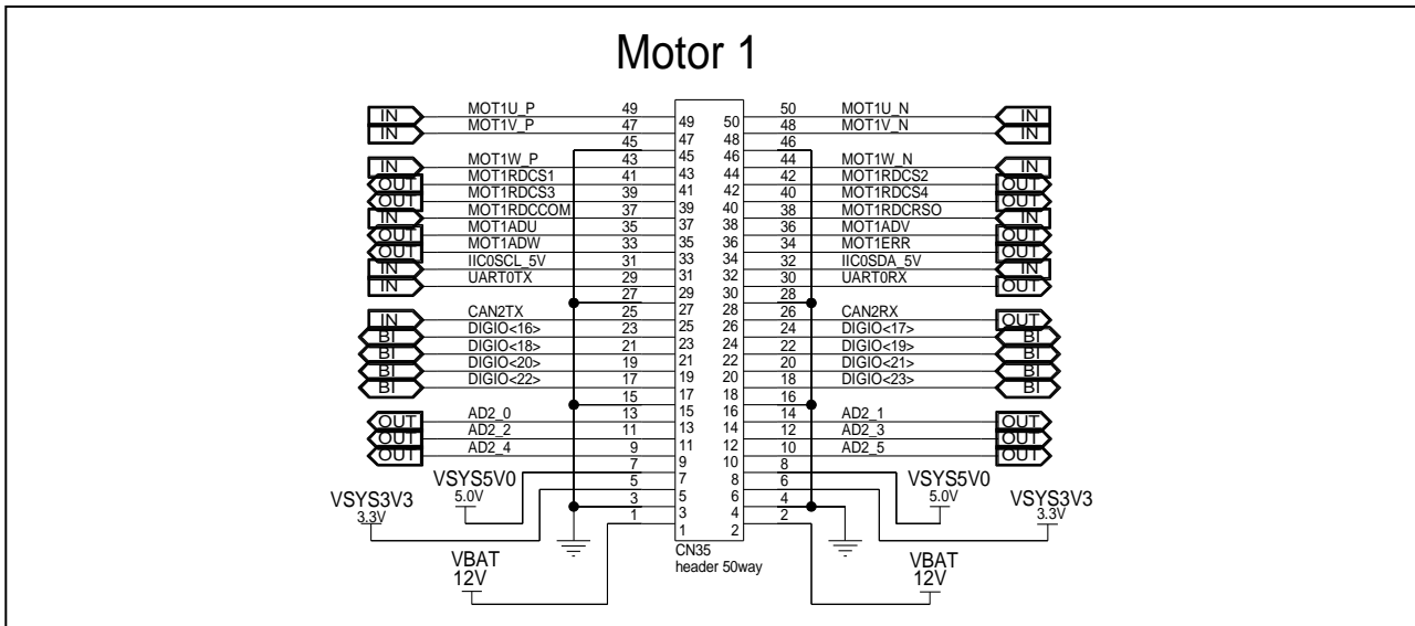
Figure 5.57 Motor control circuit Motor 1
