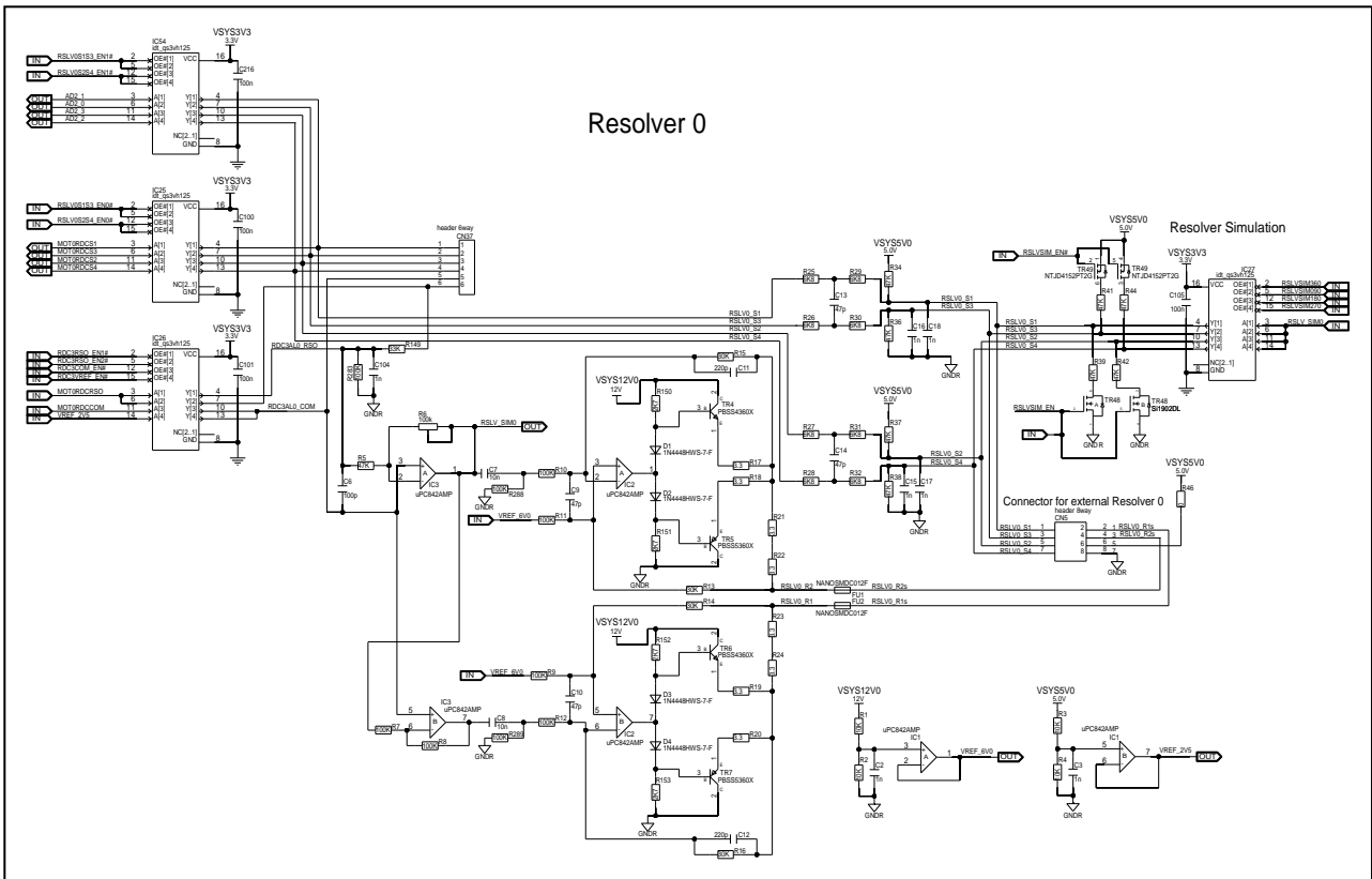
Figure 5.62 Circuit diagram resolver circuit of board version D019712_06_V01 and D019712_06_V02
