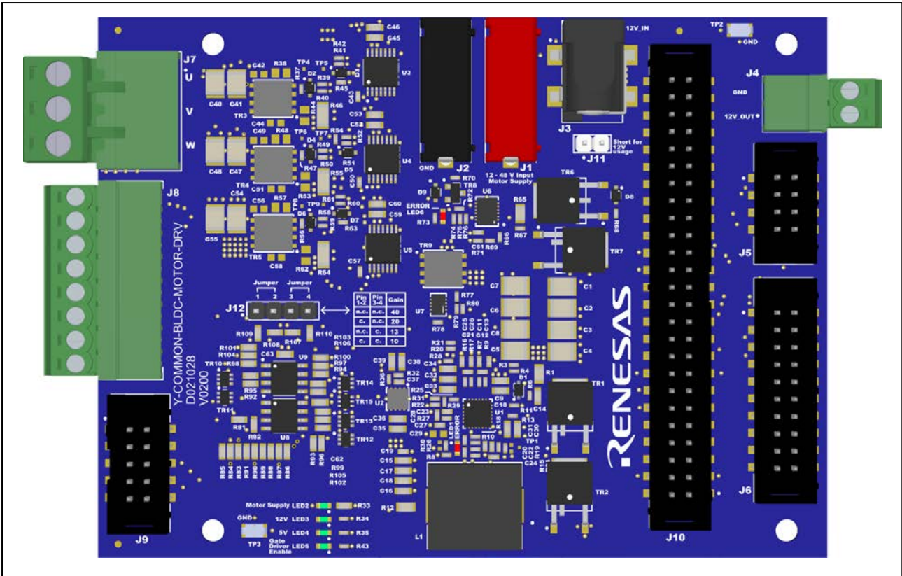
Figure 5.59 Connectors on the motor control extension board
