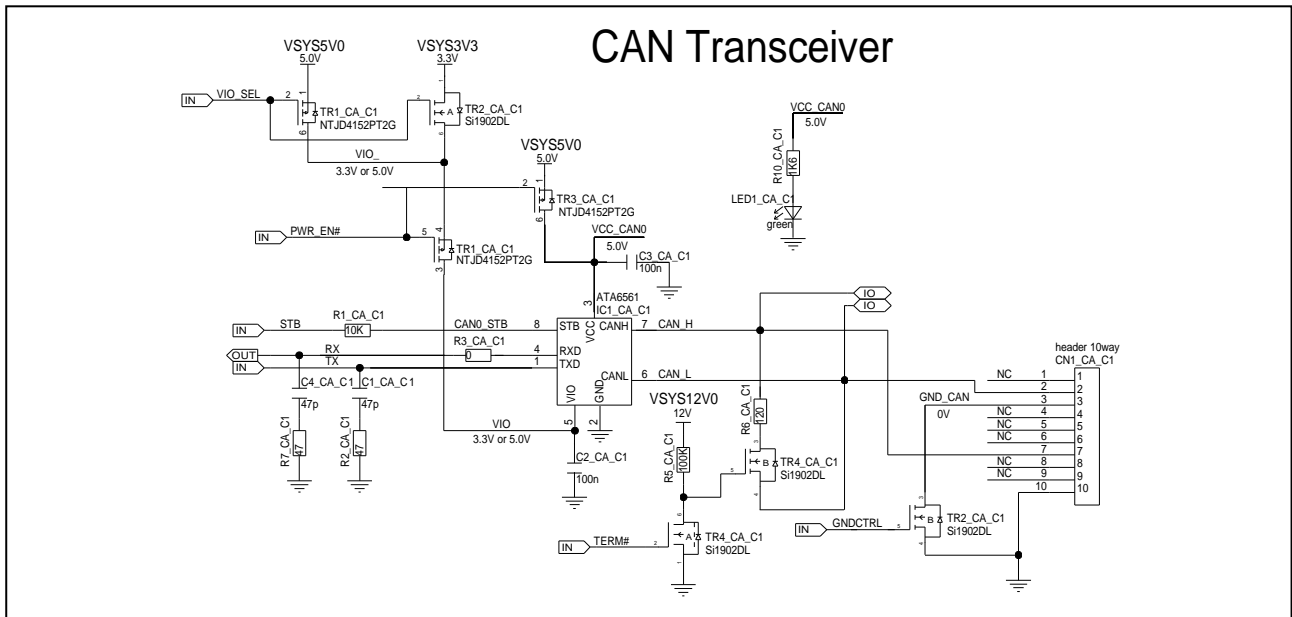
Figure 5.8 Circuit diagram CAN transceiver of board version D019712_06_V01
