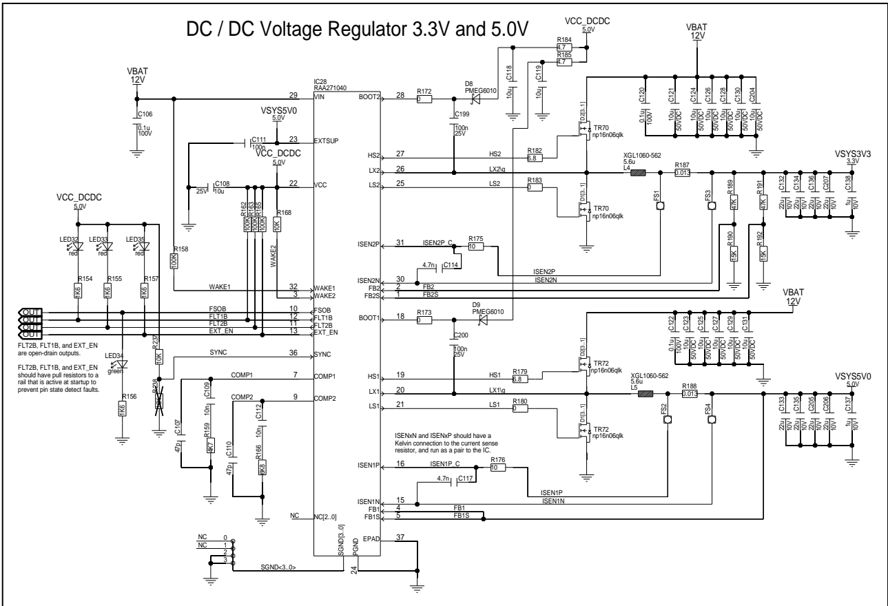
Figure 3.6 Voltage regulator 3.3V / 5.0V
