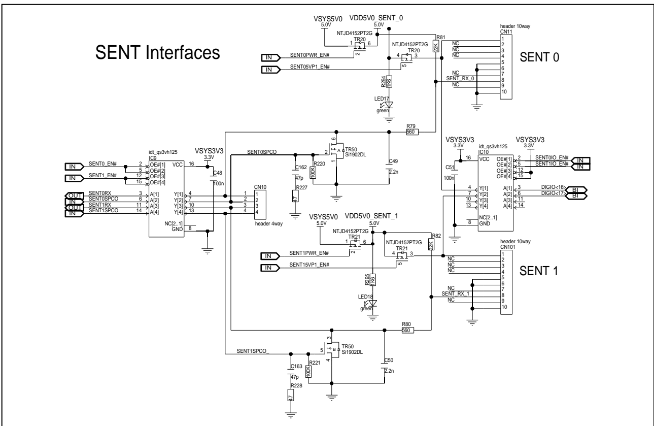
Figure 5.32 SENT interfaces of board version D019712_06_V03 and later
