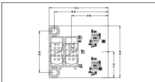
Figure 5.12 Y-COMMON-CANXL-NN dimensions
