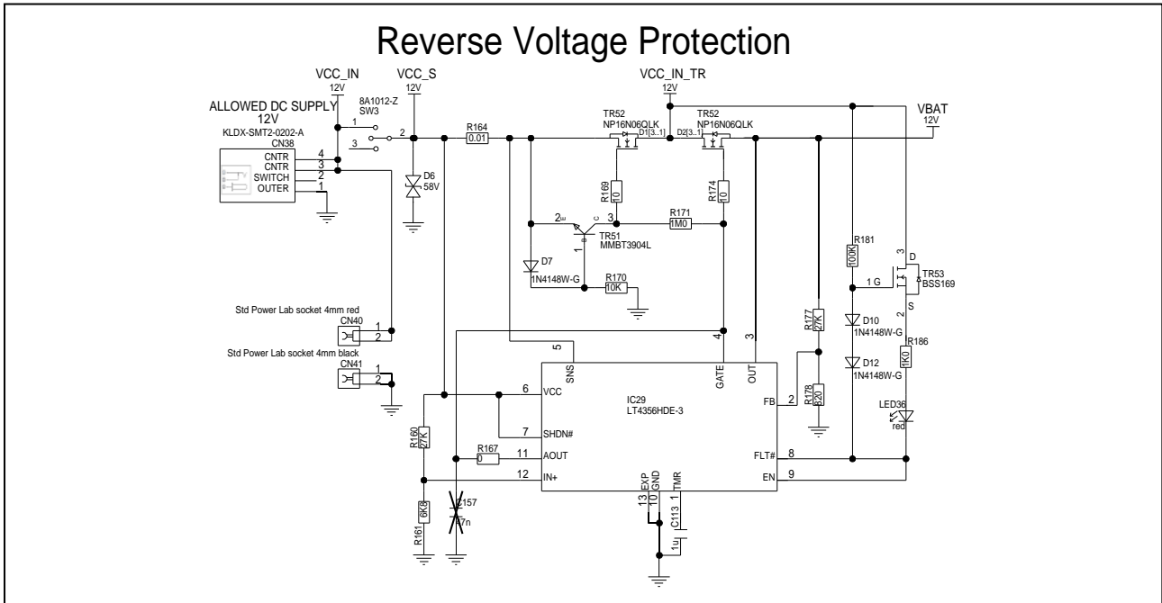
Figure 3.4 Connection of power supply and board protection circuit of board version D019712_06_V01
