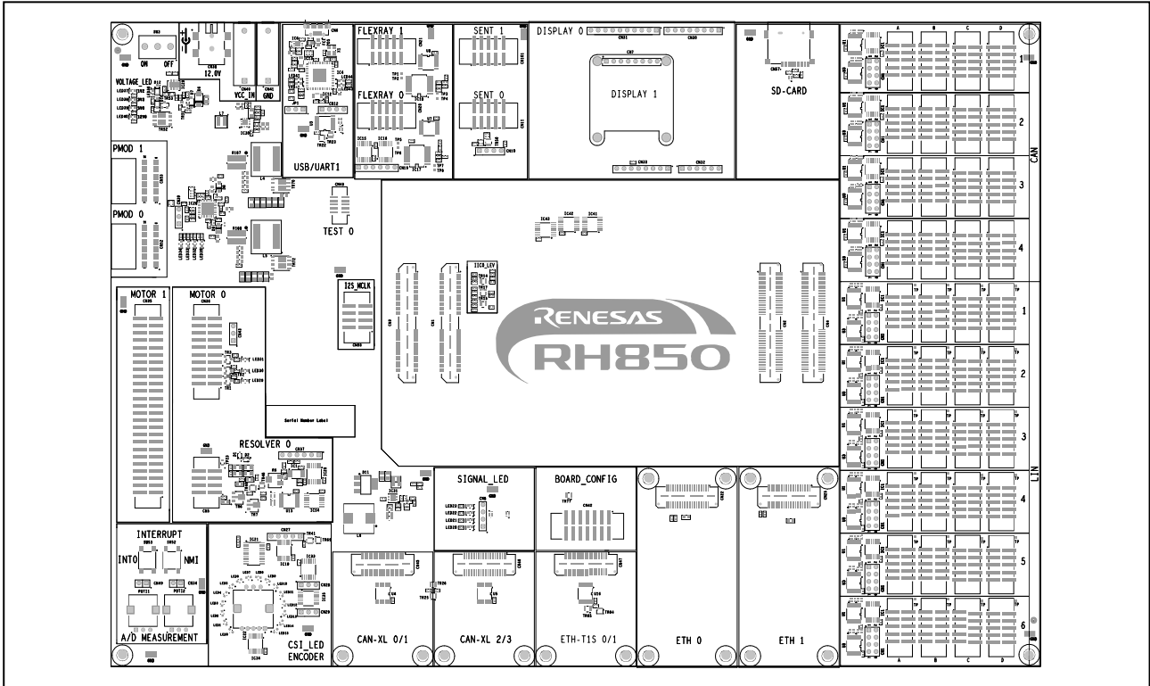
Figure 2.2 Placement of switches, connectors and LEDs on top side of board version D019712_06_V01
