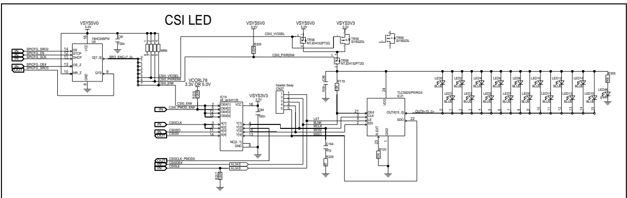
Figure 5.54 LED CSI driver for LED ring indicator of board version D019712_06_V02 and later
