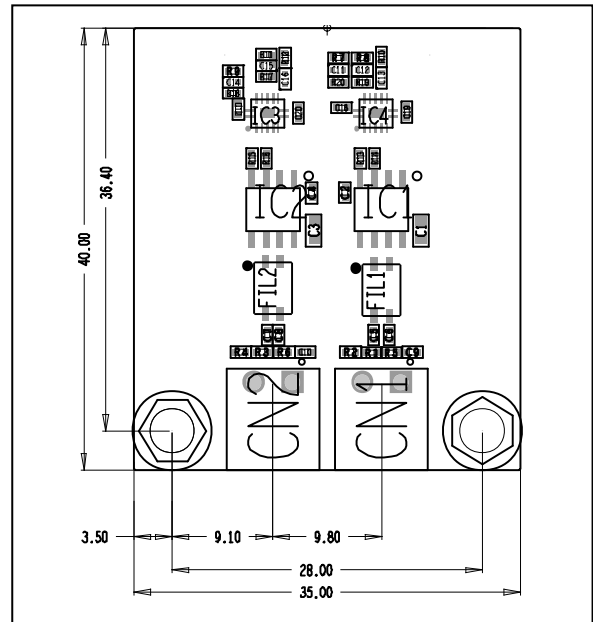
Figure 5.29 Y-COMMON-10BASE-T1S-NN dimensions
