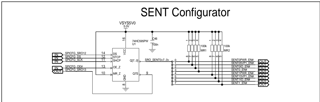
Figure 5.31 SENT interface configurator
