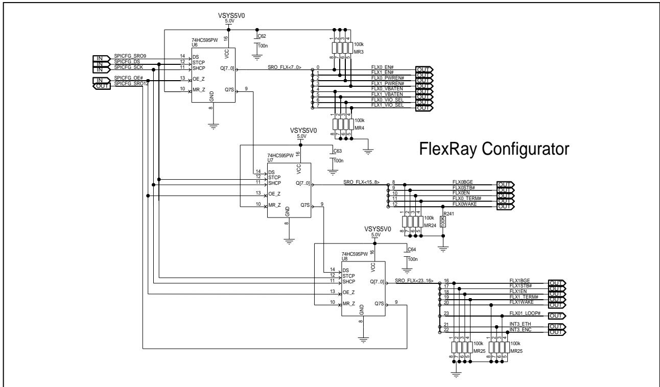
Figure 5.13 FlexRay configurator circuit diagram of board version D019712_06_V03 and later
