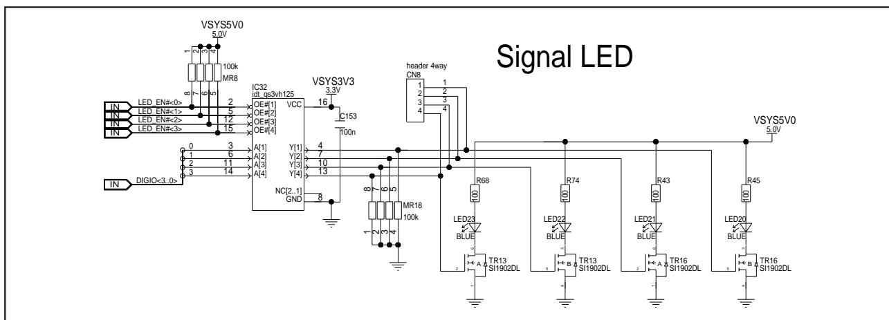
Figure 5.67 Signal LEDs
