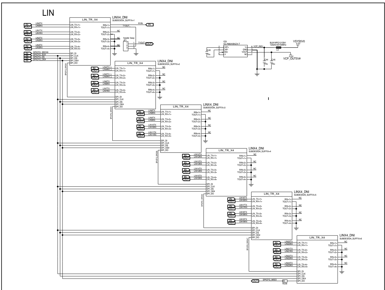
Figure 5.1 Circuit diagram LIN interfaces
