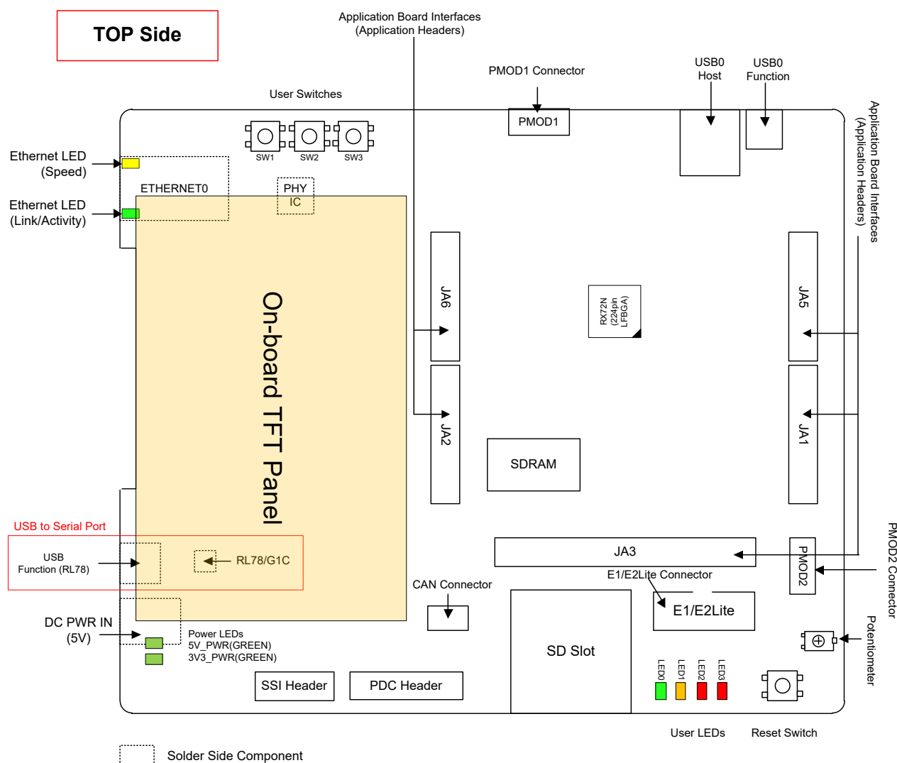
Figure 3-1: Board Layout
