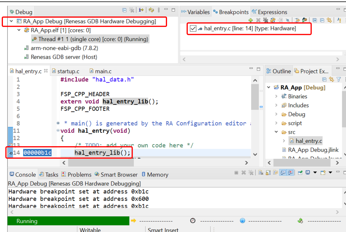
Figure 57. Application Project Executing Library Function
