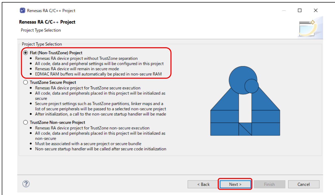
Figure 35. Project Type Selection
