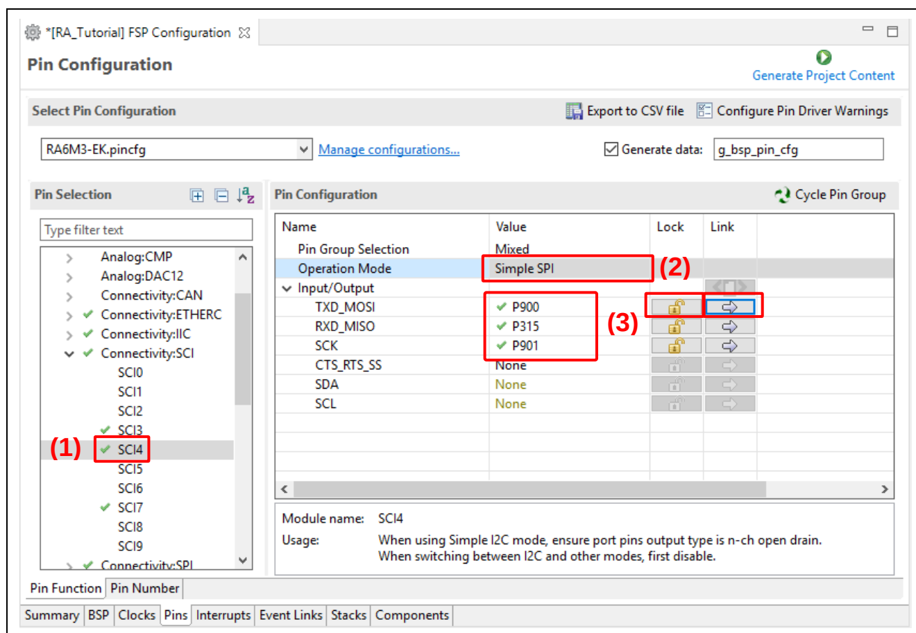
Figure 67. RA Project Configuration – Pin Configuration Setting (By Peripheral)
