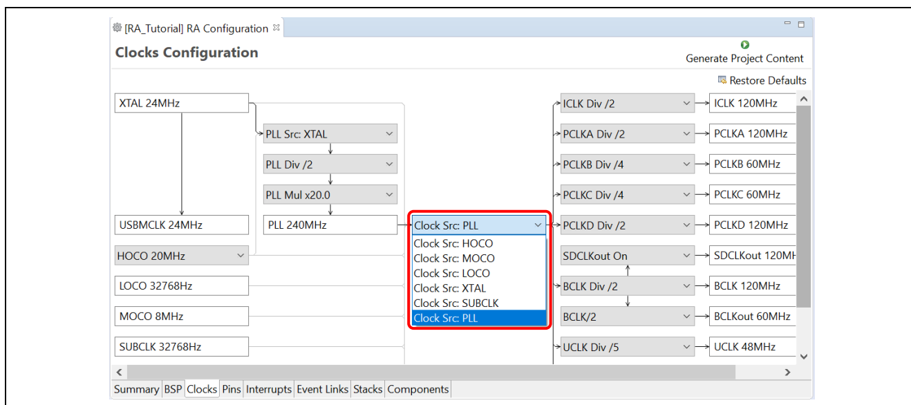
Figure 62. RA Project Configuration – Clocks Configuration
