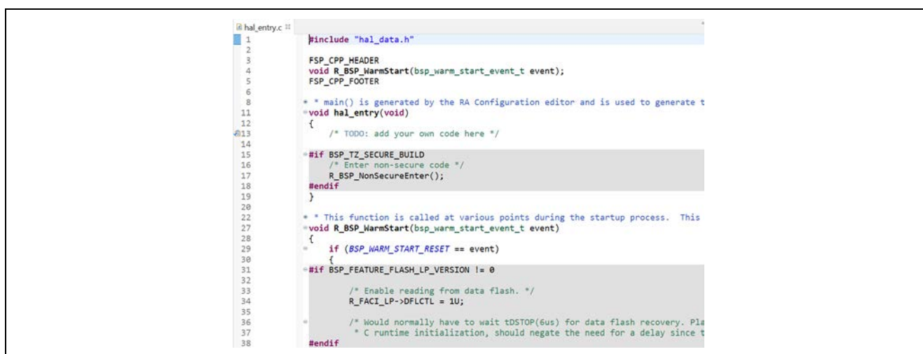
Figure 55. Old hal_entry.c
