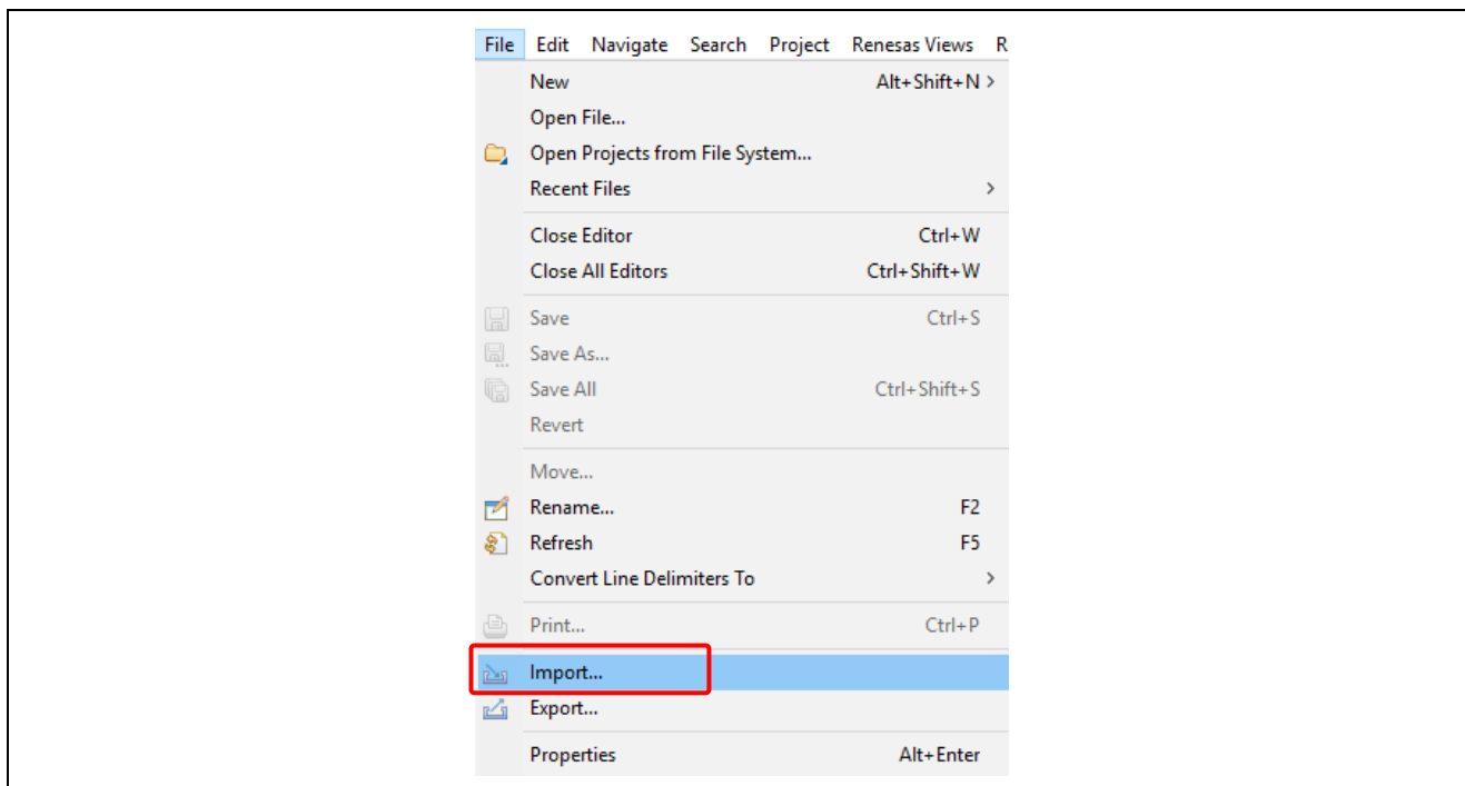
Figure 39. Import Project
