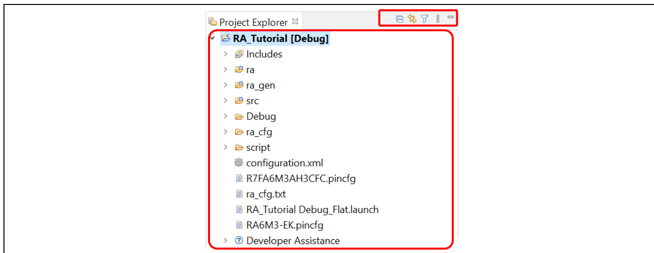
Figure 42. Imported Project
