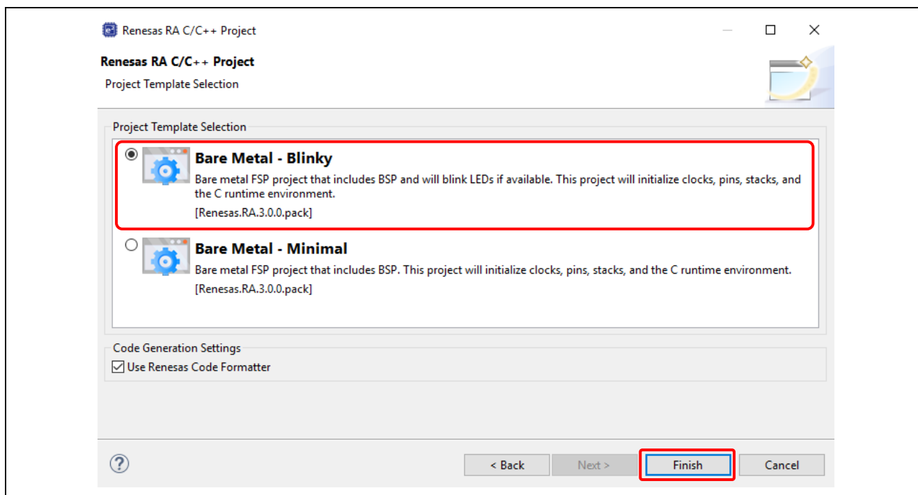
Figure 47. Select Project Template For Library
