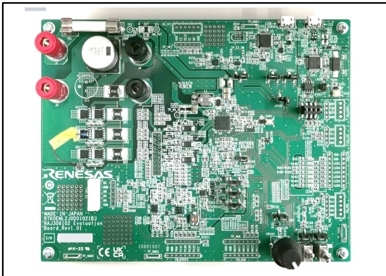
Figure 2-1 Appearance
