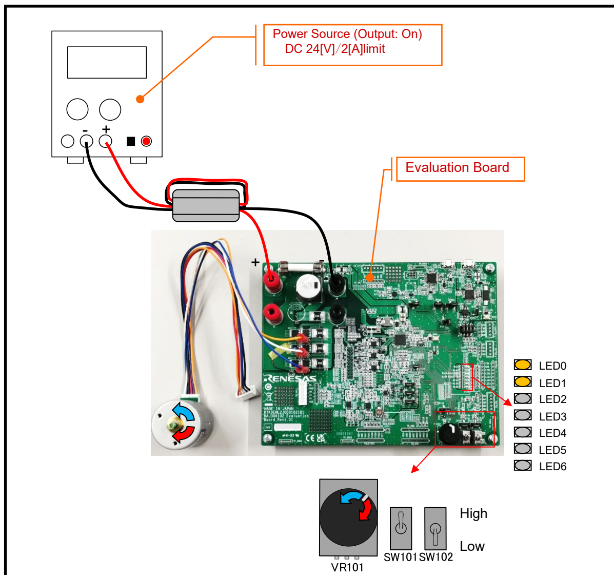
Figure 3-14 Motor Operation
