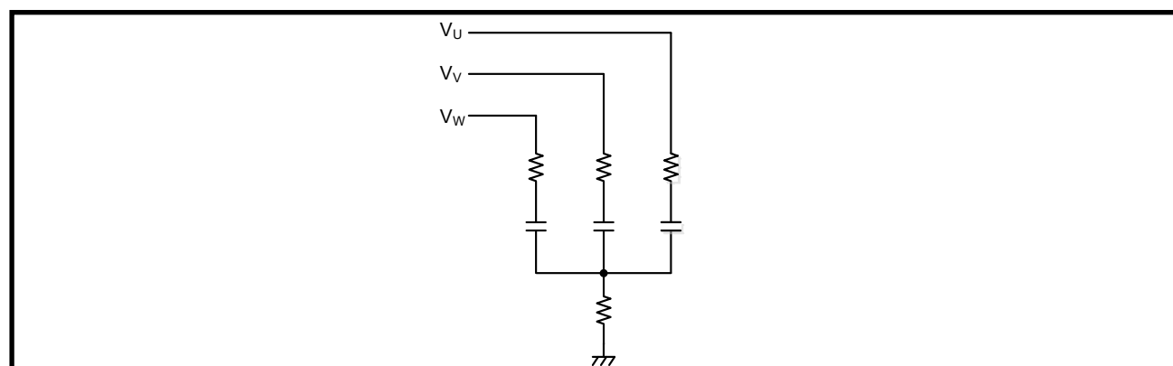
Figure 4-12 Spare Circuit
