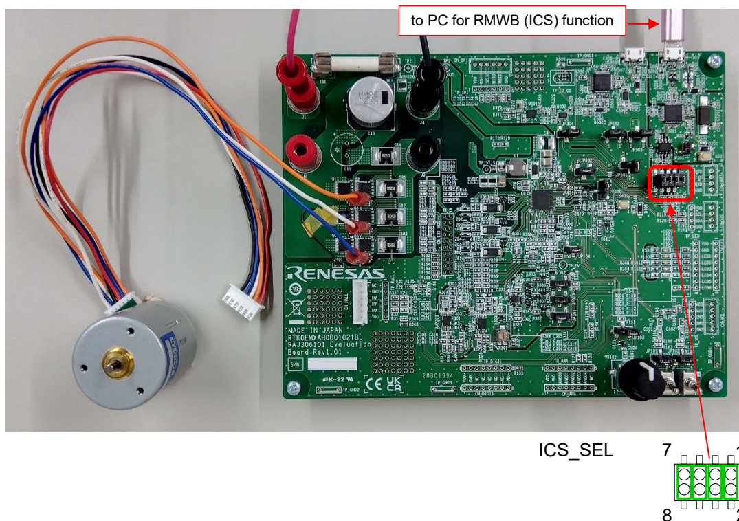
Figure 6-1 PC との接続 (RMWB (ICS) Function)
