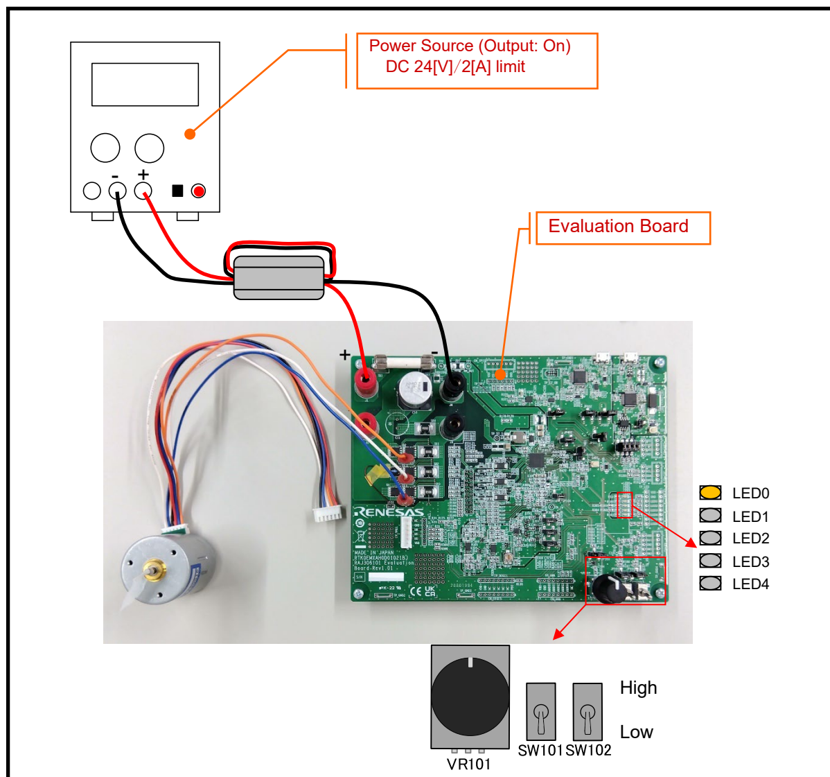
Figure 3-6 電源供給
