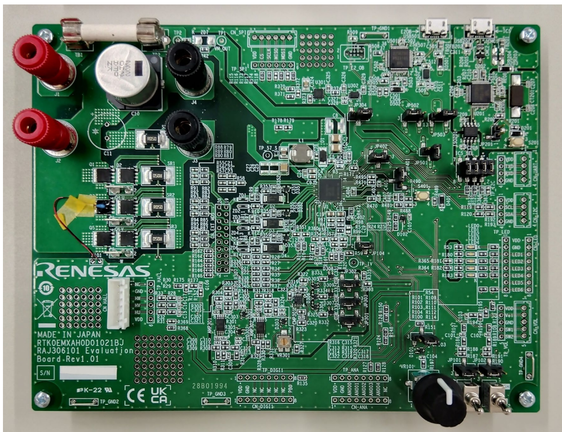
Figure 2-1 外観
