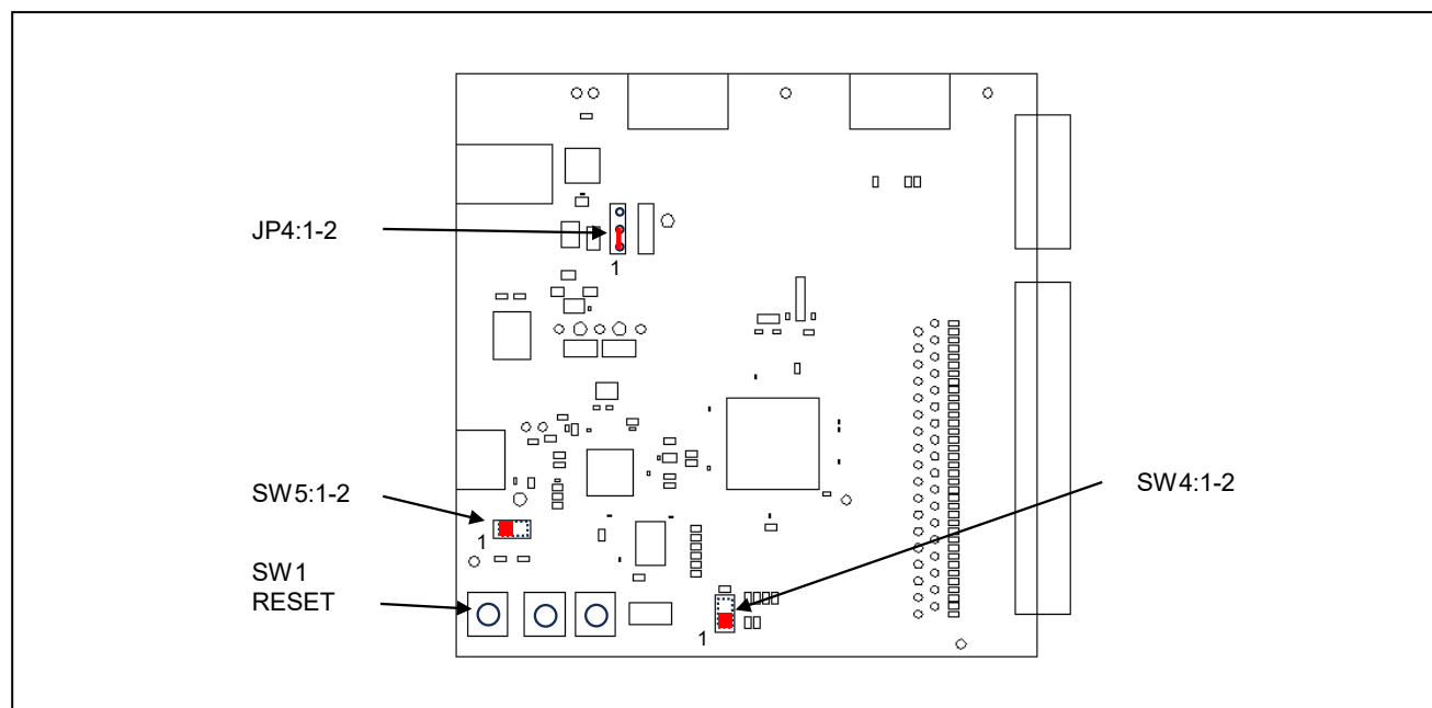
Figure 4 Switch Layout
