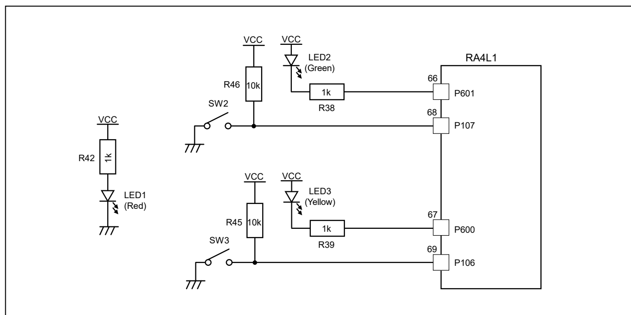
Figure 9 Push Switch and LED Circuits
