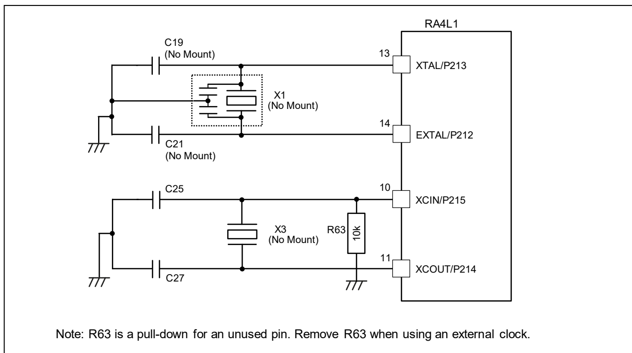
Figure 7 Clock Circuit
