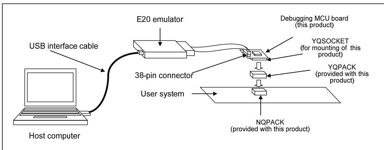
Figure 1 System Configuration
