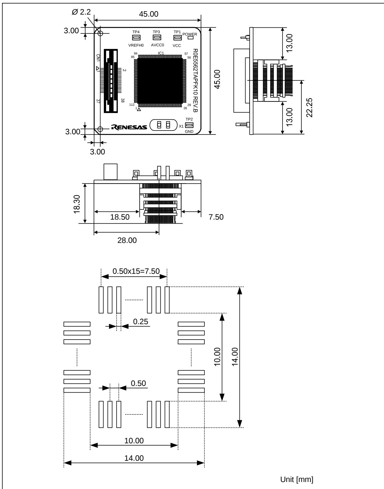
Figure 4 Reference Pad Pattern and Dimensions of the Debugging MCU Board (R0E5562TAPFK10)
