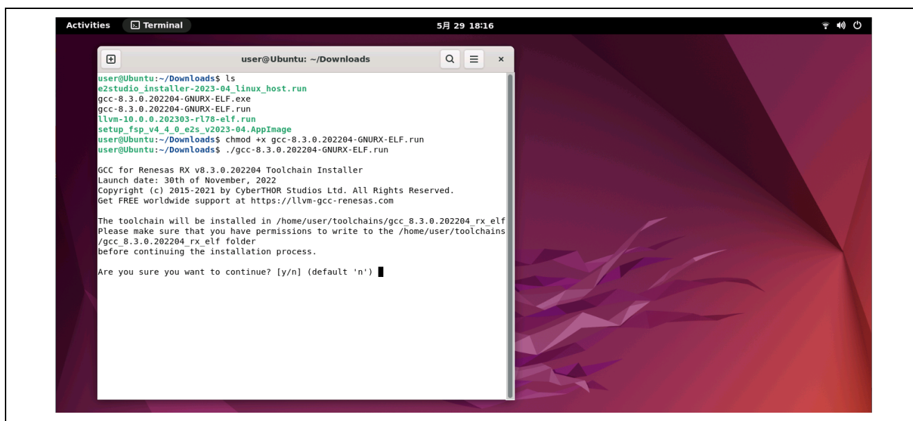
Figure 29 Running the Installer for GCC for Renesas RX
