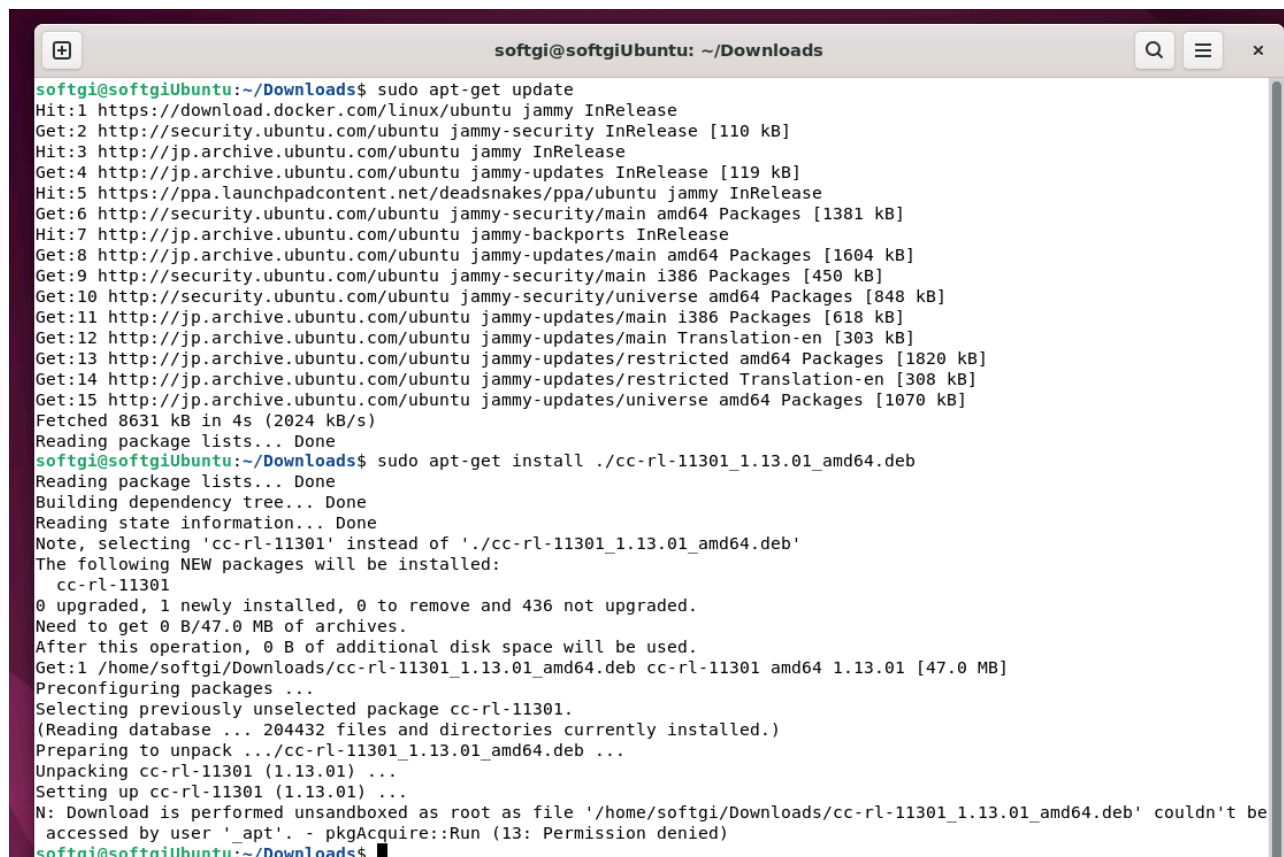
Figure 21 Installation example of the CC-RL
