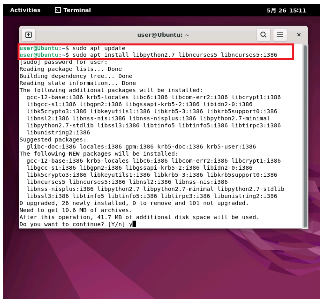
Figure 3 Installing the Required Libraries
