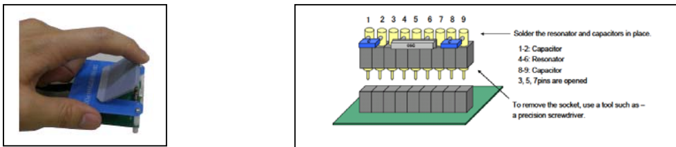
Figure 2-1 Clock setup
