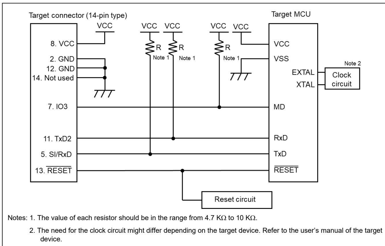
Figure 3.11 Example of a Circuit for an S7G2 (UART)
