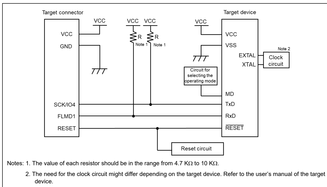
Figure 3.12 Example of a Circuit for R7F0E017D (UART)
