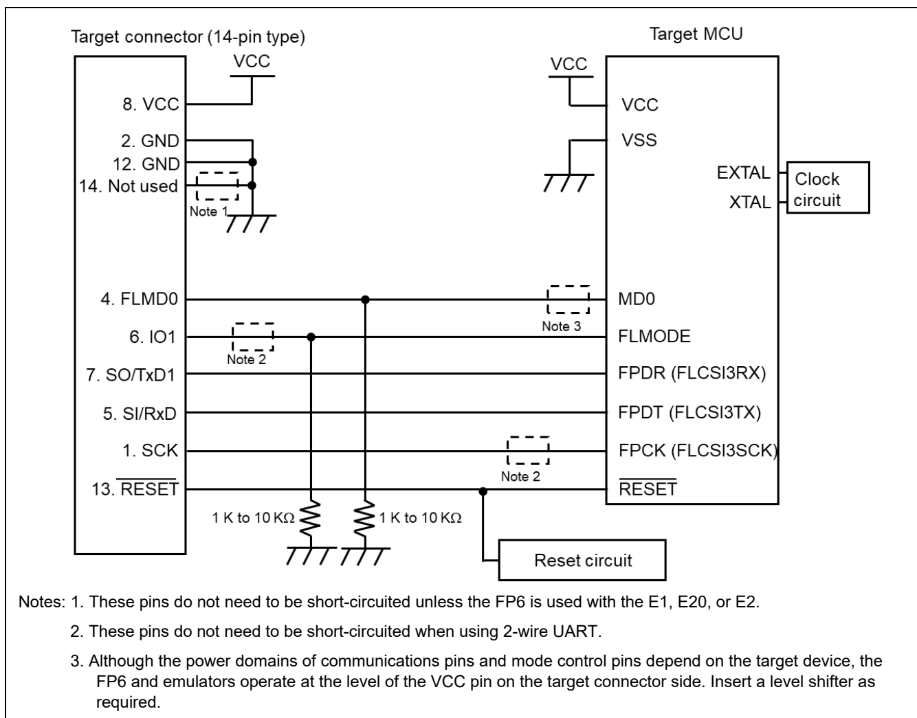
Figure 3.10 Example of a Circuit for RH850 Family (2-wire UART or CSI) (Case of RH850/E1x)
