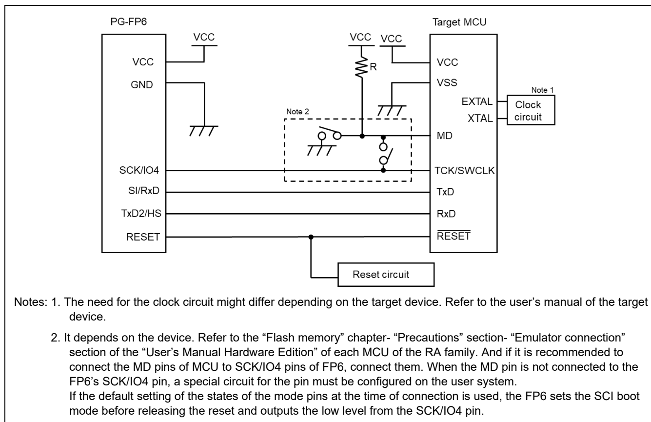
Figure 3.1 Example of a Circuit for RA6M3 (UART)
