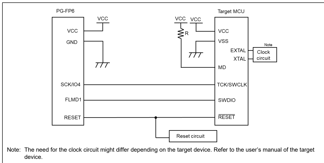
Figure 3.2 Example of a Circuit for RA6M3 (SWD)
