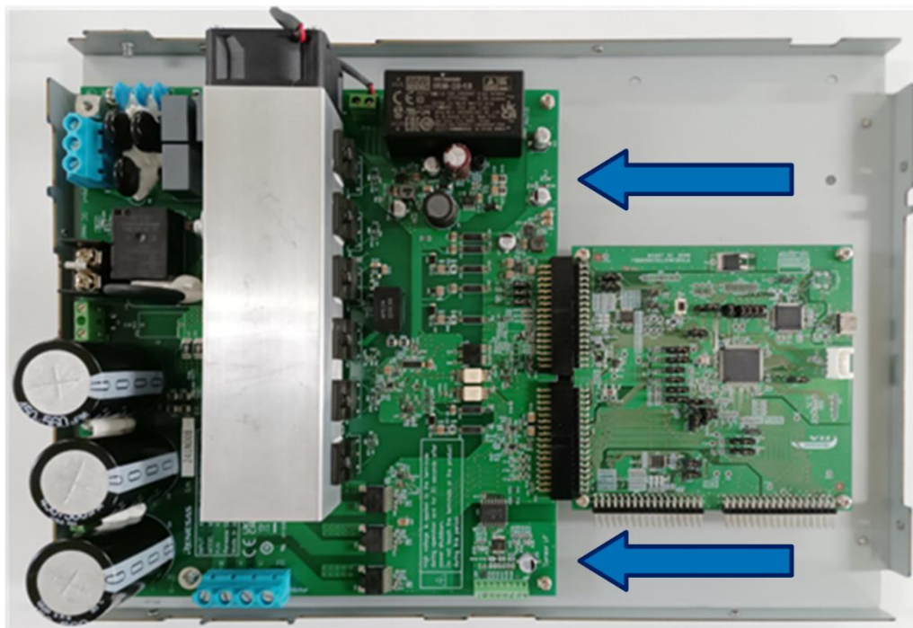
Fig. 3-3 Board Connection (Inverter board, CPU board)
