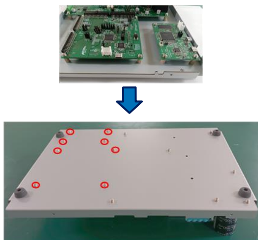
Fig. 3-4 Installation on the base plate (communication board, CPU board)
