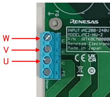
Fig. 3-6 Motor Connection
