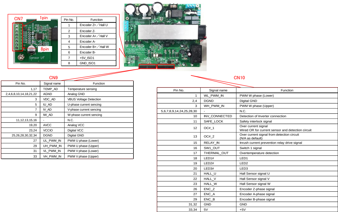
Fig. 2-4 Pin assignment of connector
