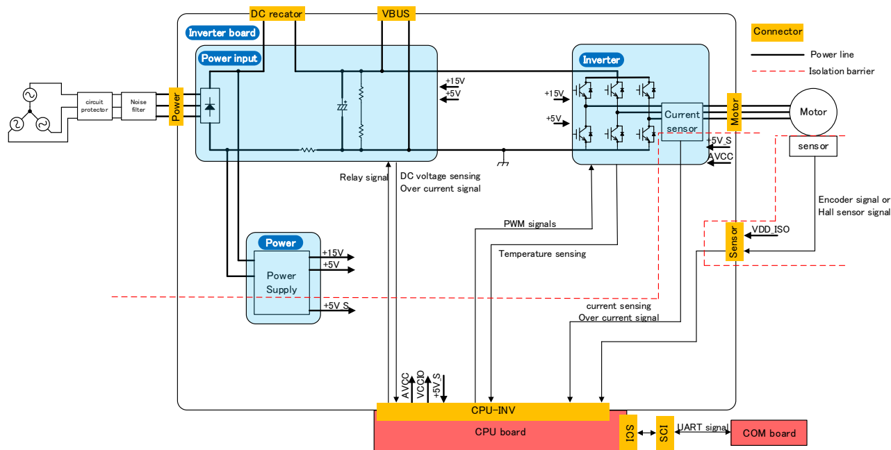
Fig. 2-1 MCI-HV-2-3PH function block diagram
