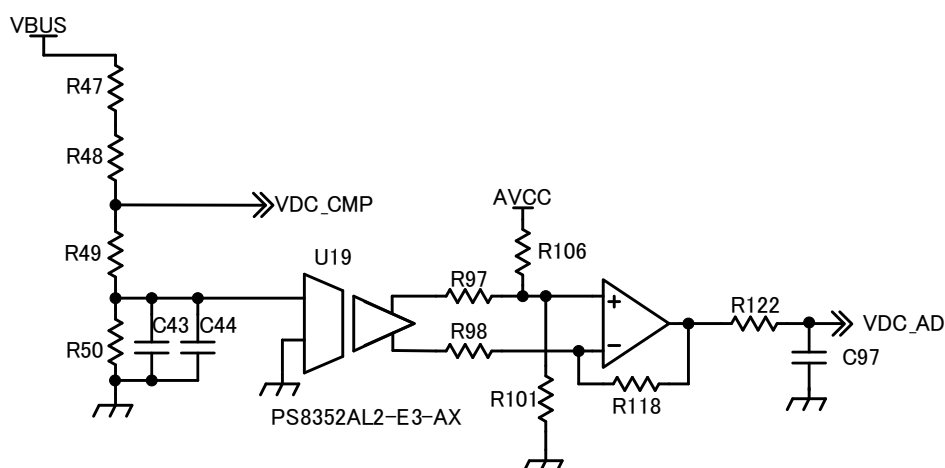
Fig. 4-1 Bus voltage sensing circuit
