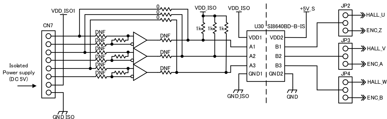
Fig. 4-6 Sensor I/F circuit
