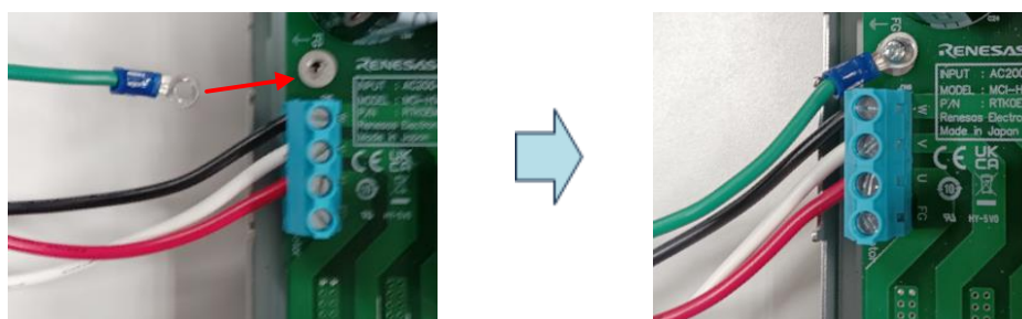
Fig. 3-7 Motor FG Connection
