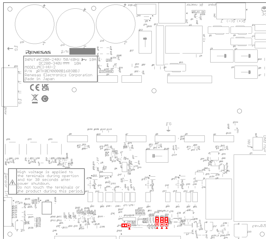
Fig. 2-3 Default jumper pin setting of inverter board
