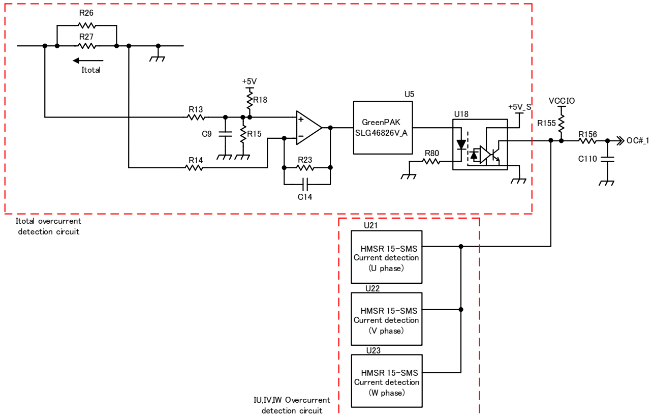
Fig. 4-5 Over current protection
