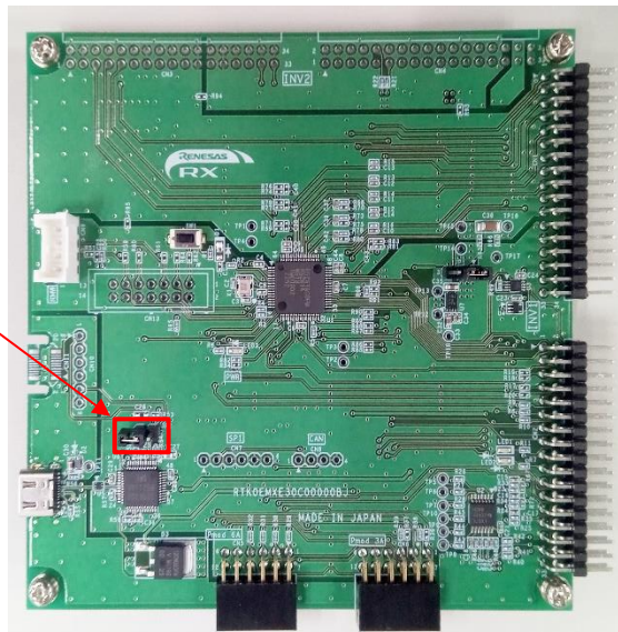
Figure 5-1 JP2 setting
