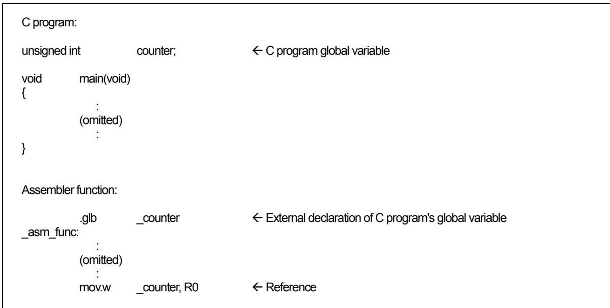
Figure 3.18 Referencing a C Global Variable
