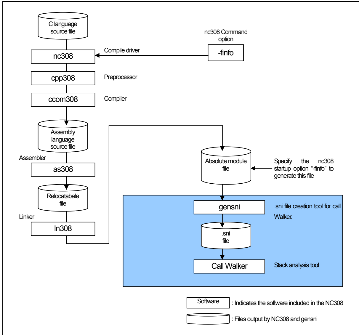
Figure G.1 Processing flow of NC308
