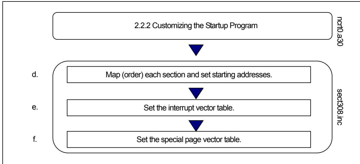
Figure 2.21 Example Sequence for Modifying Startup Programs
