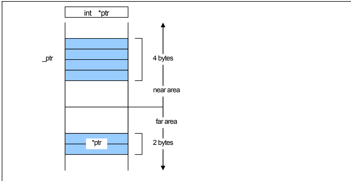
Figure B.6 Memory Location of Pointer type Variable
