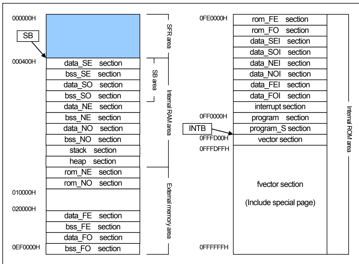
Figure 2.19 Example Section Mapping (1)
