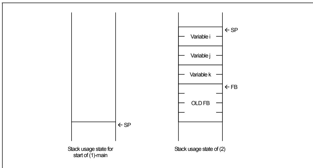
Figure D.17 Entry processing of function main
