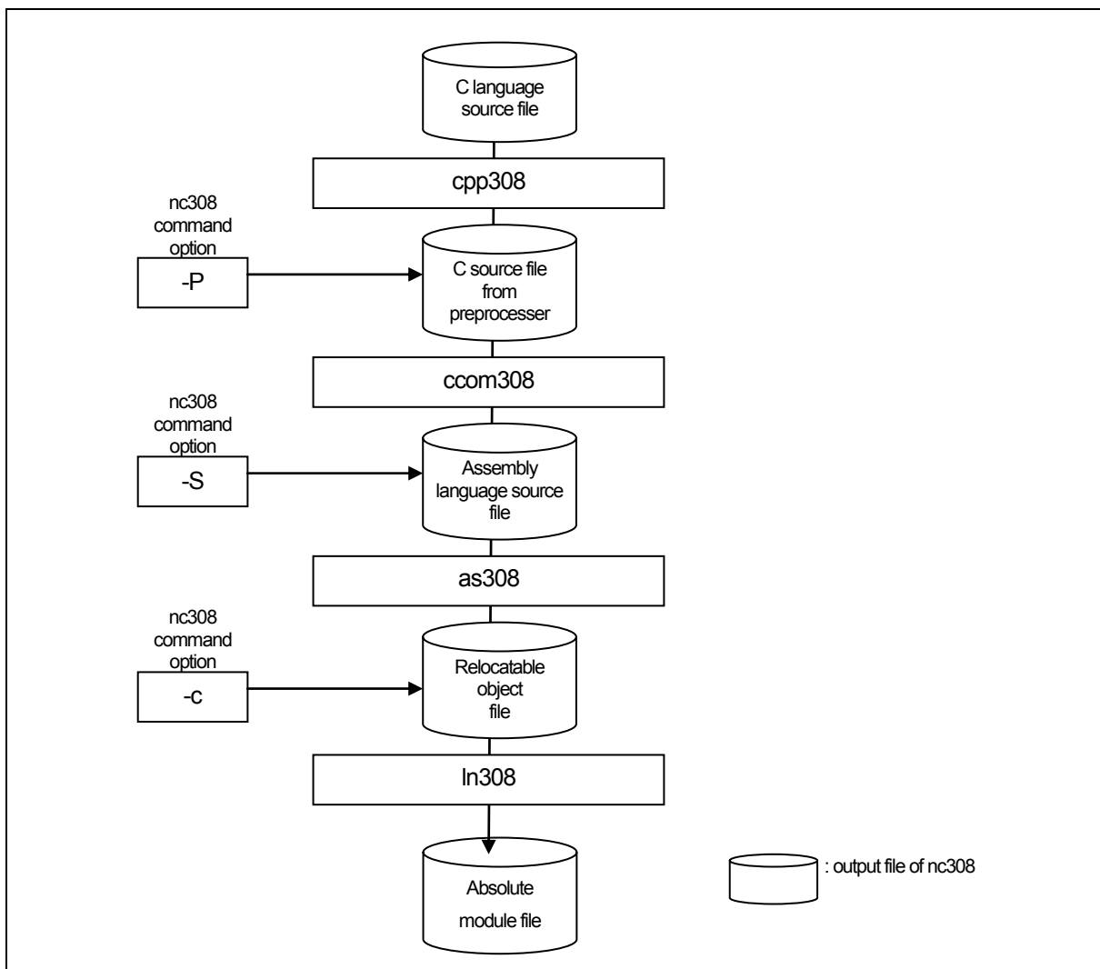
Figure 1.6 Relationship of nc308 Command Line Options and Output Files
