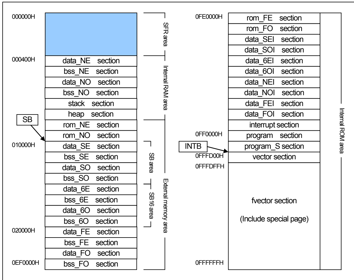
Figure 2.20 Example Section Mapping (2)
