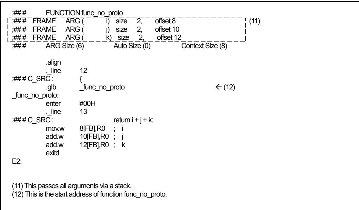
Figure D.12 Compile Result of Sample Program (sample.c) (2)
