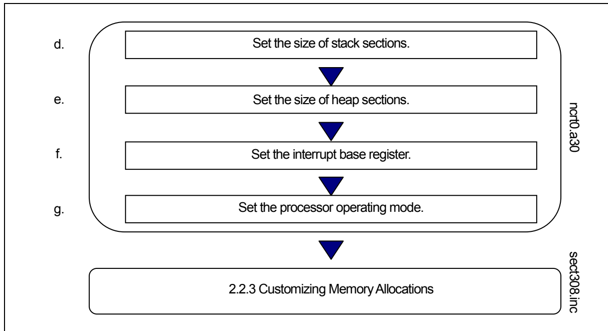
Figure 2.12 Example Sequence for Modifying Startup Programs
