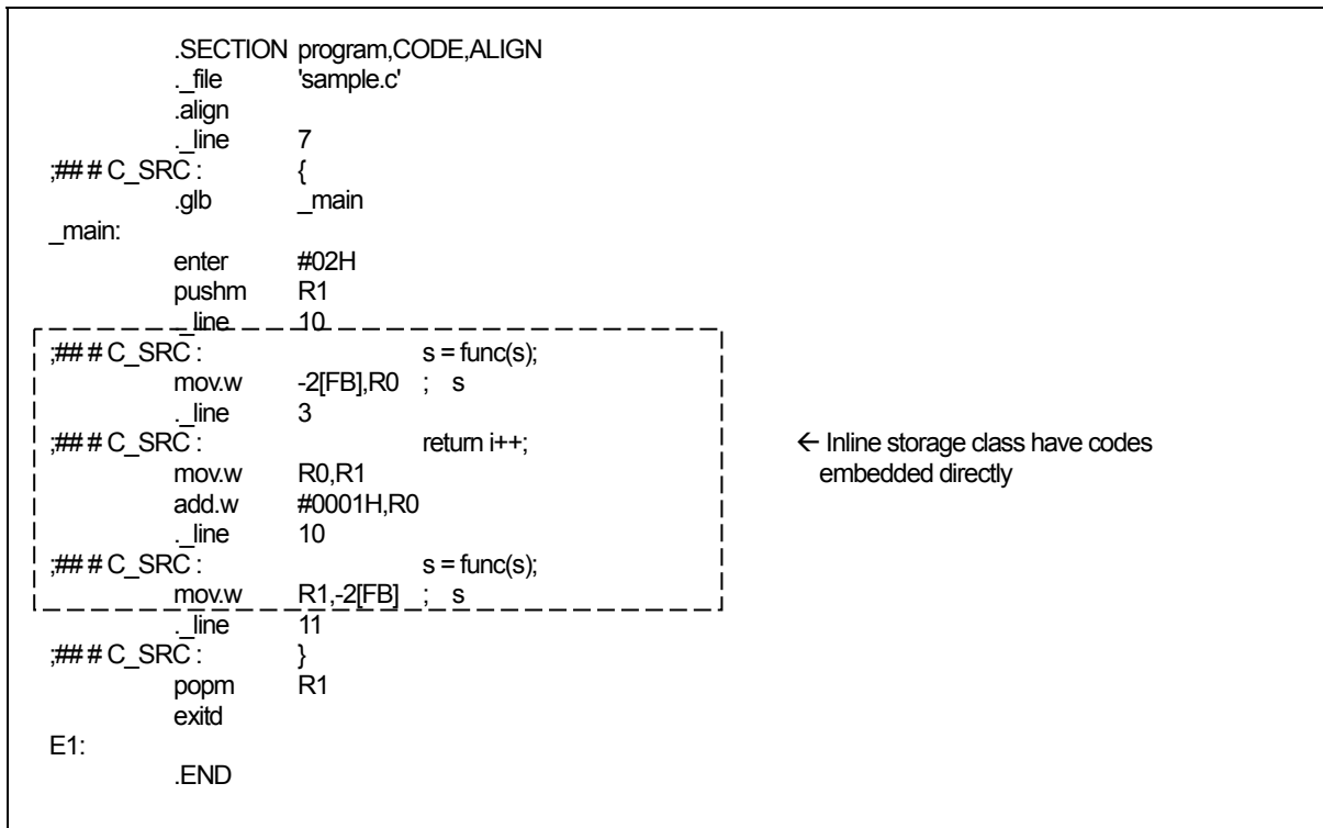
Figure B.55 Compile Result of sample program (smp.a30)
