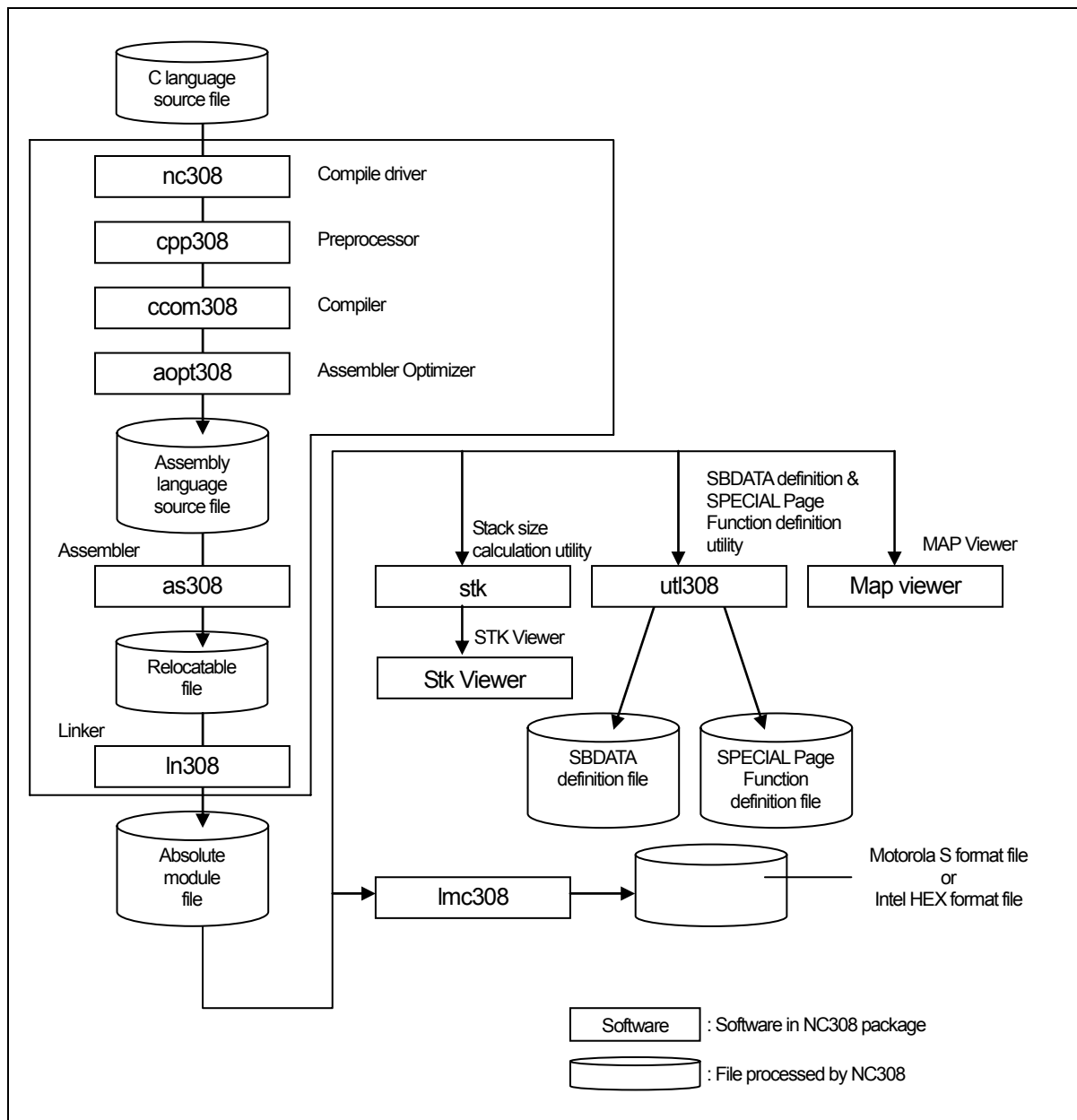
Figure 1.1 NC308 Processing Flow
