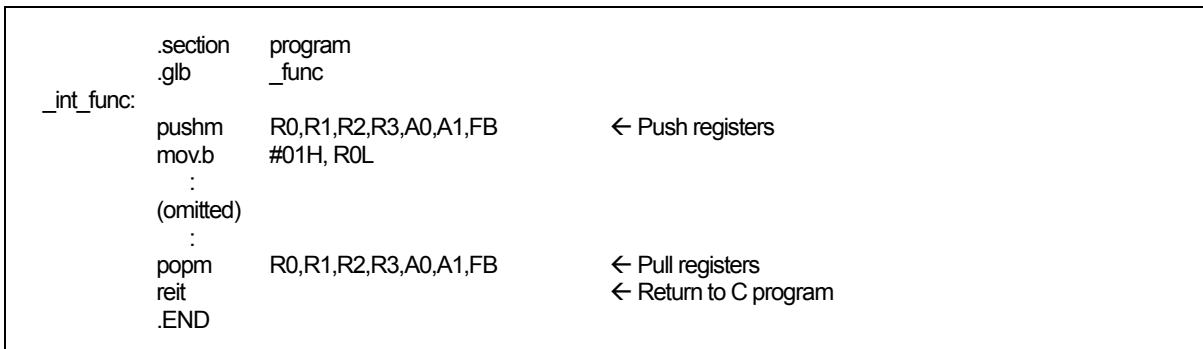
Figure 3.19 Example Coding of Interrupt Processing Assembler Function
