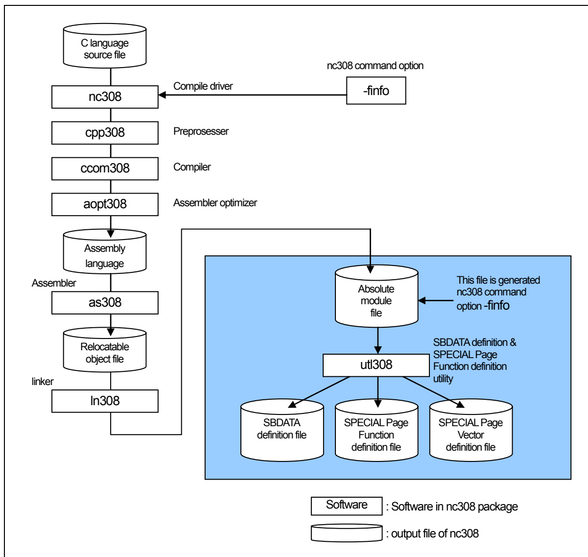
Figure G.1 NC308 Processing Flow
