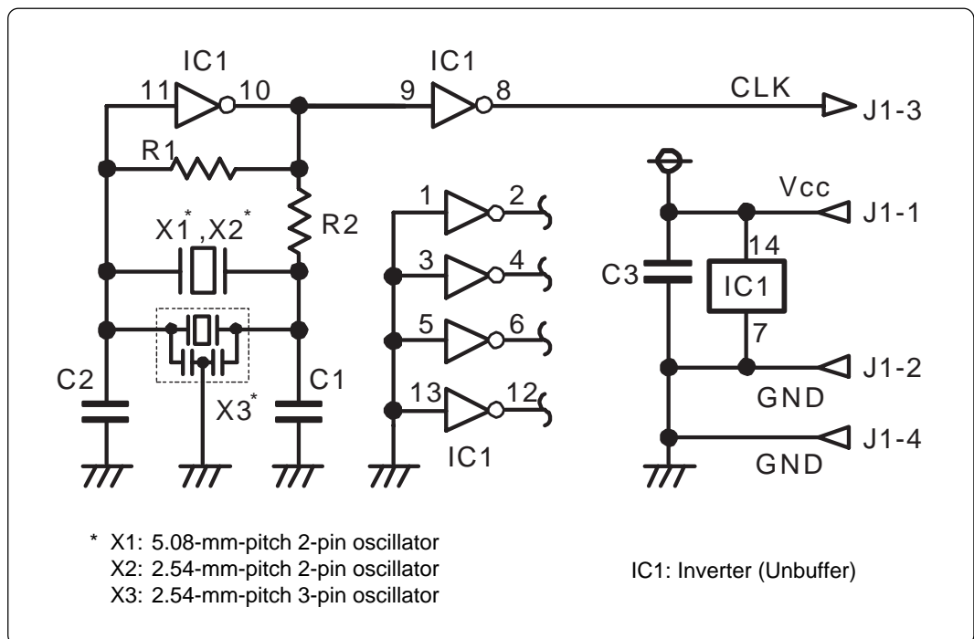
Figure 3.4 Circuit of the oscillator circuit board (OSC-2)
