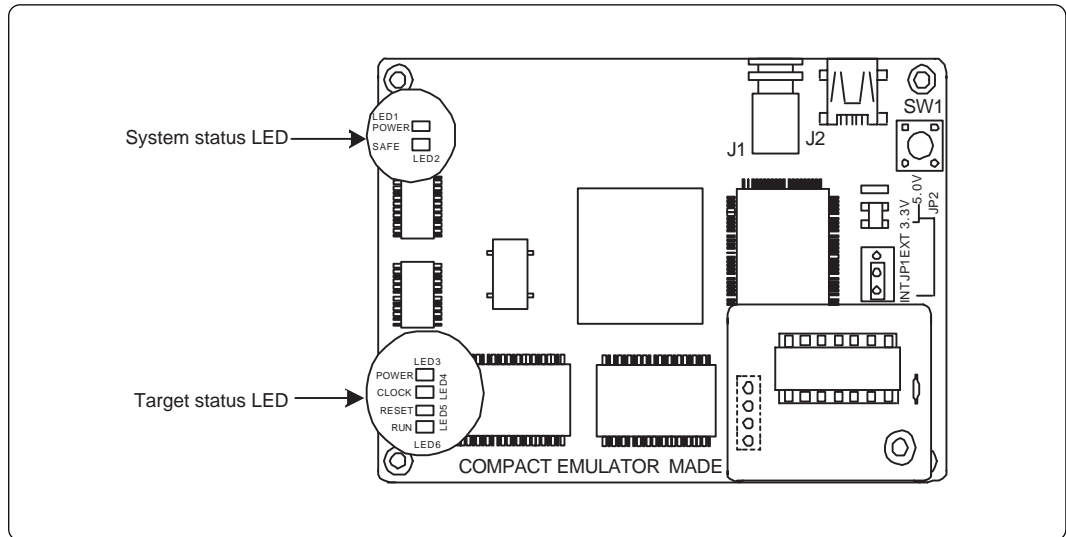
Figure 2.10 Positions of system status LEDs and target status LEDs
