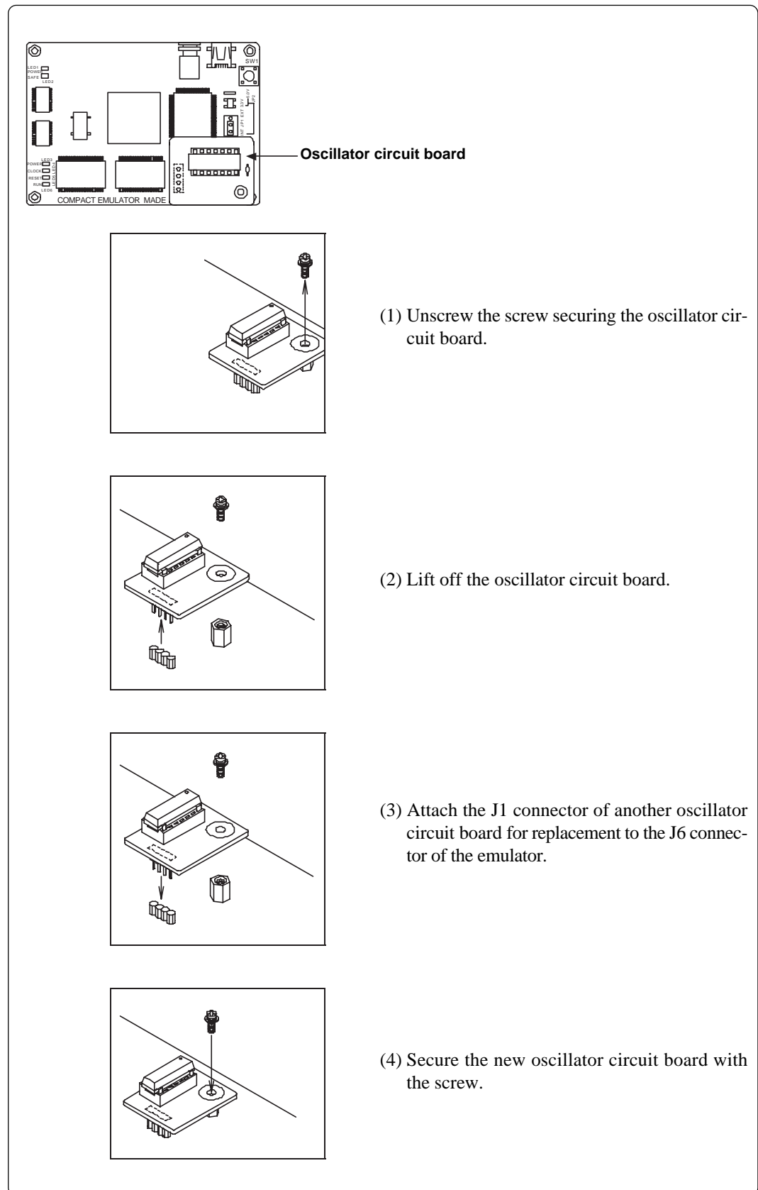
Figure 3.5 Replacing oscillator circuit boards
