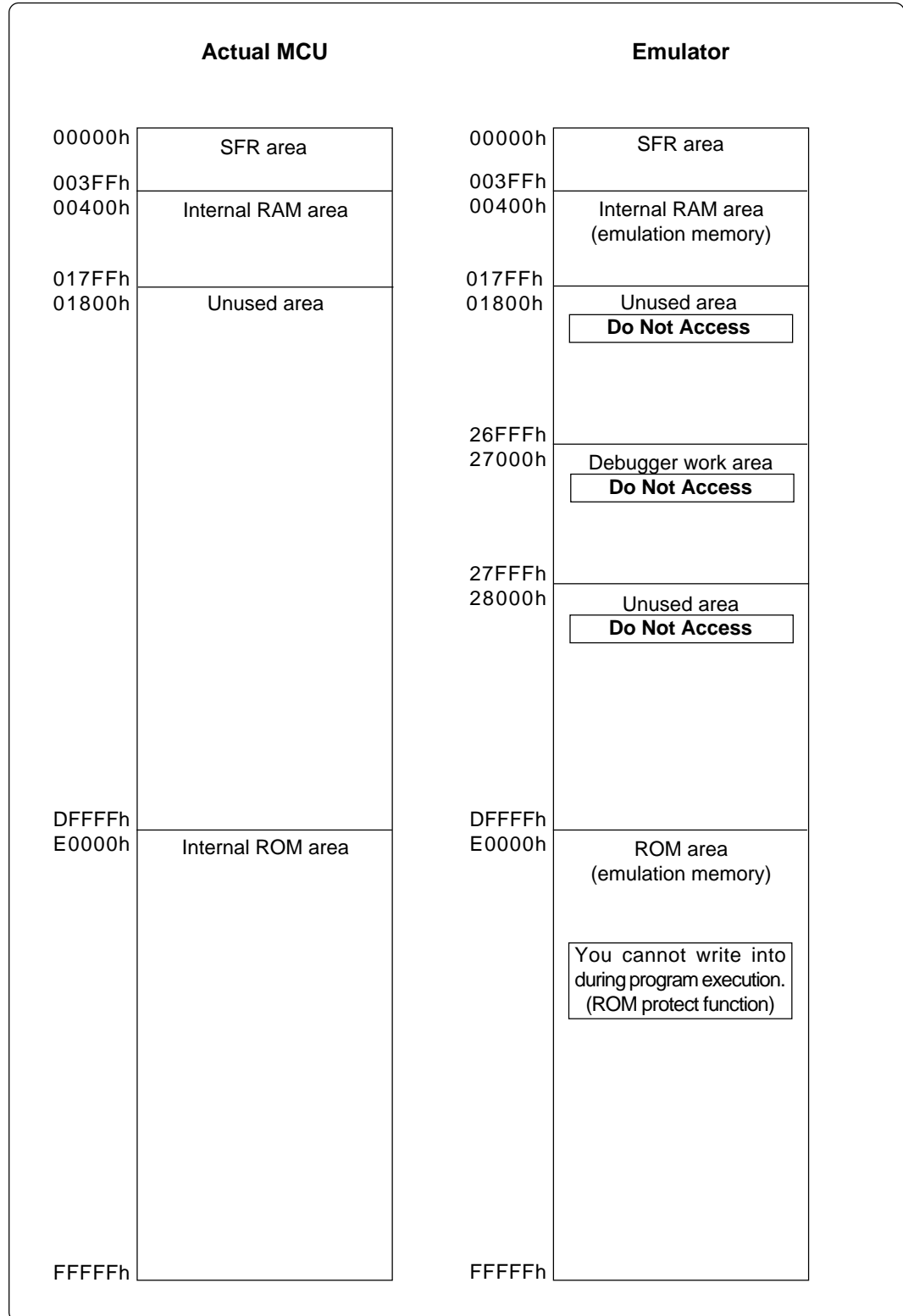
Figure 4.1 Memory map when using the emulator
