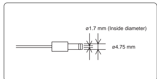
Figure 2.7 Specification of an applicable plug
