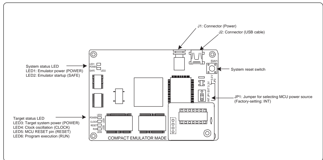
Figure 2.2 Name of each part of the emulator (upper side of the M306K9T2-CPE)
