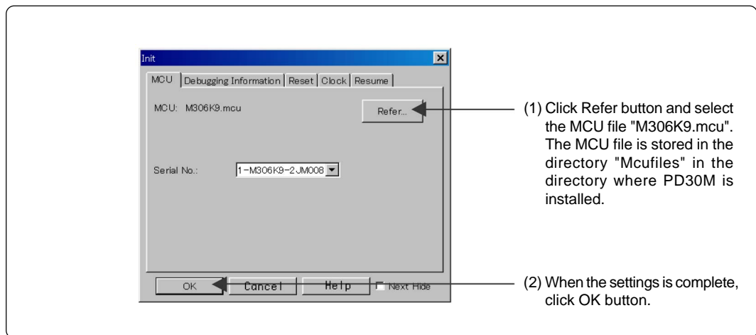
Figure 2.13 Setting the Init dialog box
