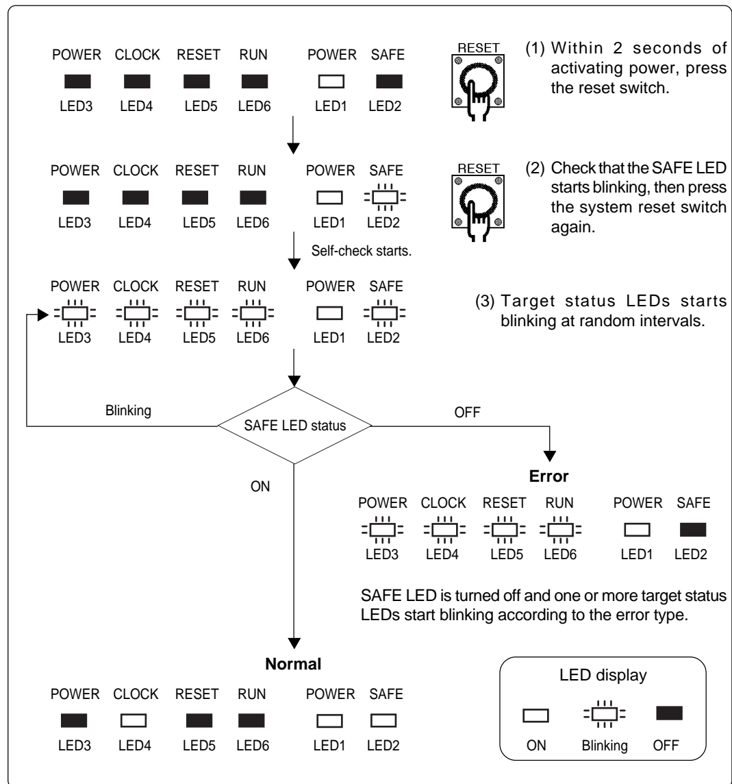
Figure 5.2 Self-check procedure
