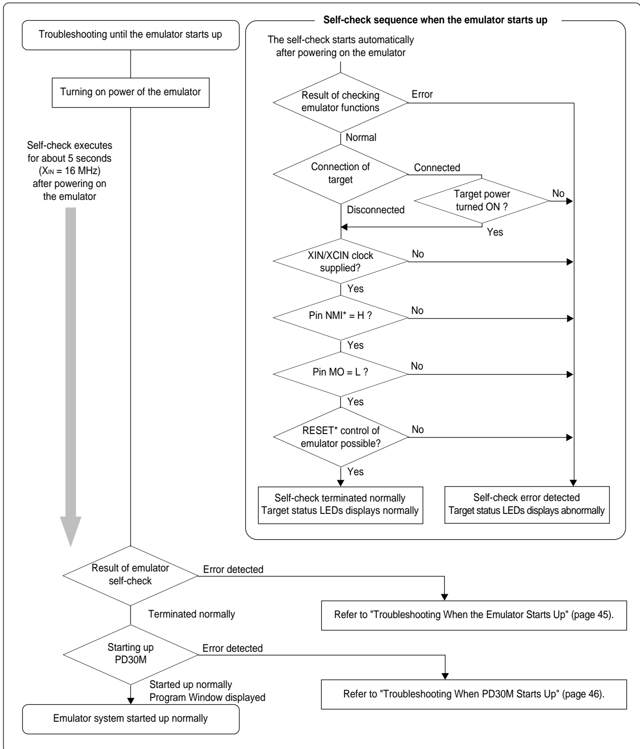
Figure 5.1 Flowchart to remedy the troubles
