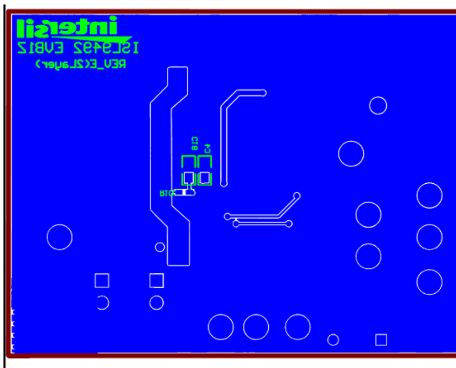
FIGURE 14. 2 LAYER - BOTTOM
