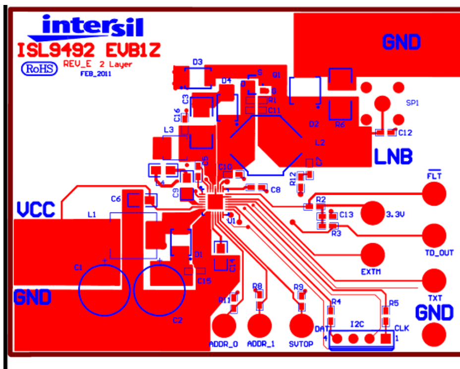
FIGURE 13. 2 LAYER - TOP
