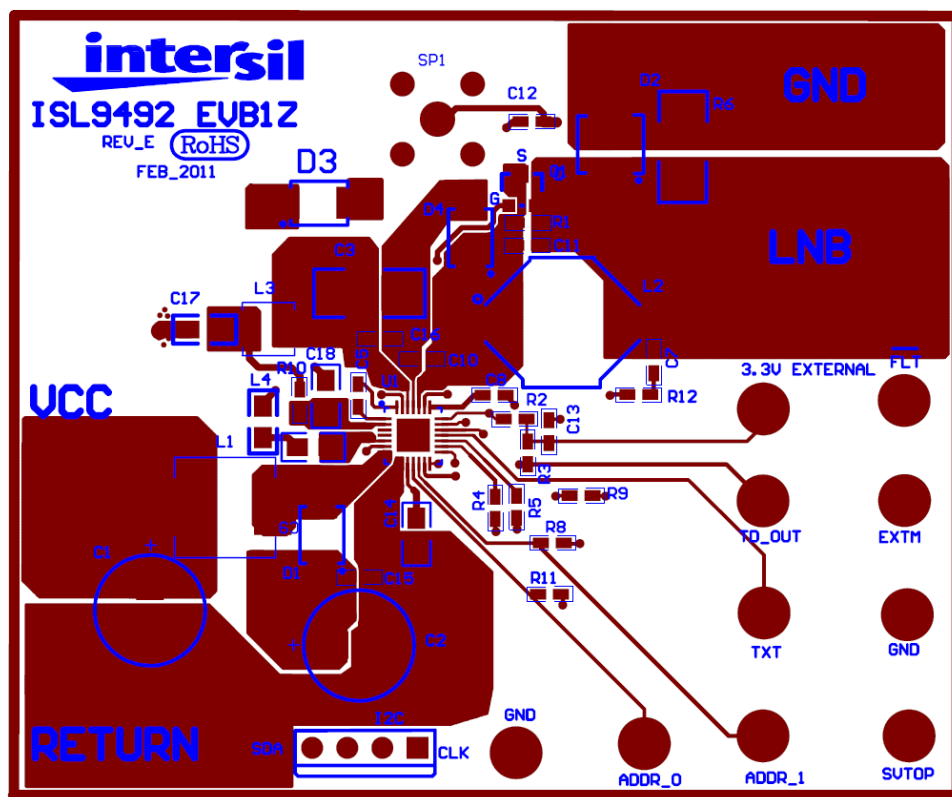
FIGURE 9. 4 LAYER - TOP
