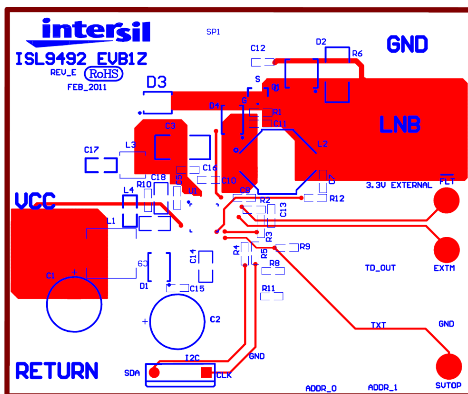
FIGURE 12. LAYER 4
