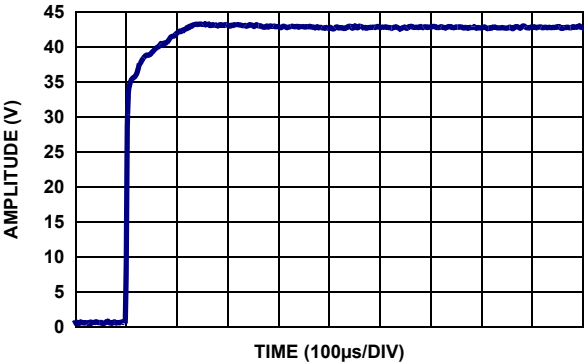
FIGURE 58. DFET RISE
