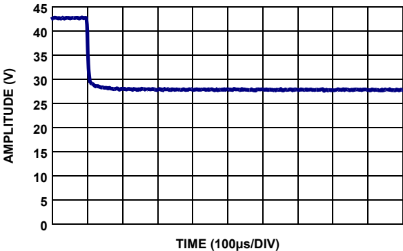
FIGURE 61. CFET FALL
