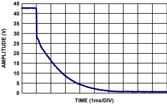
FIGURE 59. DFET FALL
