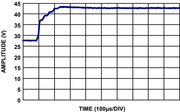
FIGURE 60. CFET RISE
