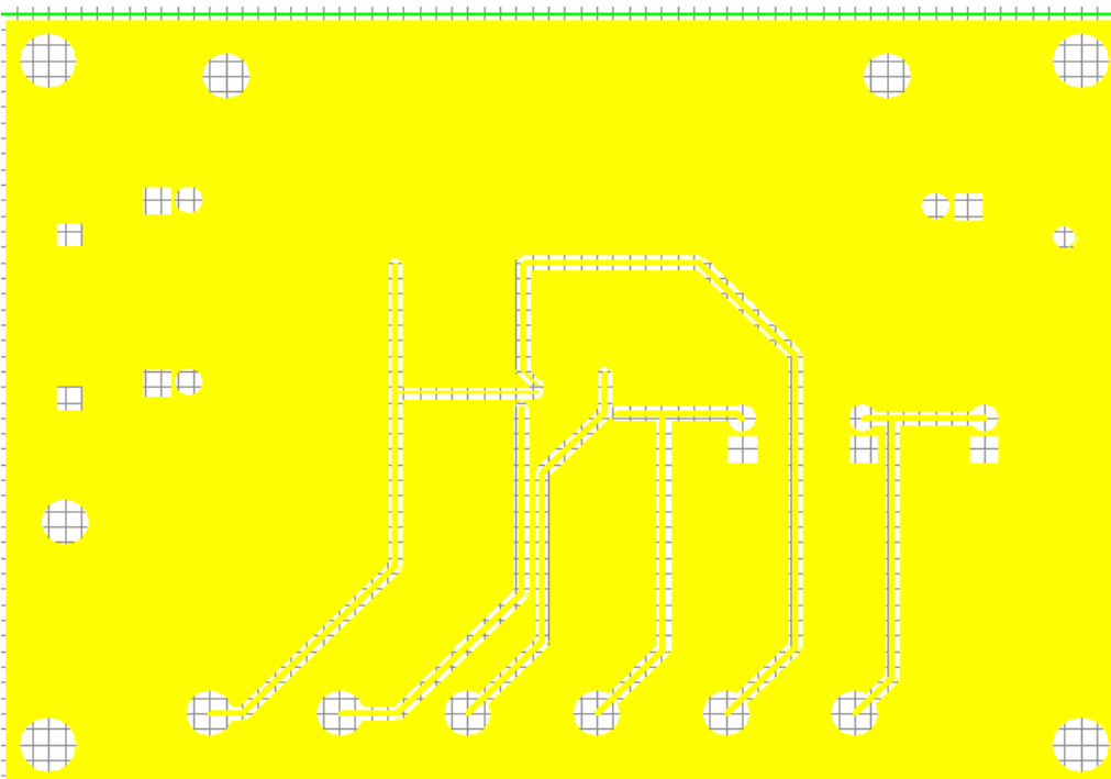
FIGURE 5. BOTTOM LAYER
