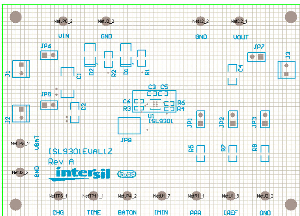
FIGURE 3. SILK LAYER
