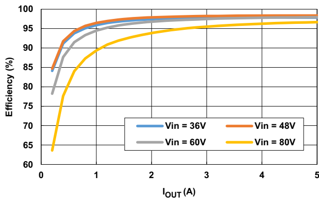
Figure 14. Efficiency, CCM
