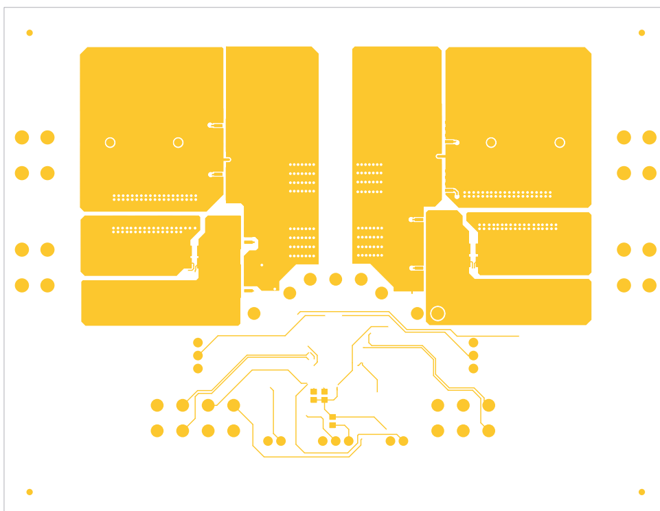
Figure 12. Bottom Layer
