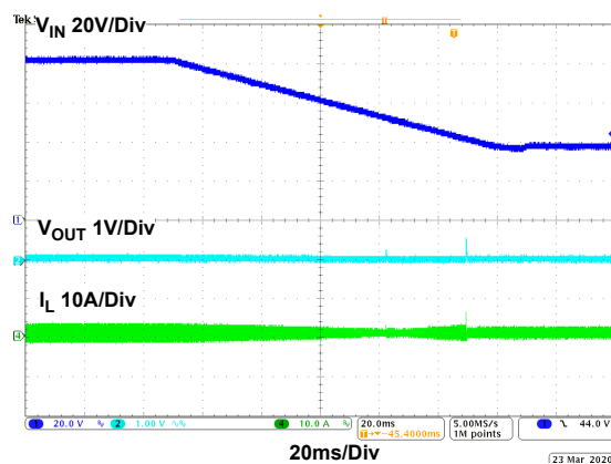
Figure 30. Line Transient, V_{IN} = 80V to 36V , 1V/ms , I_{OUT} = 0A
