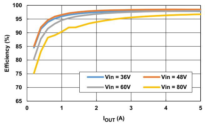
Figure 15. Efficiency, DEM
