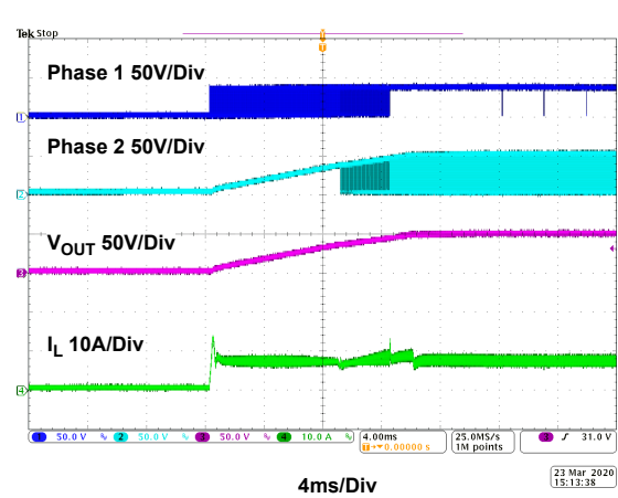
Figure 25. Start-Up Waveform, V_{IN} = 48V , I_{OUT} = 5A , CCM
