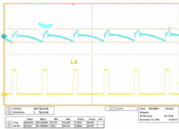
FIGURE 7. STEADY STATE: 1A LOAD (FCCM)
