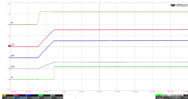
Figure 9. Startup: Fast Start Enabled, 1A Load
