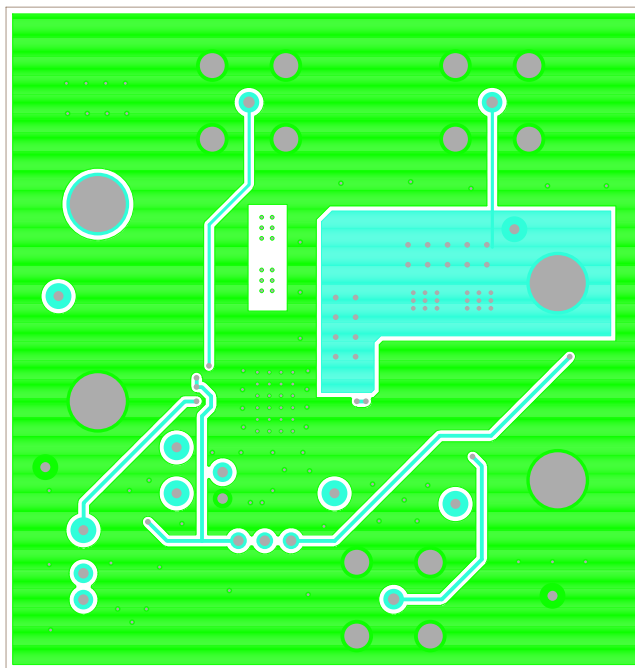
Figure 7. Layer 3
