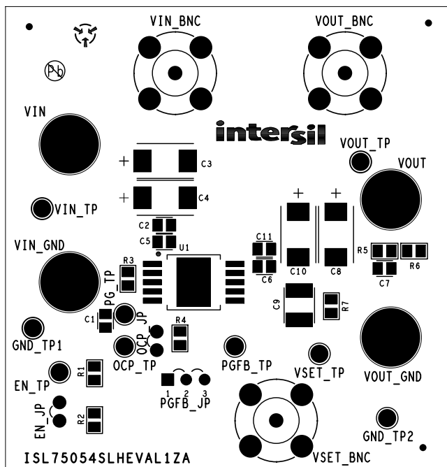
Figure 4. Silkscreen Top
