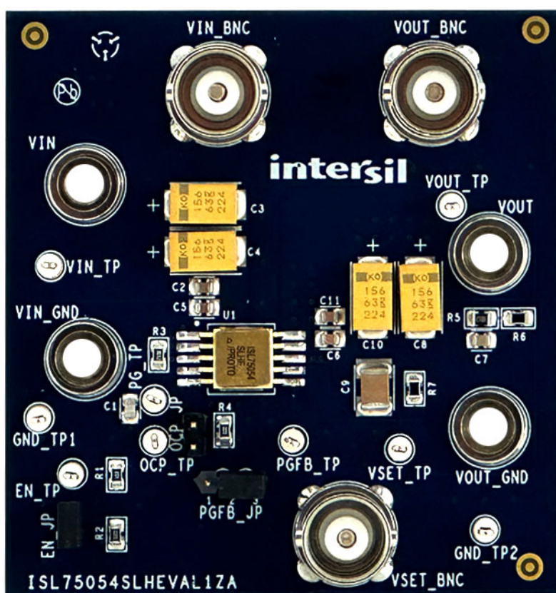
Figure 2. ISL75054SLHEVAL1Z Evaluation Board (Top)
