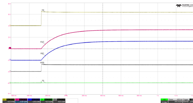
Figure 10. Startup: Fast Start Disabled, 1A Load
