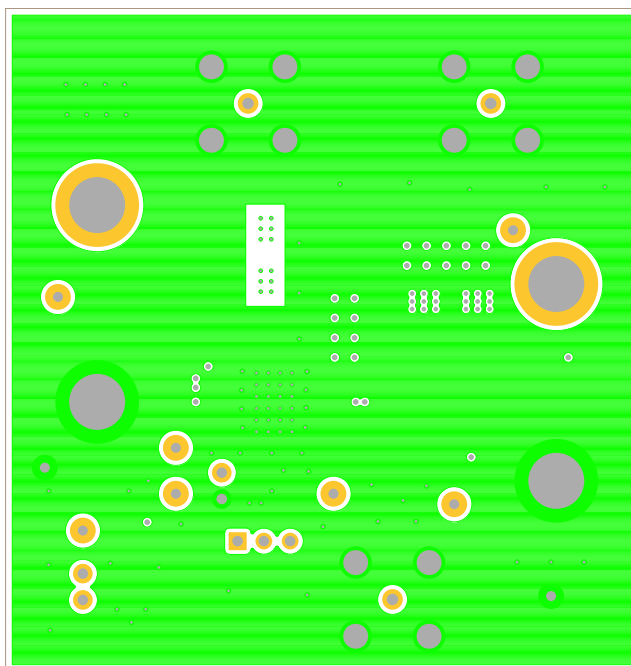
Figure 8. Bottom Layer
