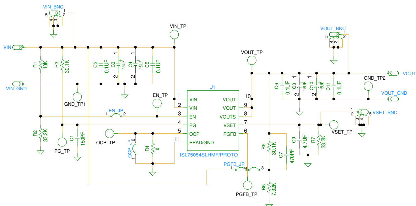
Figure 3. ISL75054SLHEVAL1Z Schematic
