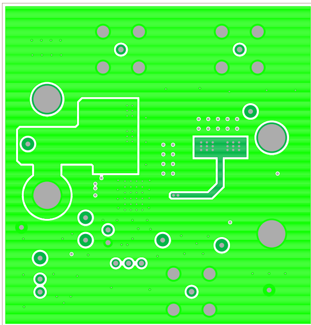
Figure 6. Layer 2
