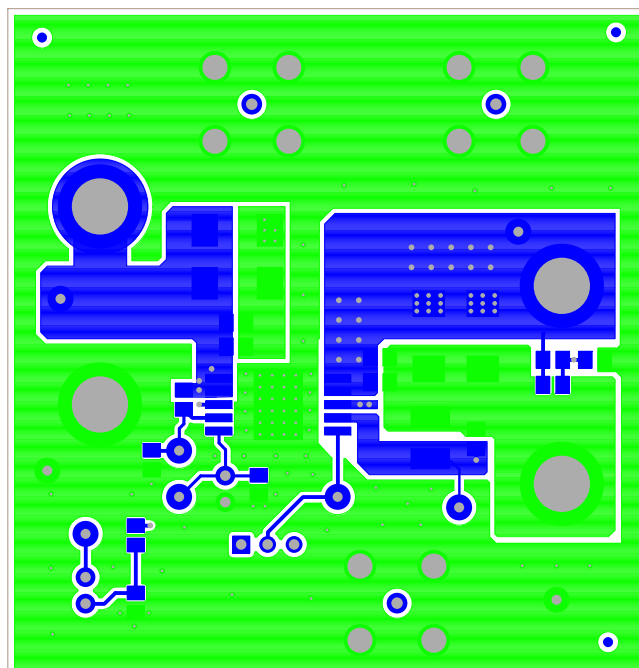
Figure 5. Top Layer
