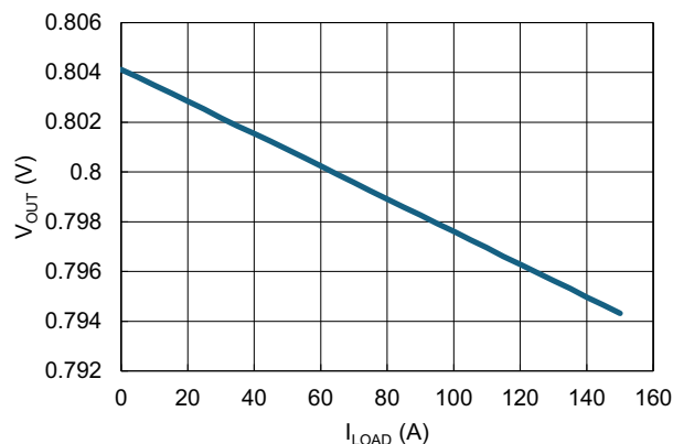
Figure 93. DROOP Regulation (VDD = 12V, PVIN = 12V)
