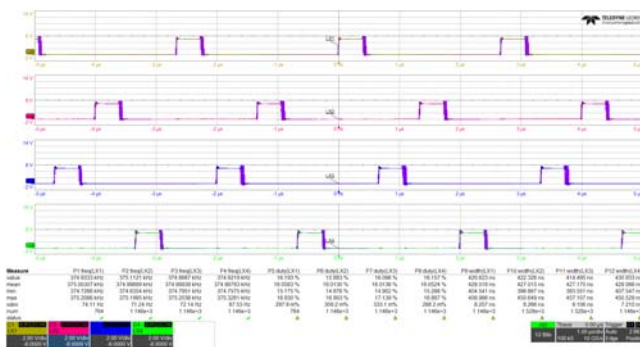
Figure 60. Phase Node Steady-State Jitter ( V_{DD} = 5V , P_{VIN} = 5V , I_{LOAD} = 0A )
