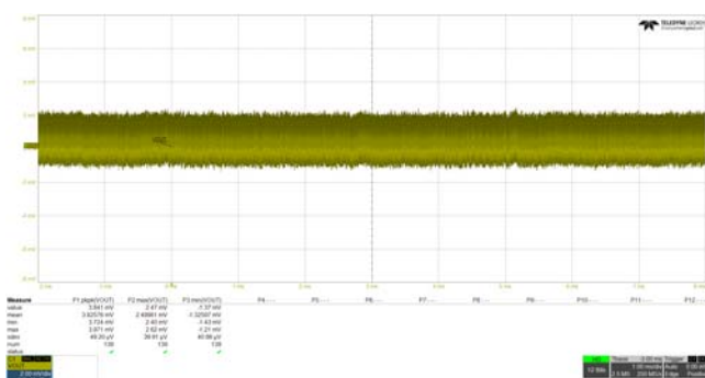
Figure 78. VOUT Ripple measured at TP76 PH2 Output (VDD = 12V, PVIN = 12V, I_{LOAD} = 0A , VOUT_COMMAND = 0.6V, 20MHz BW filter, AC-Coupled)
