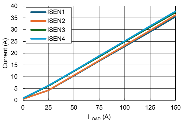
Figure 90. ISEN Telemetry (VDD = 5V, PVIN = 5V, 50 Averages)
