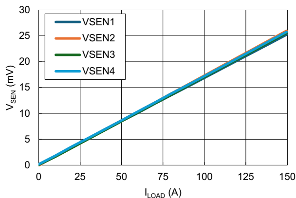
Figure 68. ISEN1-4 Current Sharing (VDD = 5V, PVIN = 5V, I_{LOAD} = 0A )
