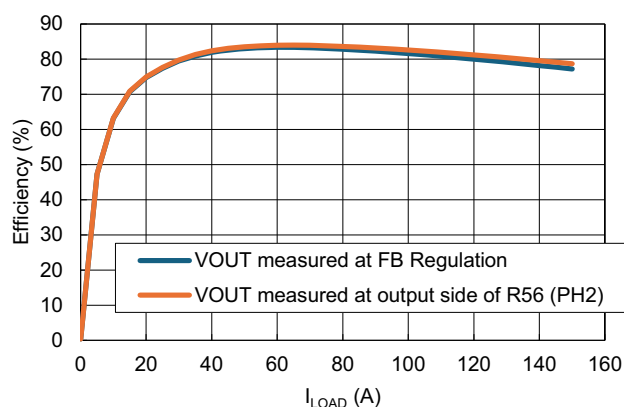
Figure 95. Efficiency (VDD = 12V, PVIN = 12V)
