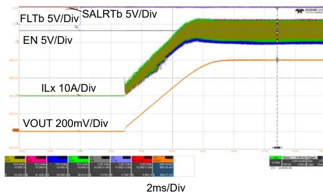
Figure 41. Soft-Start with the FLTb pin ( V_{DD} = 12V , P_{VIN} = 12V , I_{LOAD} = 150A , V_{OUT\_COMMAND} = 0.6V )
