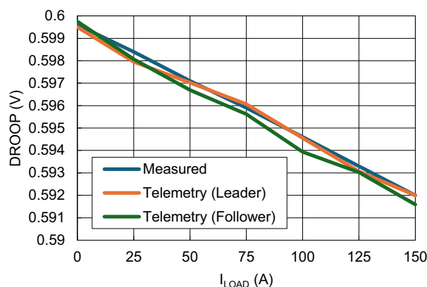
Figure 85. DROOP Telemetry ( V_{DD} = 12V , PVIN = 12V , I_{LOAD} = 0A , 50 Averages)
