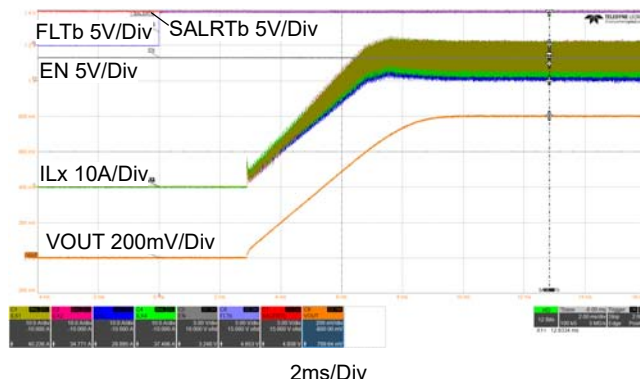
Figure 39. Soft-Start with the FLTb pin ( V_{DD} = 5V , P_{VIN} = 5V , I_{LOAD} = 150A , V_{OUT\_COMMAND} = 0.6V )
