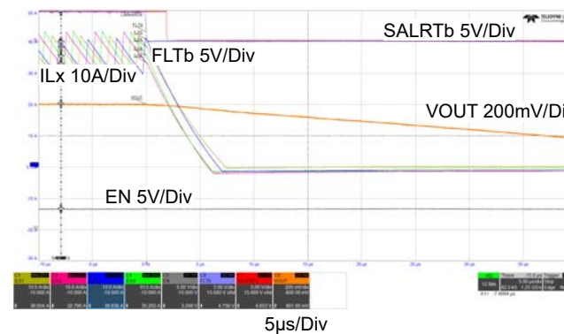
Figure 53. Shutdown with the FLTb Pin (VDD = 12V, PVIN = 12V, I_{LOAD} = 150A )
