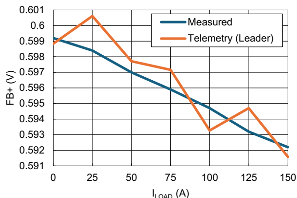
Figure 87. FB+ Telemetry (VDD = 12V, PVIN = 12V, I_{LOAD} = 0A , 50 Averages)
