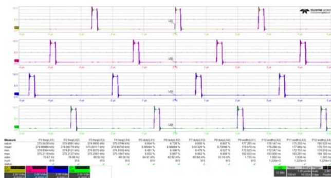
Figure 62. Phase Node Steady State Jitter (VDD = 12V, PVIN = 12V, I_LOAD = 0A)
