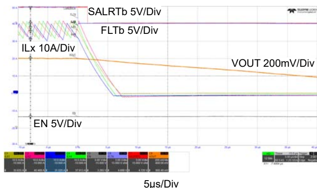
Figure 50. Shutdown with the FLTb Pin (VDD = 5V, PVIN = 5V, I_{LOAD} = 0A )
