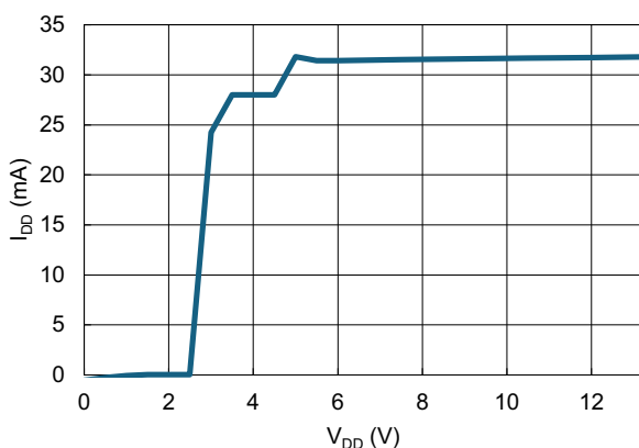
Figure 96. VDD Shutdown Current (EN = Low, OUTEN = Low)
