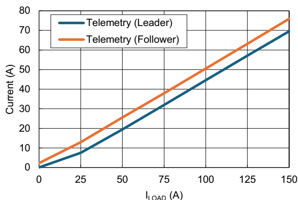
Figure 88. IOOUT Telemetry (VDD = 5V, PVIN = 5V, 50 Averages)
