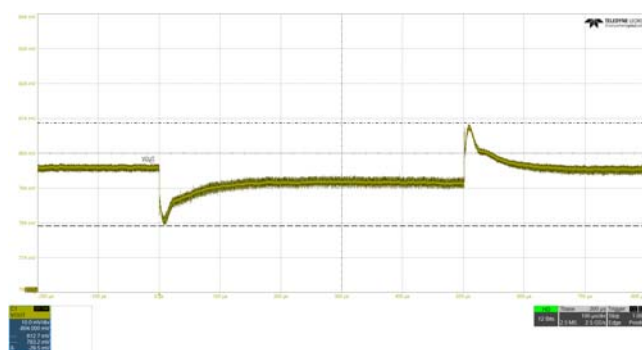
Figure 73. Load Transient Response (VDD = 5V, PVIN = 5V, I_{LOAD} = 75A \rightarrow 150A \rightarrow 75A , Slew = 200A/\mu s )
