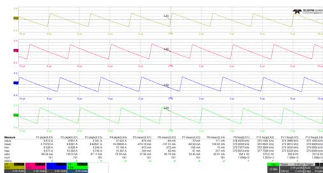
Figure 66. 4-Phase Inductor Current (VDD = 12V, PVIN = 12V, I_LOAD = 0A)
