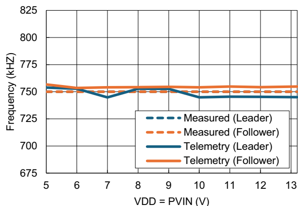
Figure 81. FOSC Telemetry ( I_{LOAD} = 0A , 50 Averages)
