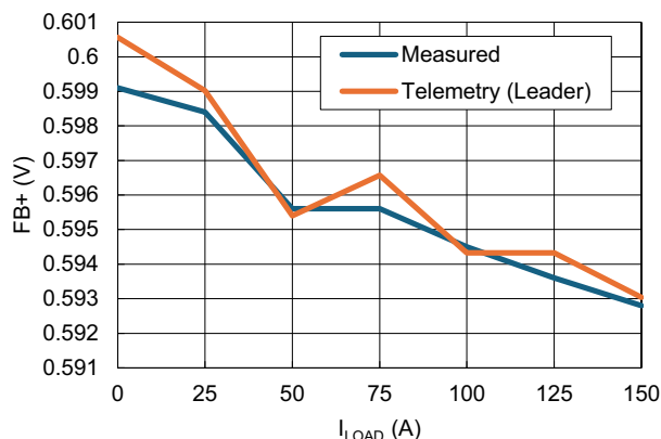
Figure 86. FB+ Telemetry (VDD = 5V, PVIN = 5V, I_{LOAD} = 0A , 50 Averages)
