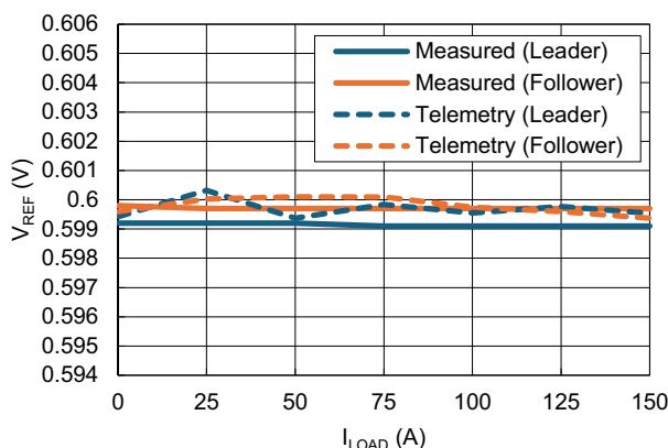
Figure 83. VREF Telemetry ( V_{DD} = 12V , PVIN = 12V , I_{LOAD} = 0A , 50 Averages)
