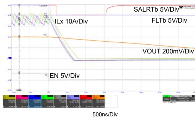
Figure 47. Shutdown with the EN Pin ( V_{DD} = 5V , PVIN = 5V , I_{LOAD} = 150A )
