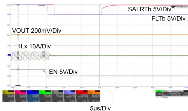
Figure 46. Shutdown with the EN Pin ( V_{DD} = 5V , PVIN = 5V , I_{LOAD} = 0A )
