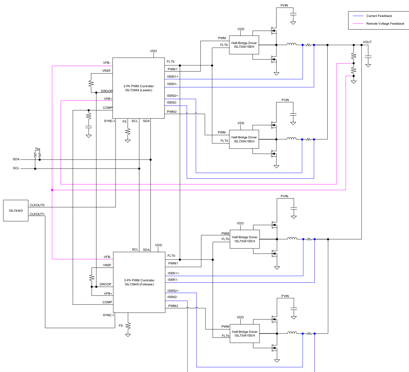
Figure 1. Block Diagram
