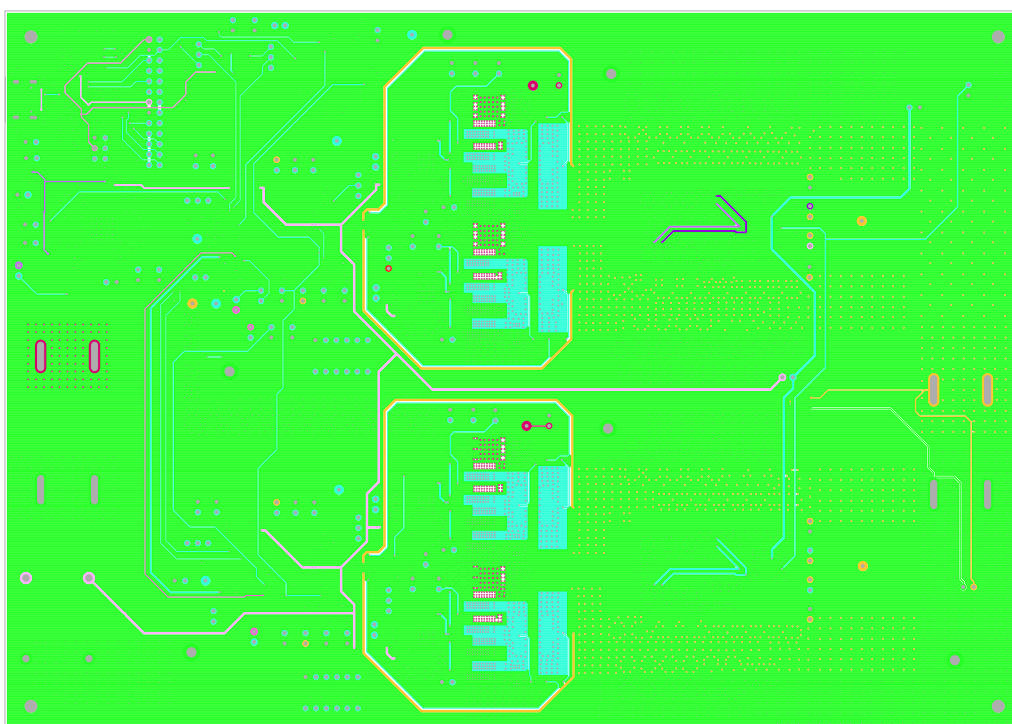
Figure 31. Layer 3
