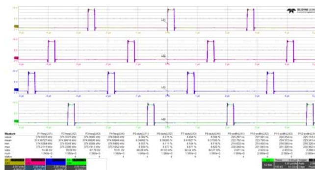
Figure 63. Phase Node Steady State Jitter (VDD = 12V, PVIN = 12V, I_LOAD = 150A)
