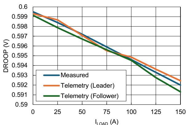
Figure 84. DROOP Telemetry ( V_{DD} = 5V , PVIN = 5V , I_{LOAD} = 0A , 50 Averages)
