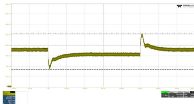
Figure 75. Load Transient Response (VDD = 12V, PVIN = 12V, I_{LOAD} = 75A \rightarrow 150A \rightarrow 75A , Slew = 200A/μs)
