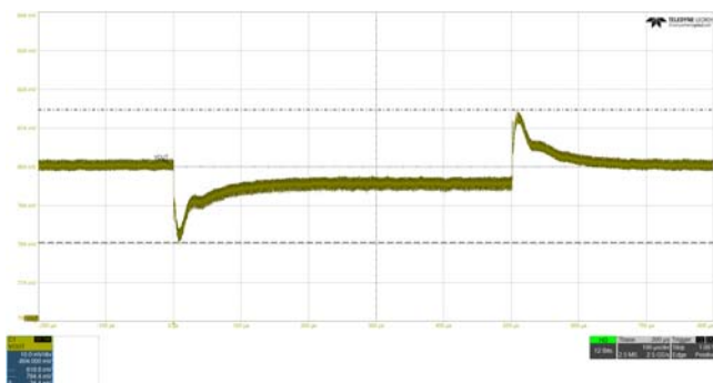
Figure 74. Load Transient Response (VDD = 12V, PVIN = 12V, I_{LOAD} = 0A \rightarrow 75A \rightarrow 0A , Slew = 200A/μs)
