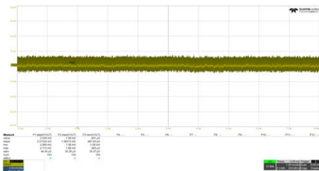
Figure 76. VOUT Ripple measured at TP76 PH2 Output (VDD = 5V, PVIN = 5V, I_{LOAD} = 0A , VOUT_COMMAND = 0.6V, 20MHz BW filter, AC-Coupled)
