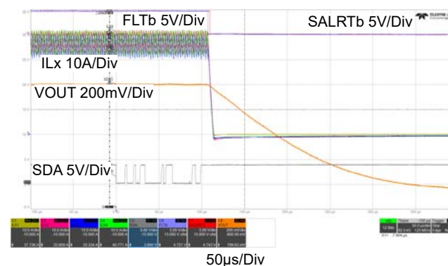
Figure 55. Shutdown with the OPERATION Bit (VDD = 5V, PVIN = 5V, I_{LOAD} = 150A , OPERATION = 0x80 to 0x00)
