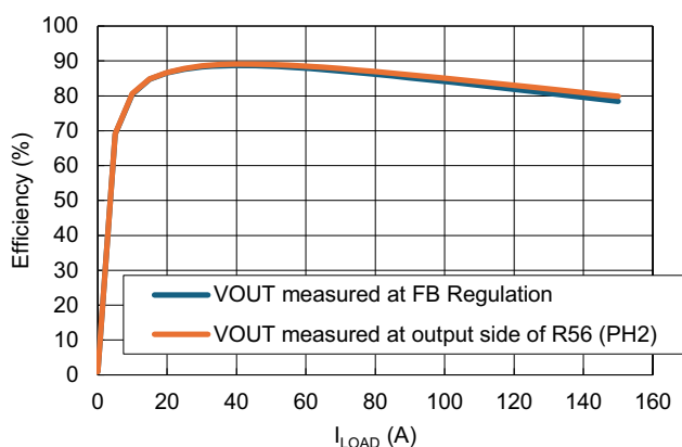
Figure 94. Efficiency (VDD = 5V, PVIN = 5V)
