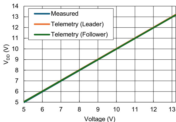
Figure 80. VDD Telemetry ( I_{LOAD} = 0A , 50 Averages)
