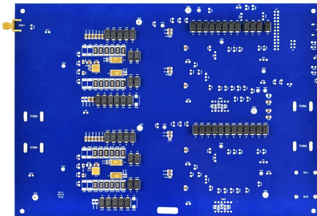
Figure 19. ISL73849SLHEV2Z4 Evaluation Board (Bottom)
