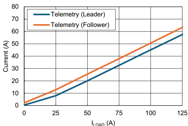
Figure 89. IOOUT Telemetry (VDD = 12V, PVIN = 12V, 50 Averages)
