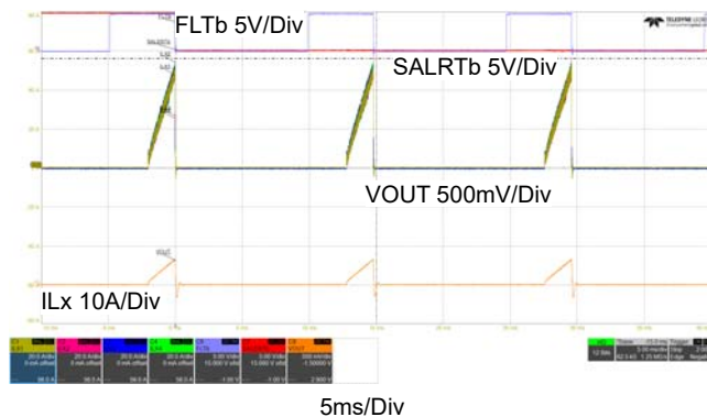
Figure 71. Overcurrent Protection on FLTb Startup (VDD = 12V, PVIN = 12V, OC_{TH} = 37.5mV )
