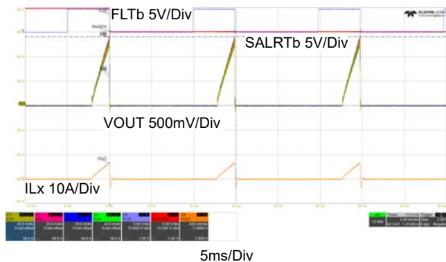
Figure 70. Overcurrent Protection on FLTb Startup (VDD = 5V, PVIN = 5V, OC_{TH} = 37.5mV )
