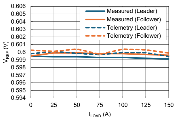
Figure 82. VREF Telemetry ( V_{DD} = 5V , PVIN = 5V , I_{LOAD} = 0A , 50 Averages)
