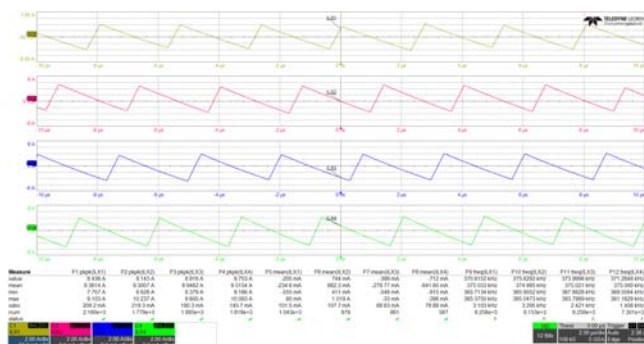
Figure 64. 4-Phase Inductor Current (VDD = 5V, PVIN = 5V, I_LOAD = 0A)
