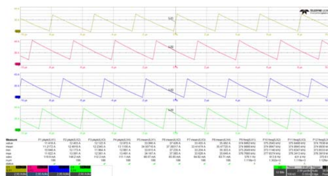
Figure 67. 4-Phase Inductor Current (VDD = 12V, PVIN = 12V, I_LOAD = 150A)
