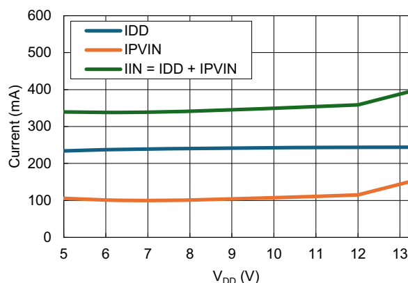
Figure 98. Operating Supply Current (EN = High, FLT B = High, OUTEN = High)
