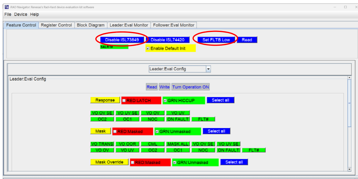
Figure 8. Enable Switching
