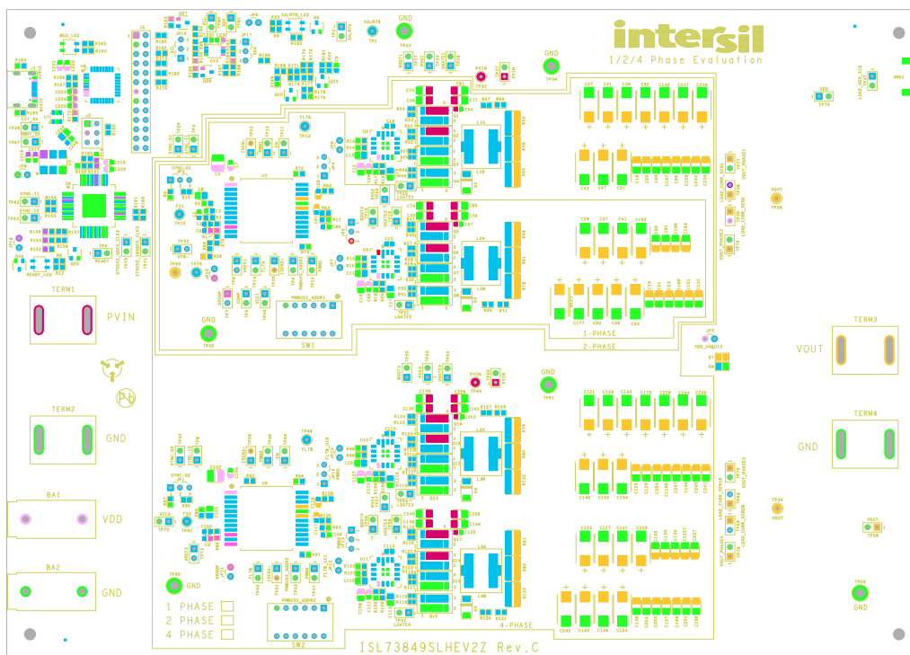
Figure 28. Silkscreen Top Layer
