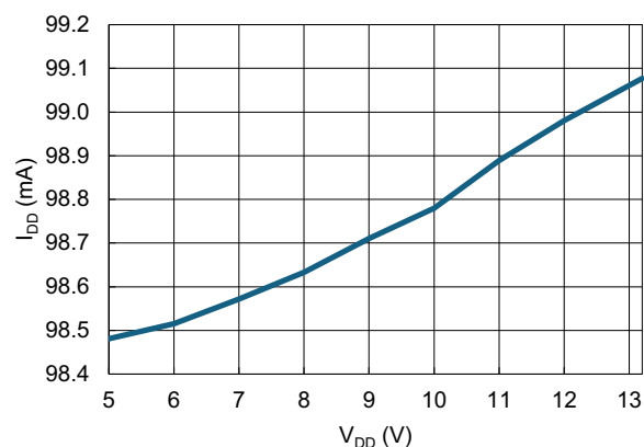
Figure 97. VDD Standby Current (FLTb = Low, EN = High, OUTEN = Low)
