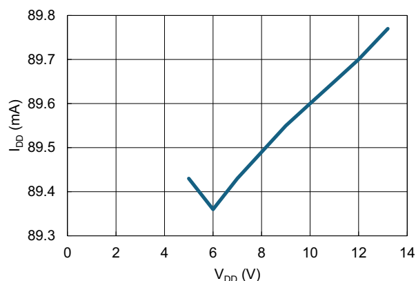
Figure 99. VDD Current with OPERATION Bit Low (EN = High, OPERATION = 0x00)
