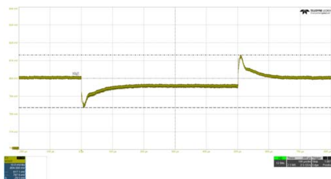
Figure 72. Load Transient Response (VDD = 5V, PVIN = 5V, I_{LOAD} = 0A \rightarrow 75A \rightarrow 0A , Slew = 200A/\mu s )
