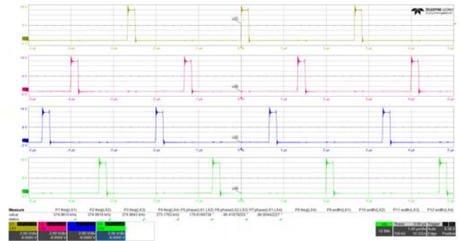
Figure 59. Phase Shifting ( V_{DD} = 12V , P_{VIN} = 12V , I_{LOAD} = 0A )
