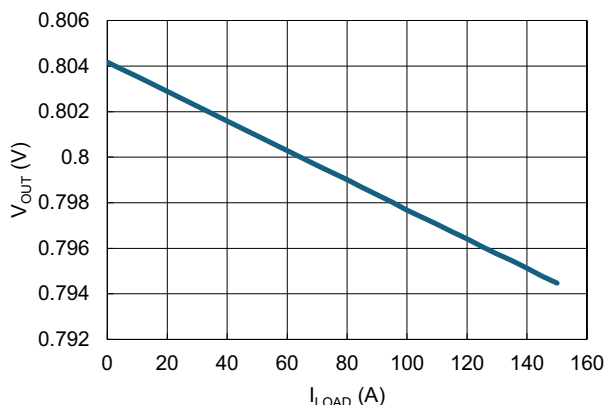
Figure 92. DROOP Regulation (VDD = 5V, PVIN = 5V)
