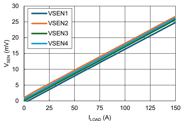
Figure 69. ISEN1-4 Current Sharing (VDD = 12V, PVIN = 12V, I_{LOAD} = 0A )
