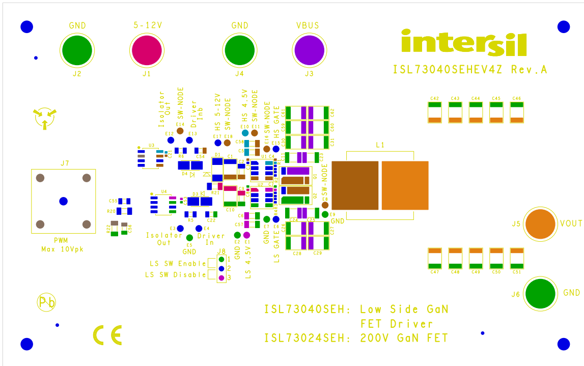
Figure 6. Silkscreen Top
