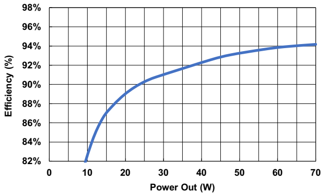
Figure 13. V_{BUS} = 100\text{V} , V_{OUT} = 28\text{V}
