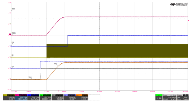
Figure 15. Enabled Turn-on, 1.1Ω load
