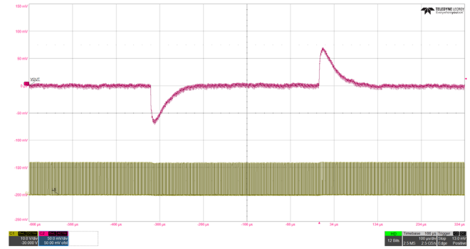
Figure 19. 1A DC (3.3Ω Load) with 2A Load Transient (Internal Compensation)
