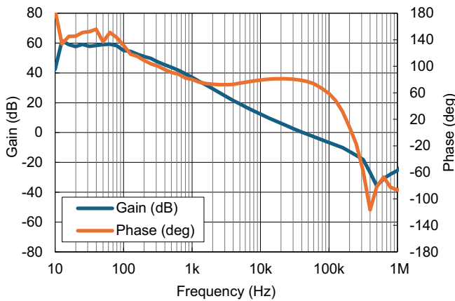
Figure 22. Bode Plot: External Comp, P_{VIN} = 12V , V_{OUT} = 3.3V , I_{OUT} = 3A
