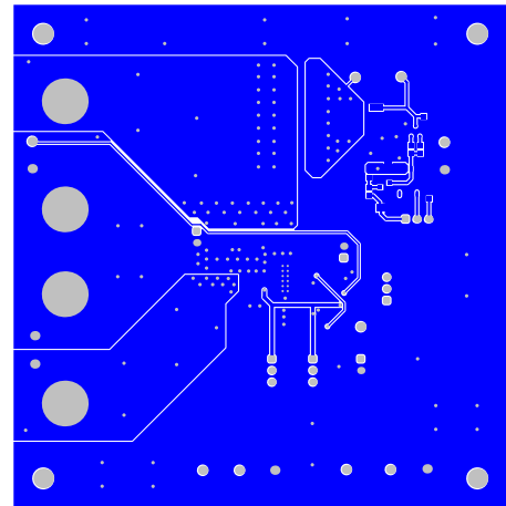
Figure 9. Bottom Layer
