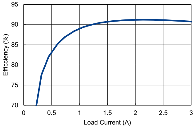
Figure 12. Efficiency
