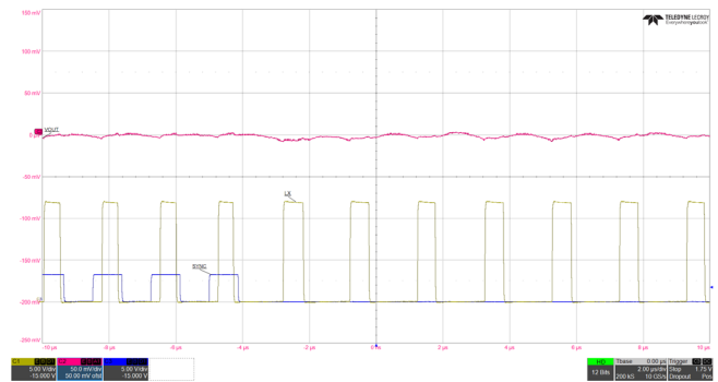
Figure 17. 575kHz SYNC Input Stop
