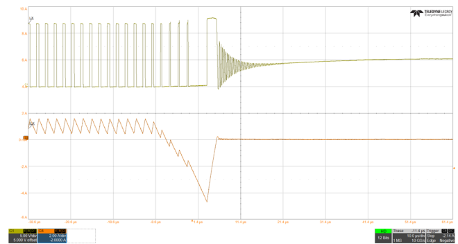
Figure 21. Negative Overcurrent Protection
