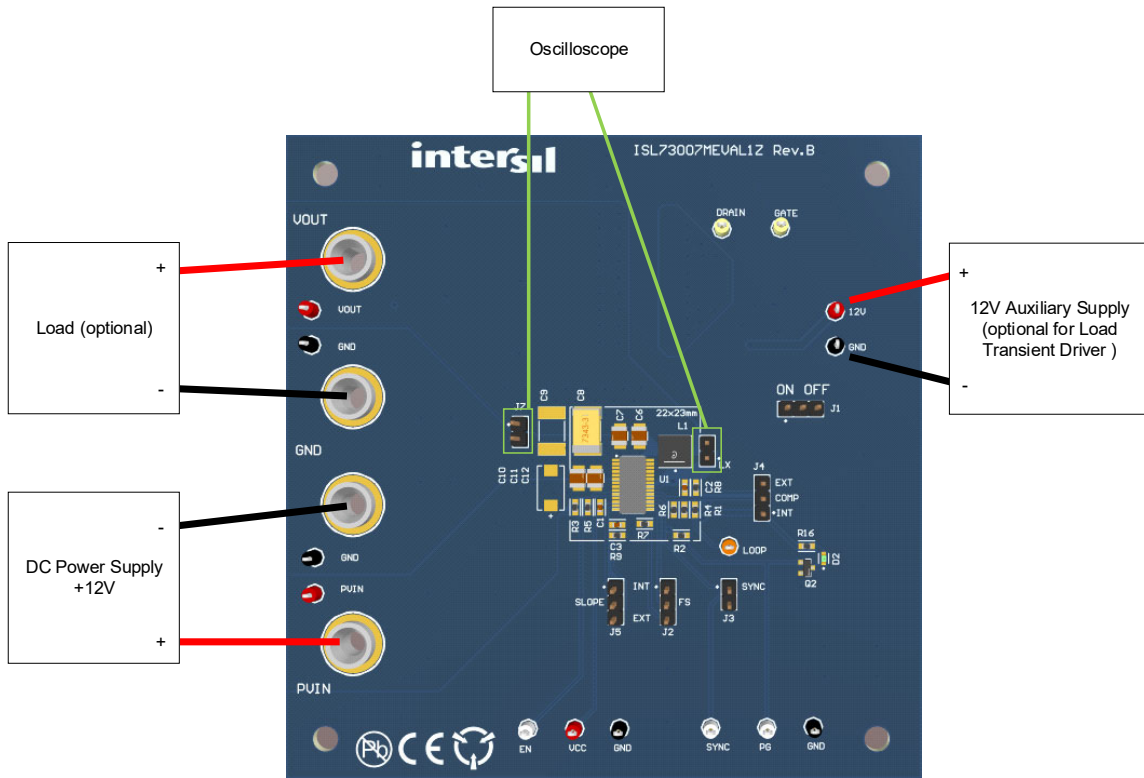
Figure 1. Basic Evaluation Test Setup Block Diagram
