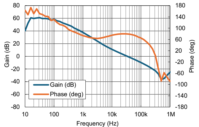
Figure 23. Bode Plot: Internal Comp, P_{VIN} = 12V , V_{OUT} = 3.3V , I_{OUT} = 3A
