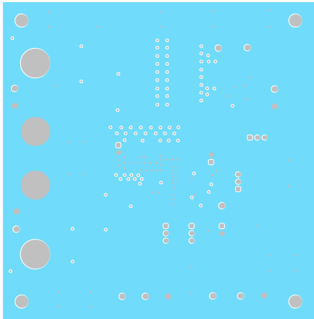
Figure 8. Layer 3
