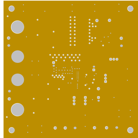
Figure 7. Layer 2
