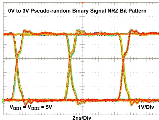
Figure 22. ISL71710M 150Mbps Eye Diagram
