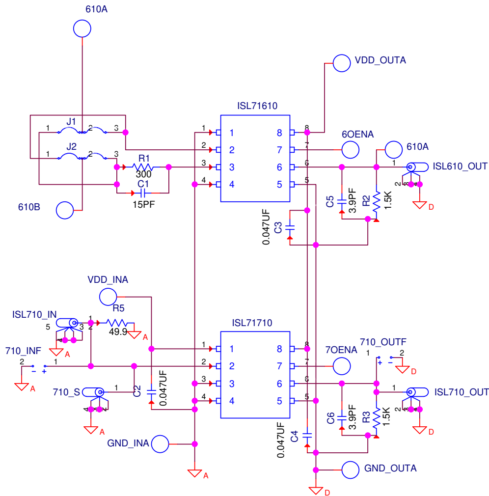
Figure 5. Schematic
