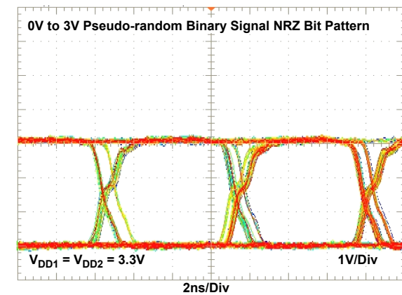
Figure 20. ISL71710M 150Mbps Eye Diagram
