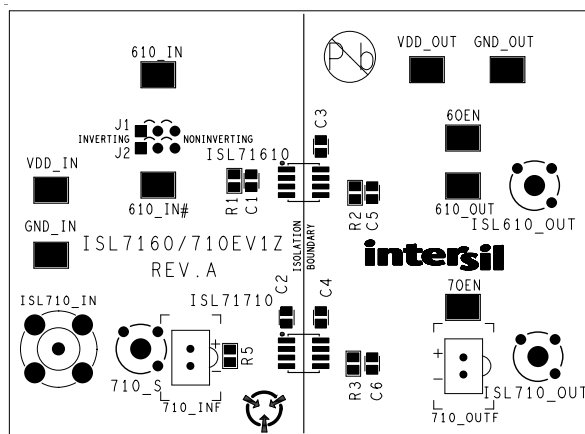
Figure 8. Top Layer Silk Screen
