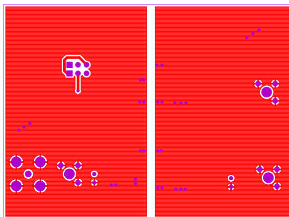
Figure 7. Bottom Layer
