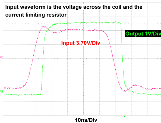
Figure 14. ISL71610M Switching, Coil Current \sim\pm 20\text{mA} , C_{\text{BOOST}} = \text{open} , C_{\text{OUT}} = 15\text{pF} , V_{\text{DD}} = 5\text{V}
