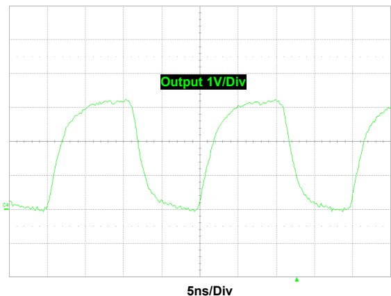
Figure 9. ISL71610M Output at 100Mbps, C_{\text{BOOST}} = 15\text{pF} , C_{\text{OUT}} = 15\text{pF} , V_{\text{DD}} = 3.3\text{V}
