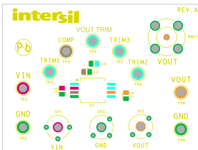
FIGURE 10. TOP SILKSCREEN
