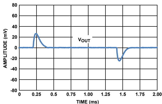
FIGURE 5. LOAD TRANSIENT ( \Delta I_L = 1\text{mA} )
