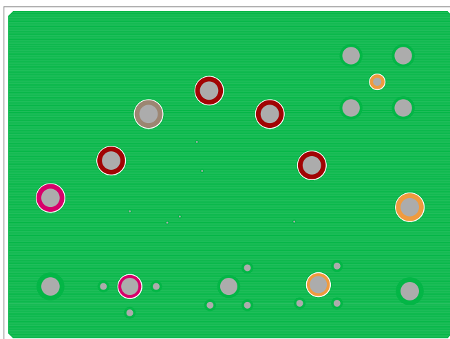
FIGURE 9. BOTTOM LAYER (VIEWED FROM TOP)
