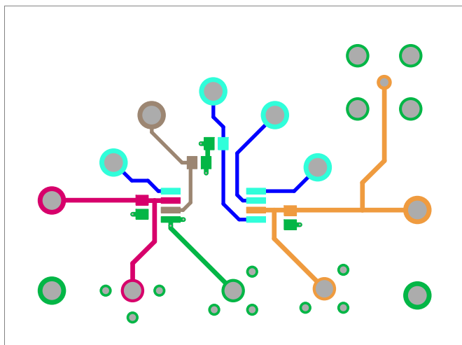
FIGURE 8. TOP LAYER
