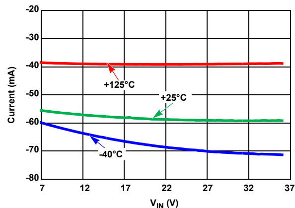
Figure 17. Short-Circuit to GND
