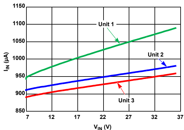
Figure 13. I_{IN} vs V_{IN} , Three Units
