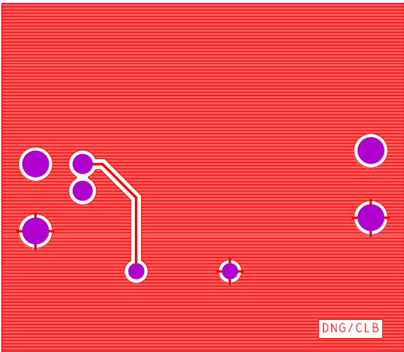
Figure 6. Bottom Layer
