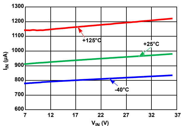
Figure 14. I_{IN} vs V_{IN} , Three Temperatures
