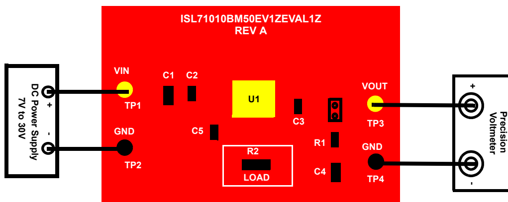
Figure 2. Basic Evaluation Test Setup Block Diagram (Measure V OUT of the Voltage Reference)
