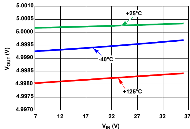
Figure 12. Line Regulation, Three Temperatures
