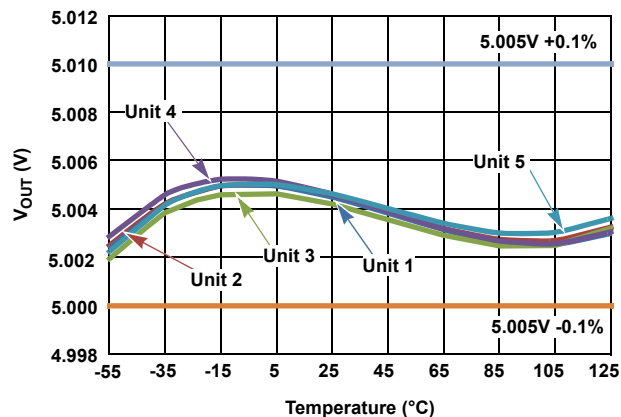
Figure 9. 5.005V V_{OUT} Limits Plot
