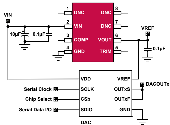
Figure 1. ISL71010BM50EV1Z Block Diagram
