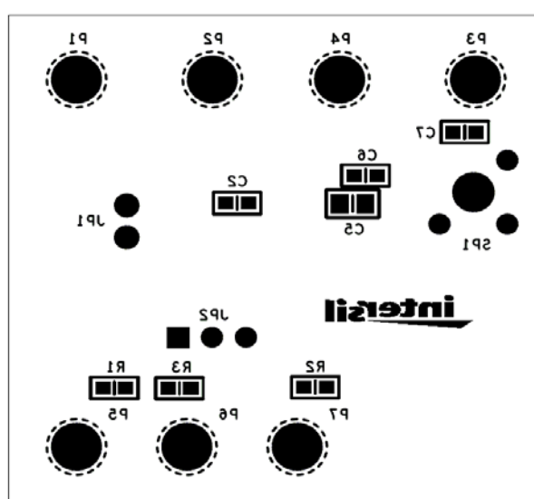
BOTTOM SILK
