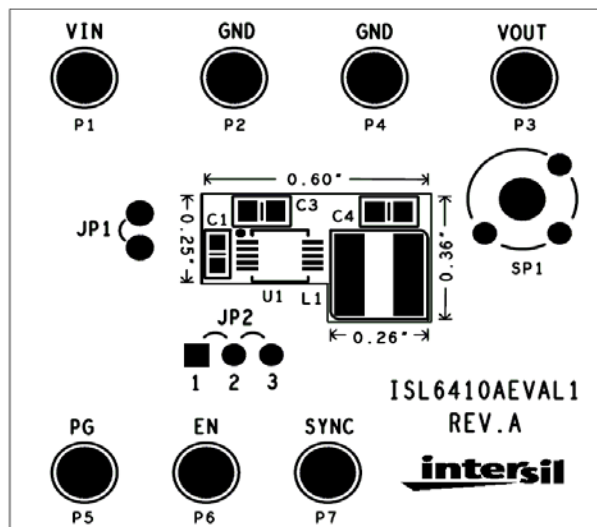
TOP SILK
