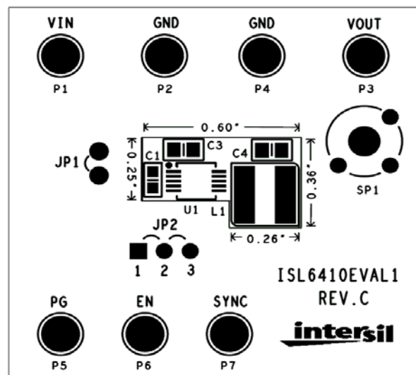
TOP SILK
