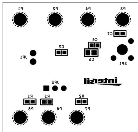
BOTTOM SILK
