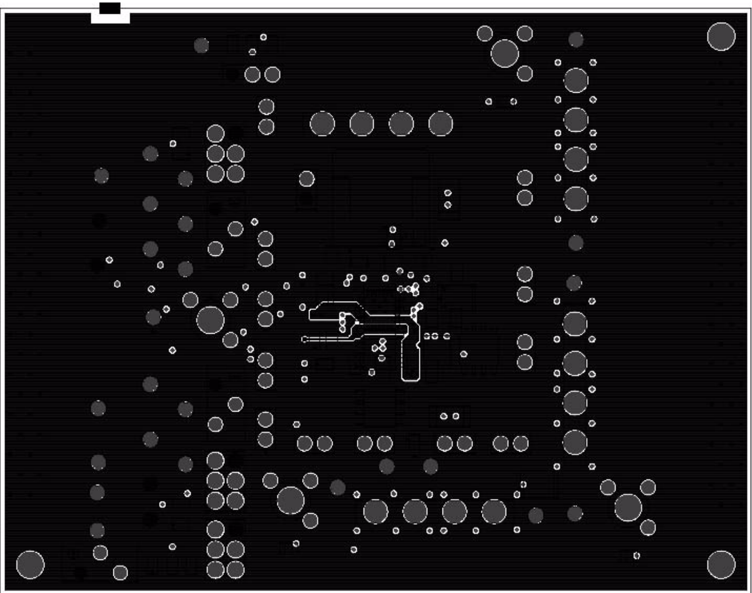
FIGURE 7. L4 GND
