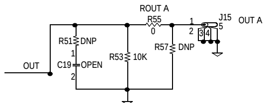
FIGURE 3. 1/2 OUTPUT STAGE
