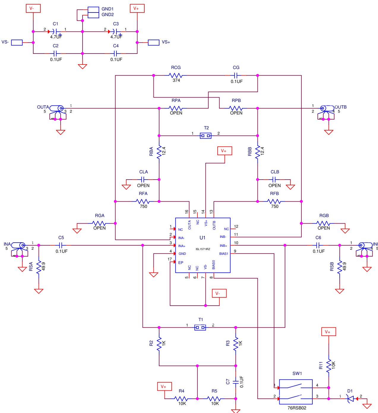
Figure 4. Schematic
