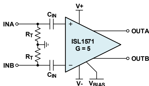
Figure 1. ISL1571IRZ-EVAL Block Diagram
