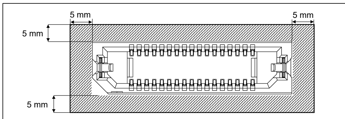
Figure 4-1 Area where Restriction Applies to Mounted Components
