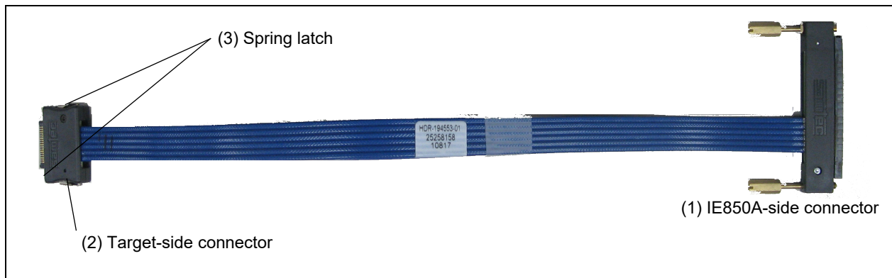
Figure 2-2 Names of the Parts of the Trace Cable for the IE850A (RTE0T0850AKCAC0000J)
