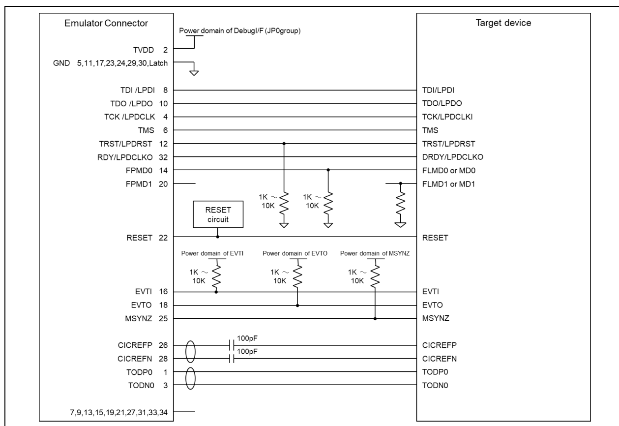
Figure 4-4 Example of Recommended Connections for Debugging (4-Pin LPD, JTAG) and Tracing (One Lane)
