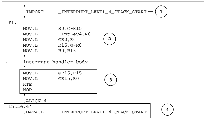
Figure 11.1 ISR Implementation in Assembler
