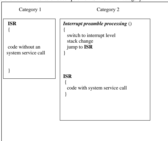
Figure 6.3 ISR Description in Each Category
