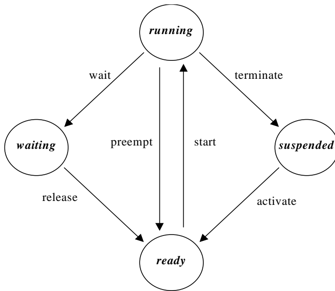
Figure 4.2 Extended Task State
