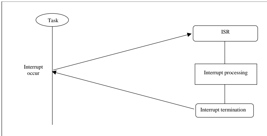
Figure 6.1 Flow of Interrupt Category 1
