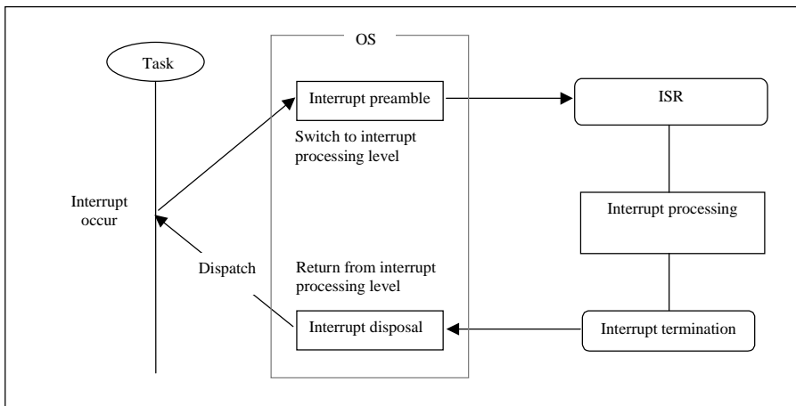
Figure 6.2 Flow of Interrupt Category 2
