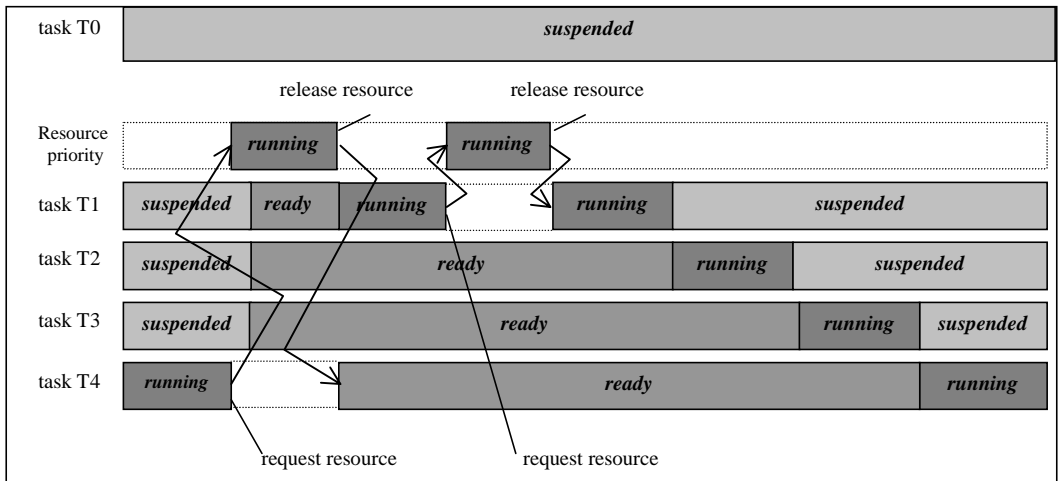
Figure 7.1 Resource Priority Assignment
