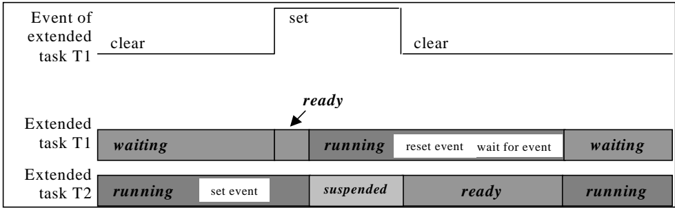
Figure 8.2 Synchronisation of Non-Preemptive Extended Tasks
