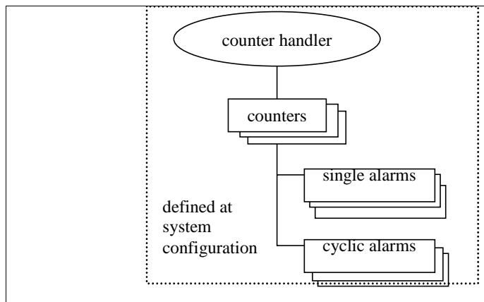
Figure 9.1 Layered Model of Alarm Management
