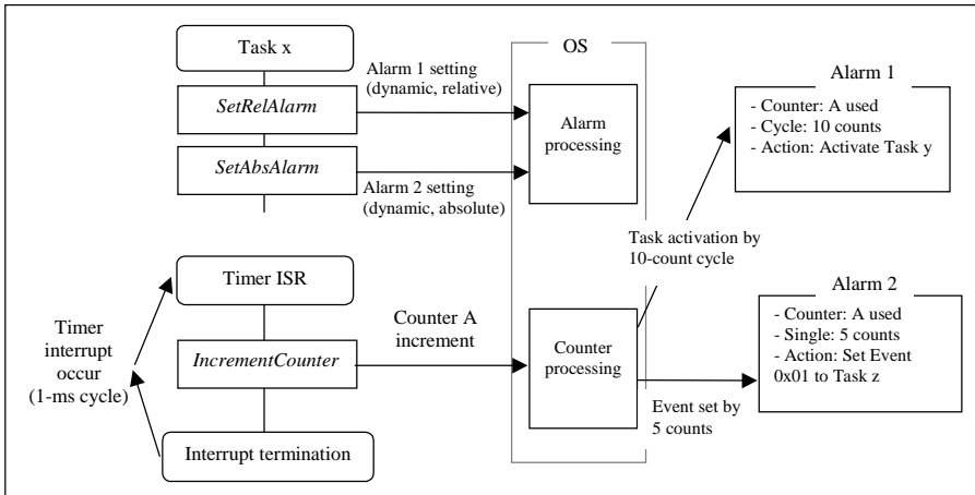
Figure 9.4 Example for Using Counter and Alarm
