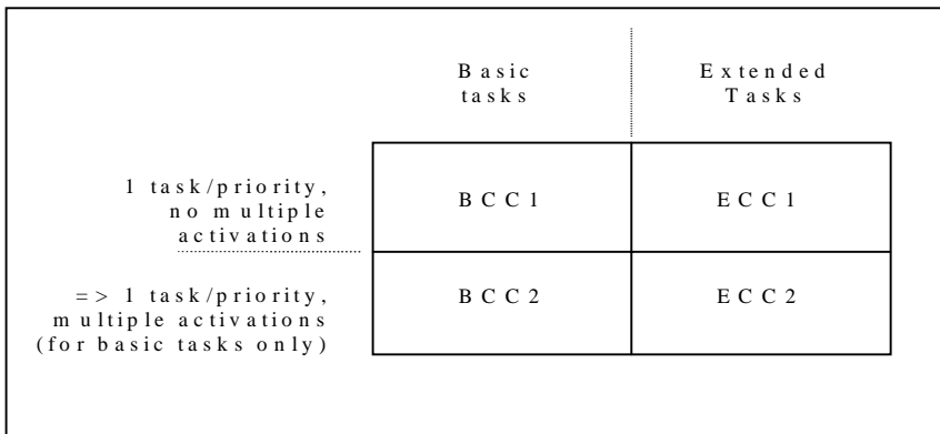
Figure 3.2 OS Conformance Classes
