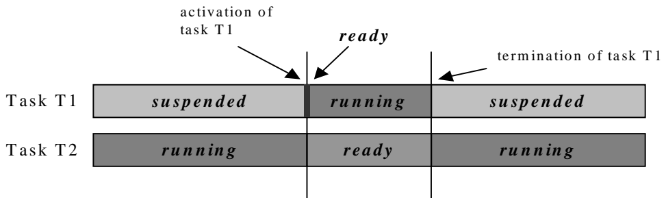
Figure 5.3 Full-Preemptive Scheduling
