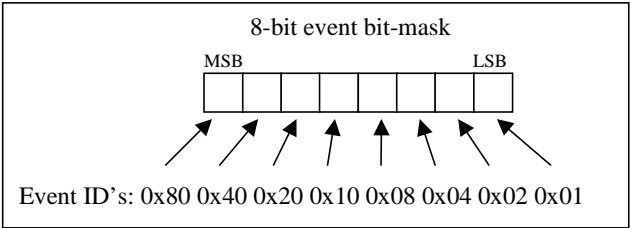
Figure 8.3 Event IDs
