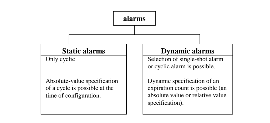
Figure 9.3 Alarm Classification
