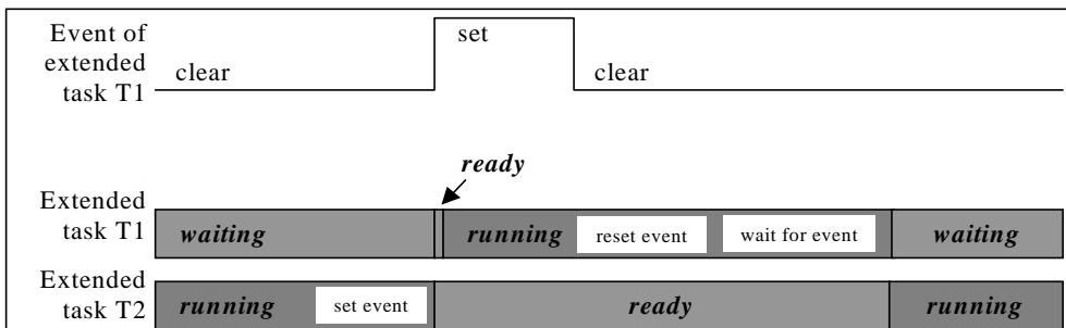
Figure 8.1 Synchronisation of Full Preemptive Extended Tasks
