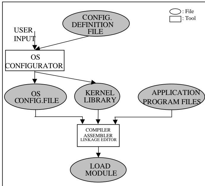
Figure 2.1 OS Application Building Flow
