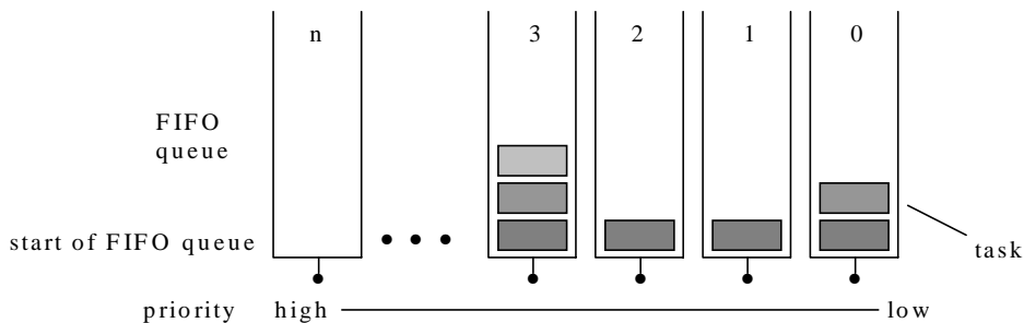
Figure 5.1 Ready Queues
