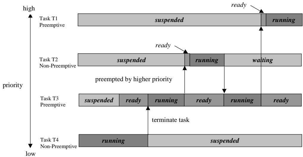
Figure 5.4 Mixed-Preemptive Scheduling
