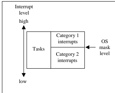
Figure 6.4 Interrupt Level
