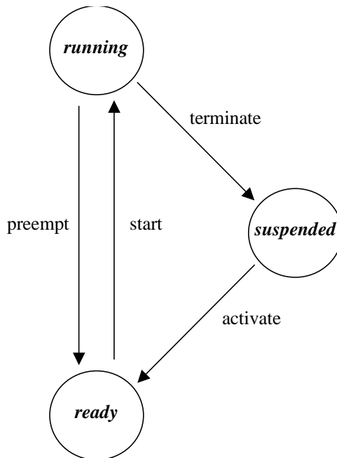
Figure 4.1 Basic Task State
