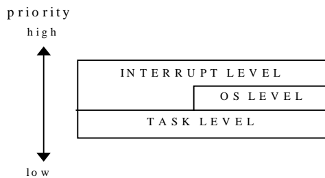
Figure 3.1 OSEK Processing Levels
