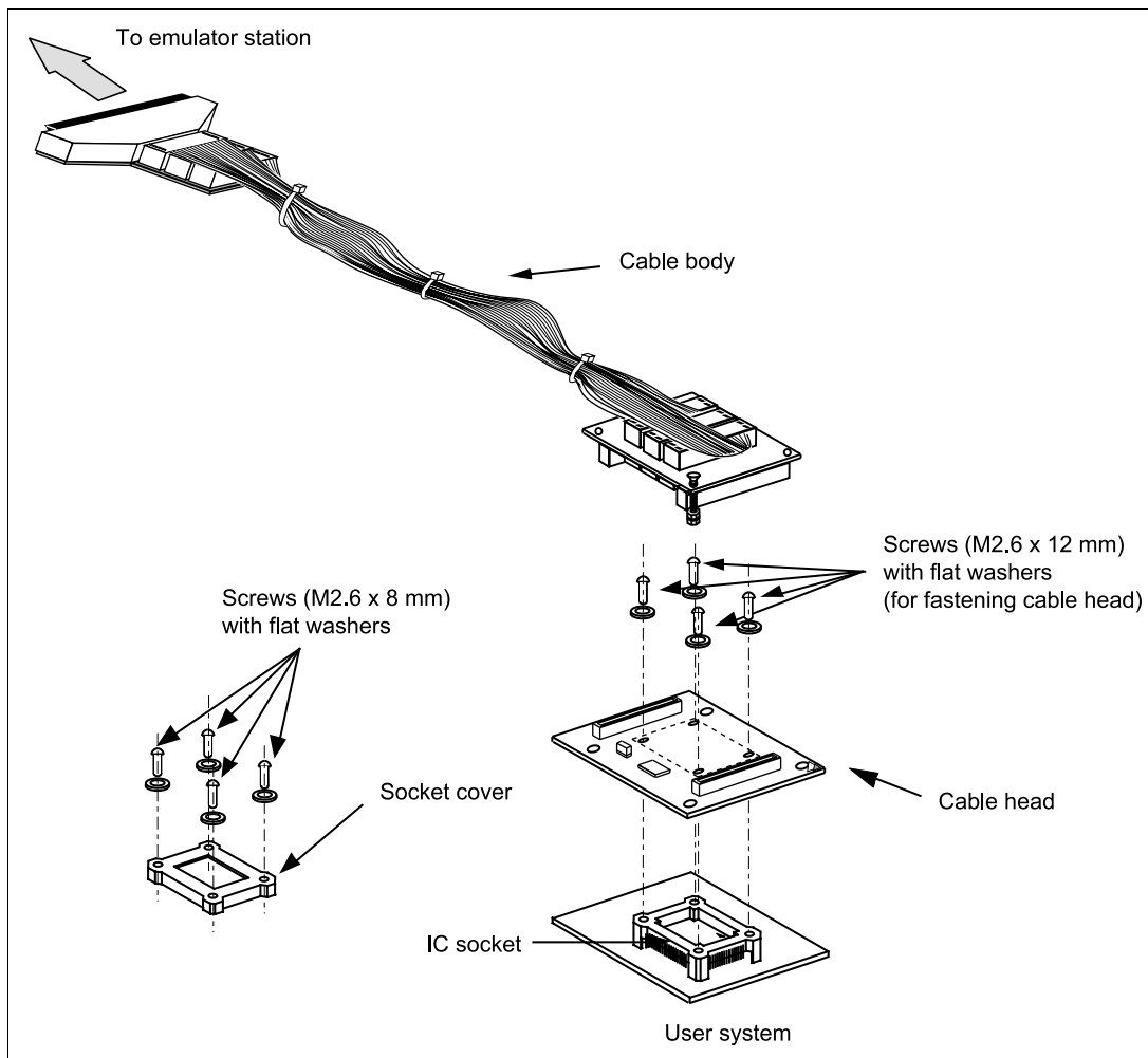
Figure 1 HS3657ECN62H User System Interface Cable
