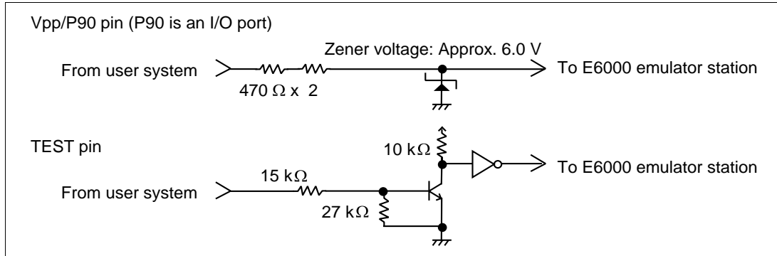
Figure 11 Vpp/P90 and TEST Pin Protection Circuits
