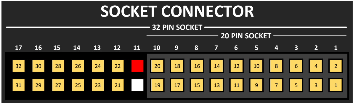
Figure 3: GreenPAK Socket Connector Pinout
