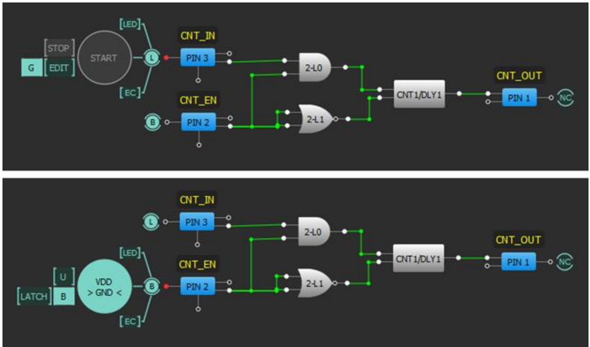
Figure 26: Signal Labels and Control Panels
