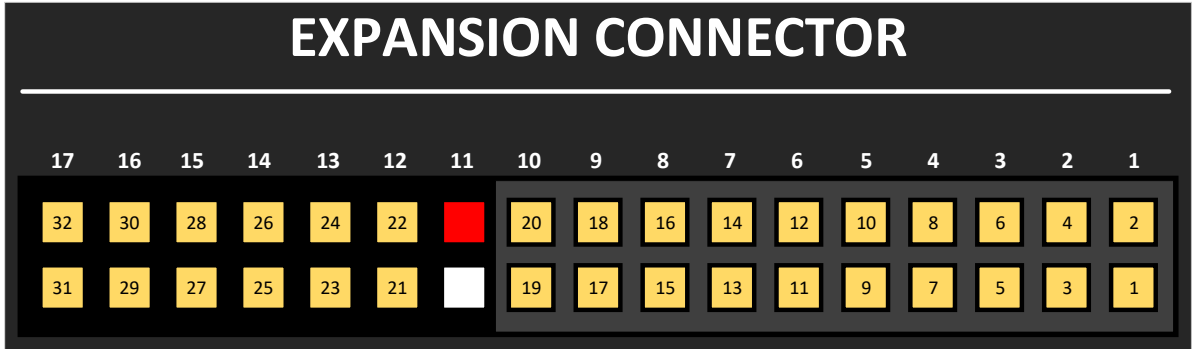
Figure 4: GreenPAK Expansion Connector Pinout
