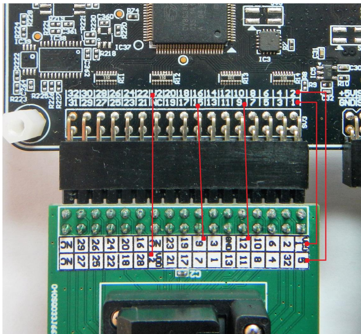
Figure 13: Some PINs and TPs Accordance (for SLG46880V)
