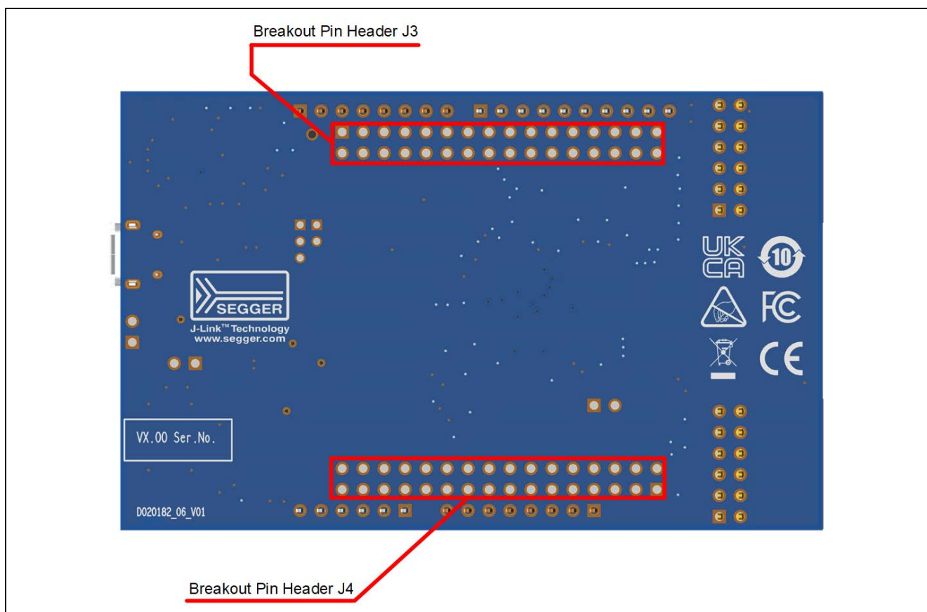
Figure 2. FPB-RA4T1 Board Bottom Side
