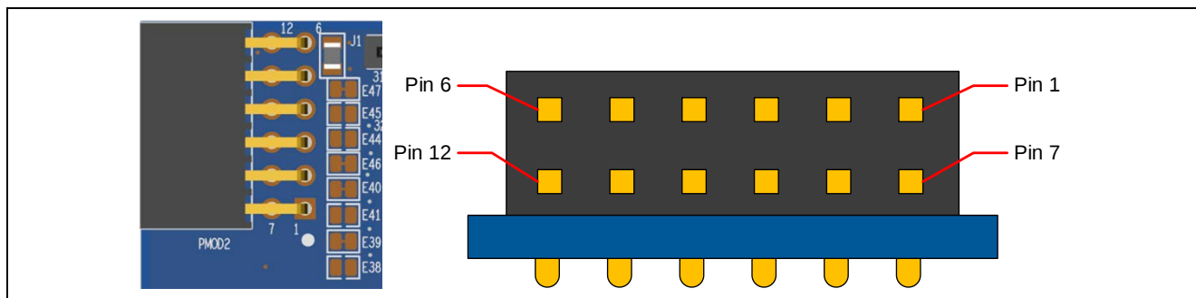
Figure 11. Pmod 2 Connector
