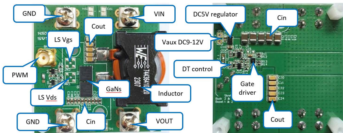
Figure 4. Top (Left) and Bottom (Right) Views
