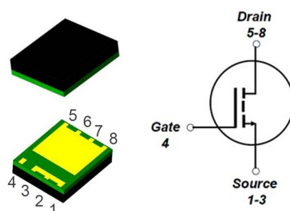
Figure 5. RTP100E2P6G1FL and Schematic Symbol
