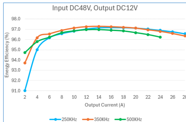
Figure 23. Energy Efficiency at Different Output Currents and Switching Frequencies
