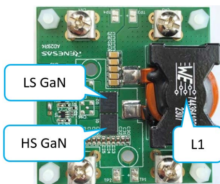
Figure 25. Measurement Location
