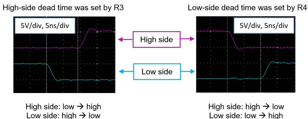
Figure 11. Resistor R3 and R4 Dead Time
