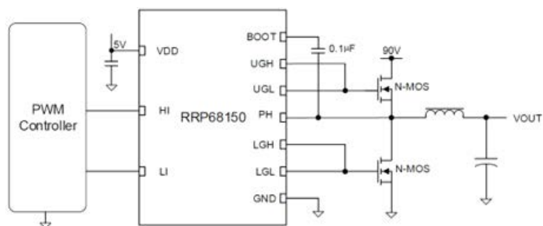
Figure 7. Typical Application
