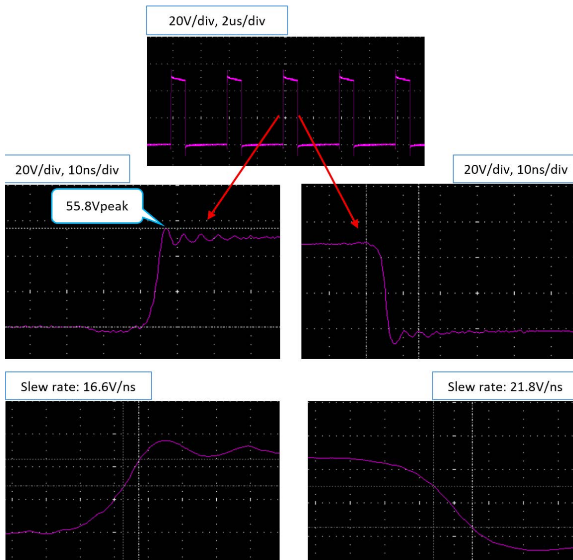
Figure 26. Switching Node Waveforms
