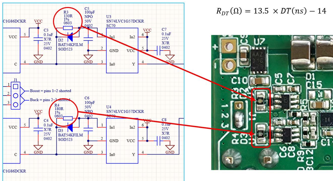
Figure 10. Resistors R3 and R4
