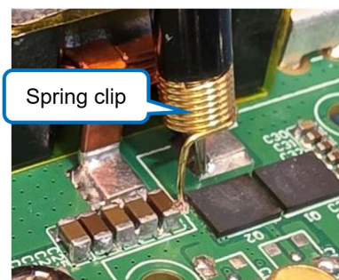
Figure 20. Passive Probe
