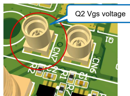
Figure 18. MMCX Jack
