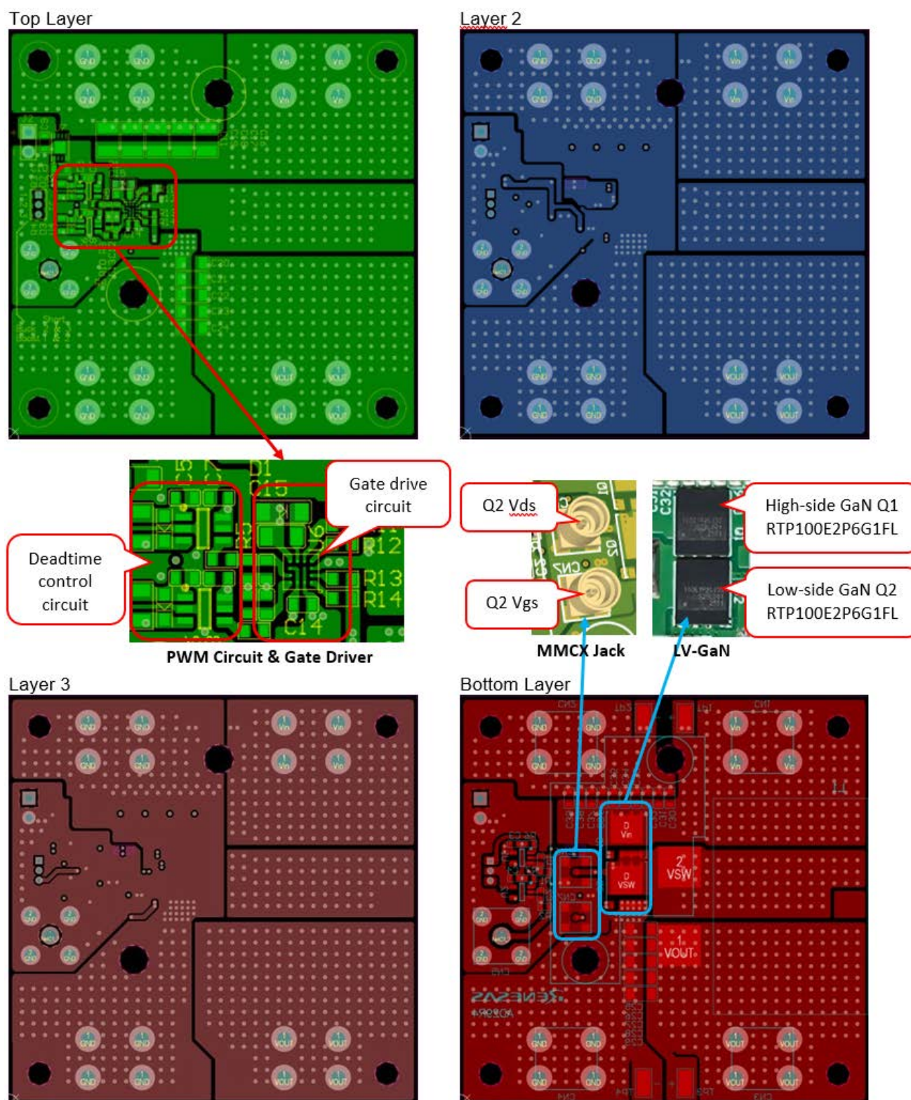
Figure 28. PCB Layout
