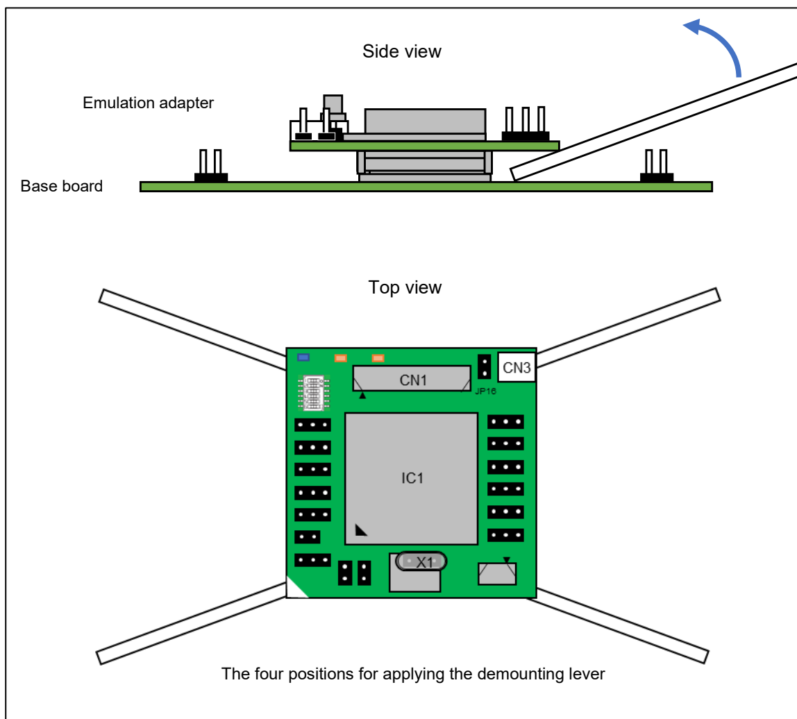
Figure 2-8 Demounting Lever
