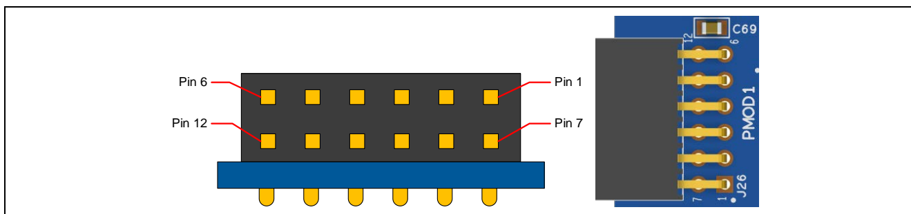
Figure 12. Pmod 1 Connector
