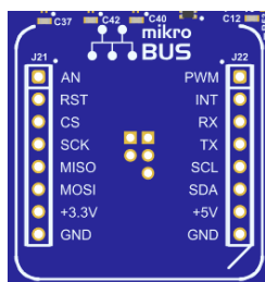
Figure 17. mikroBUS™ Connector
