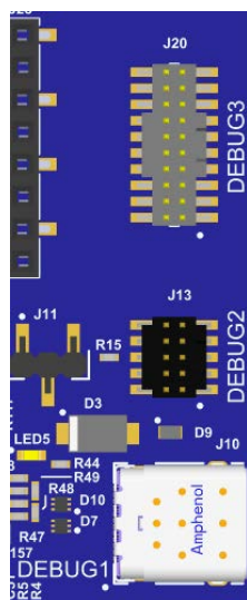
Figure 12. EK-RA4C1 Debug Interface
