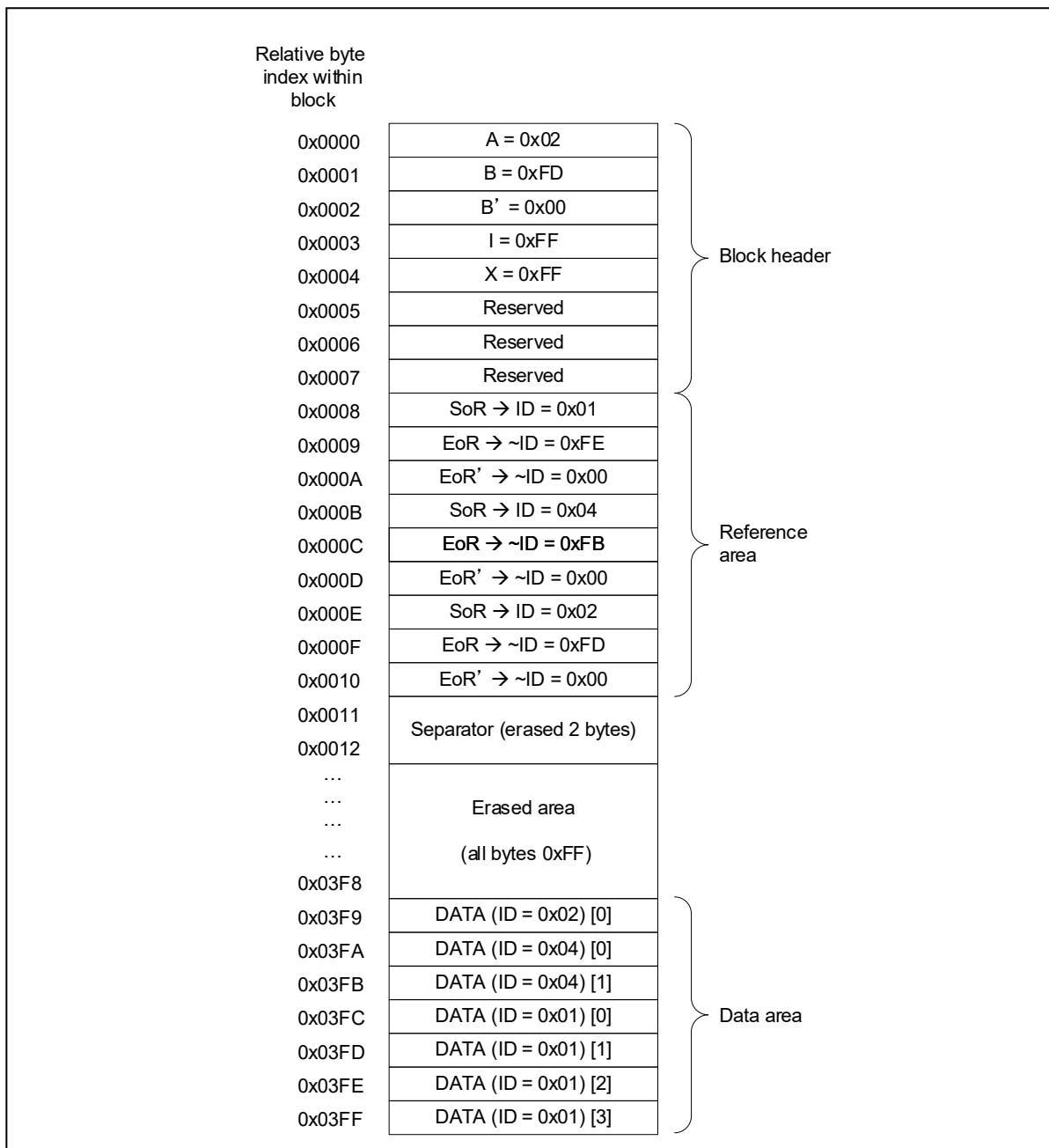
Figure 3-6 Example of an Active EES Block
