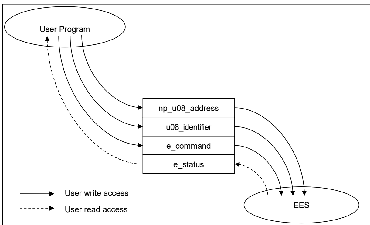
Figure 5-1 Request Structure (st_ees_request_t)
