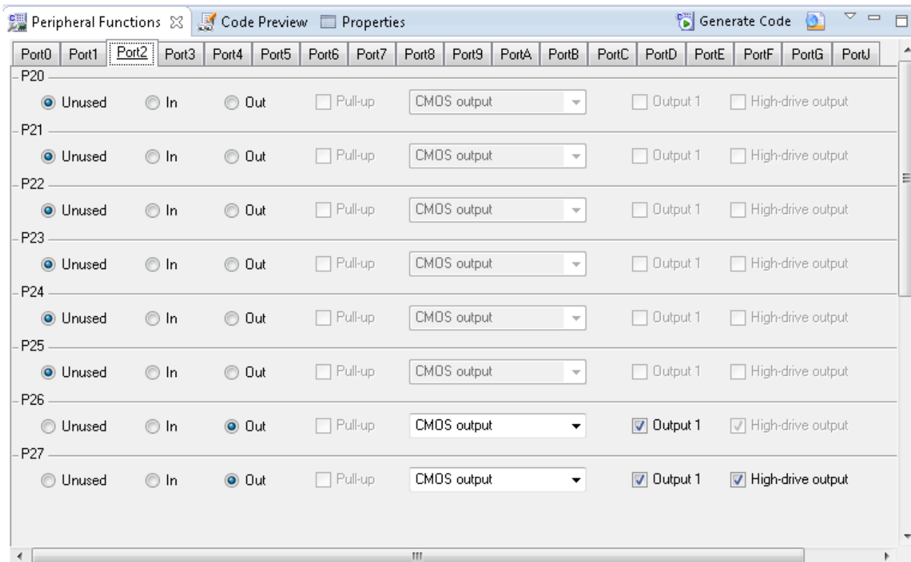
Figure 4-15 I/O ports – Port2
