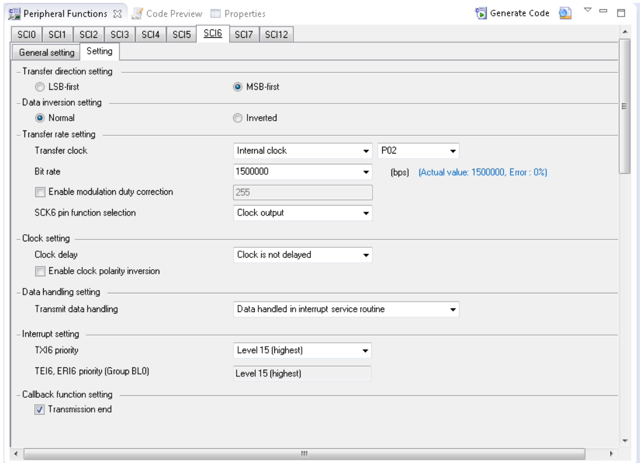
Figure 4-11 SCI6 SPI Master Setting
