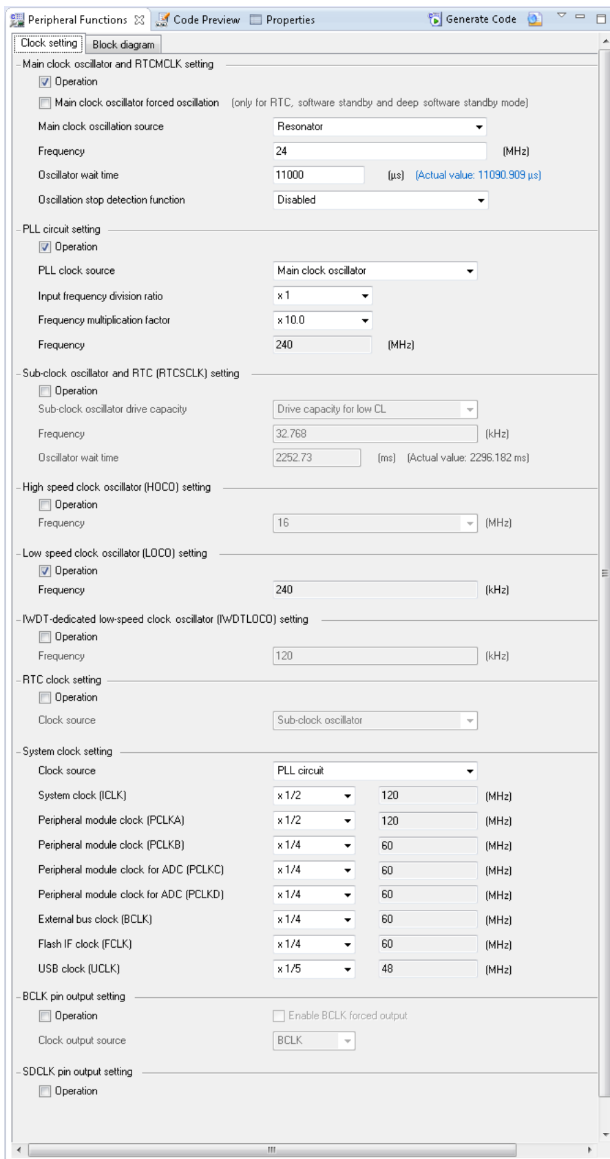
Figure 4-3 Clock setting tab
