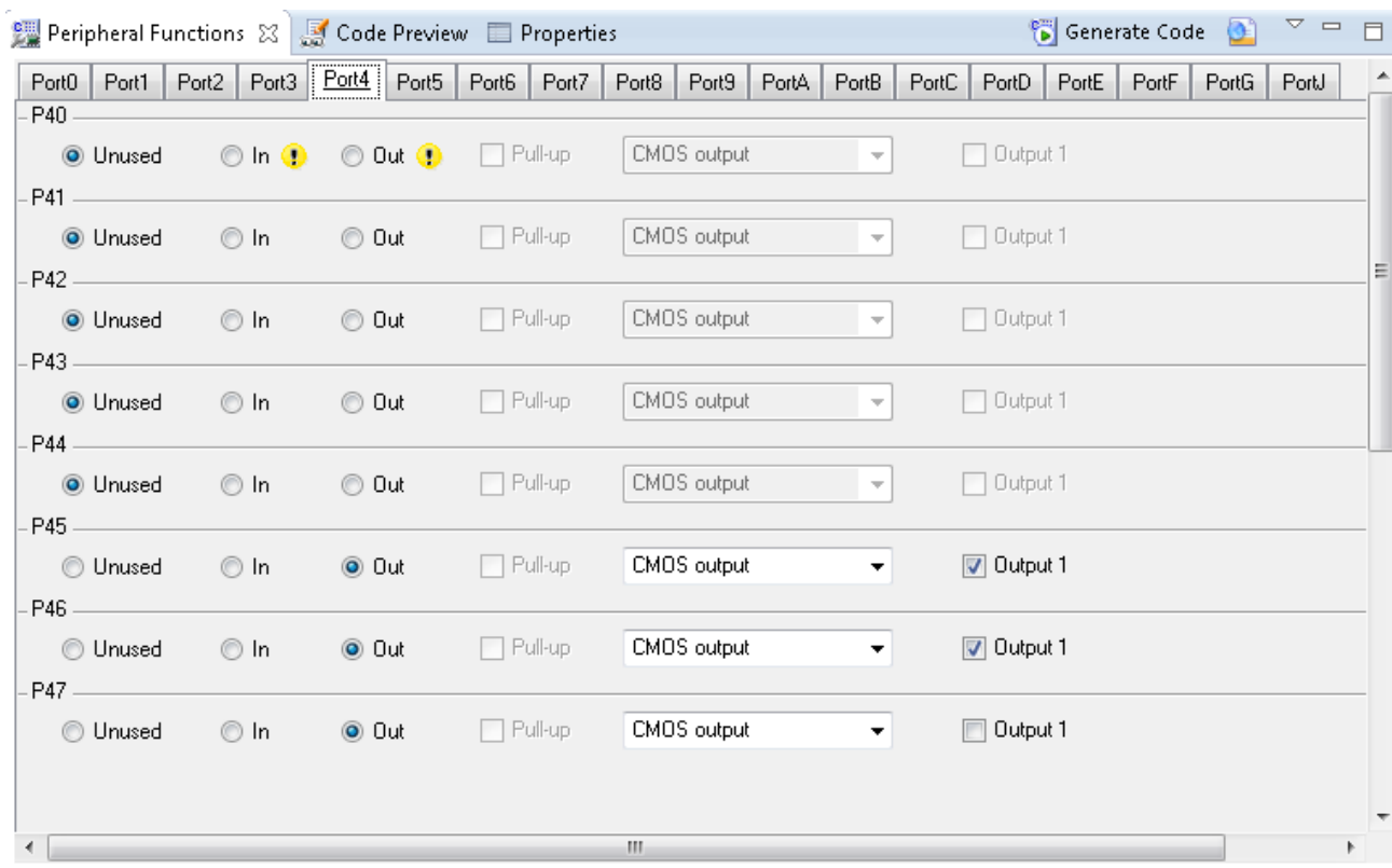
Figure 4-16 I/O ports – Port4
