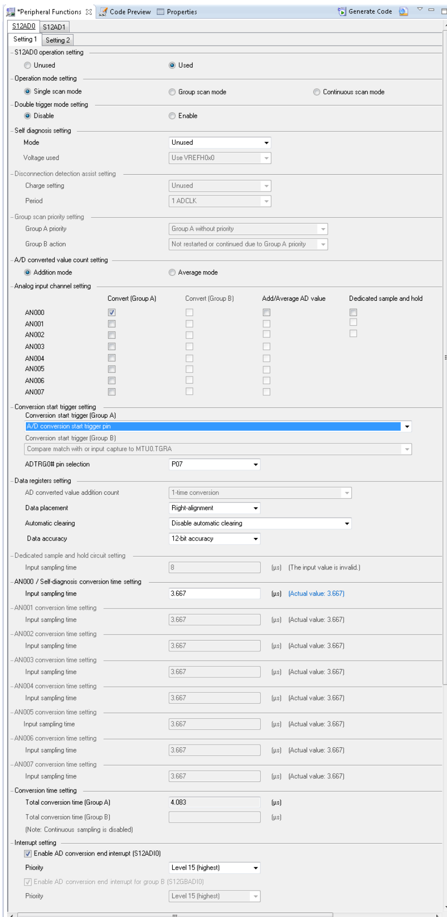
Figure 4-9 A/D Converter tab
