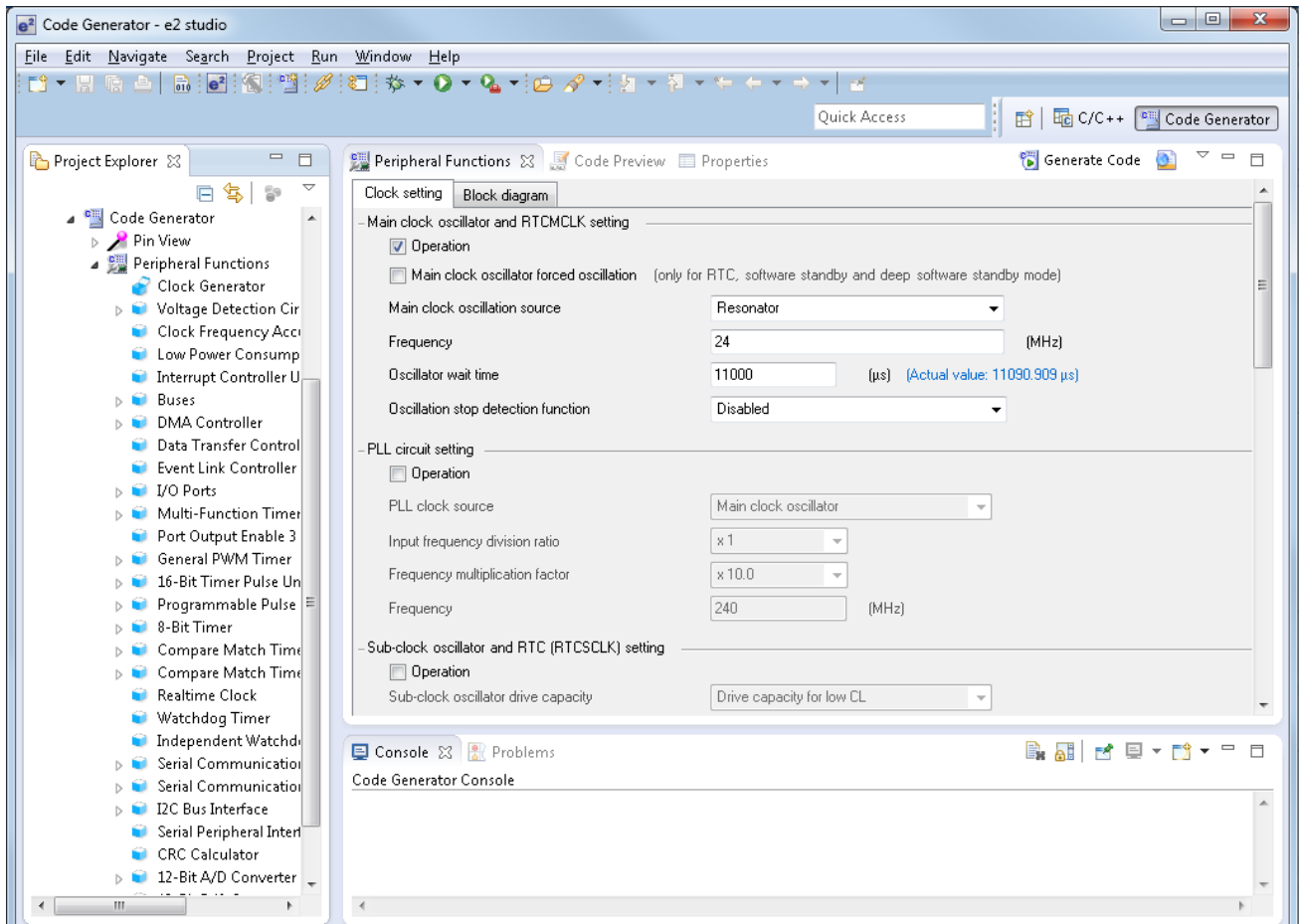
Figure 4-2 Initial View
