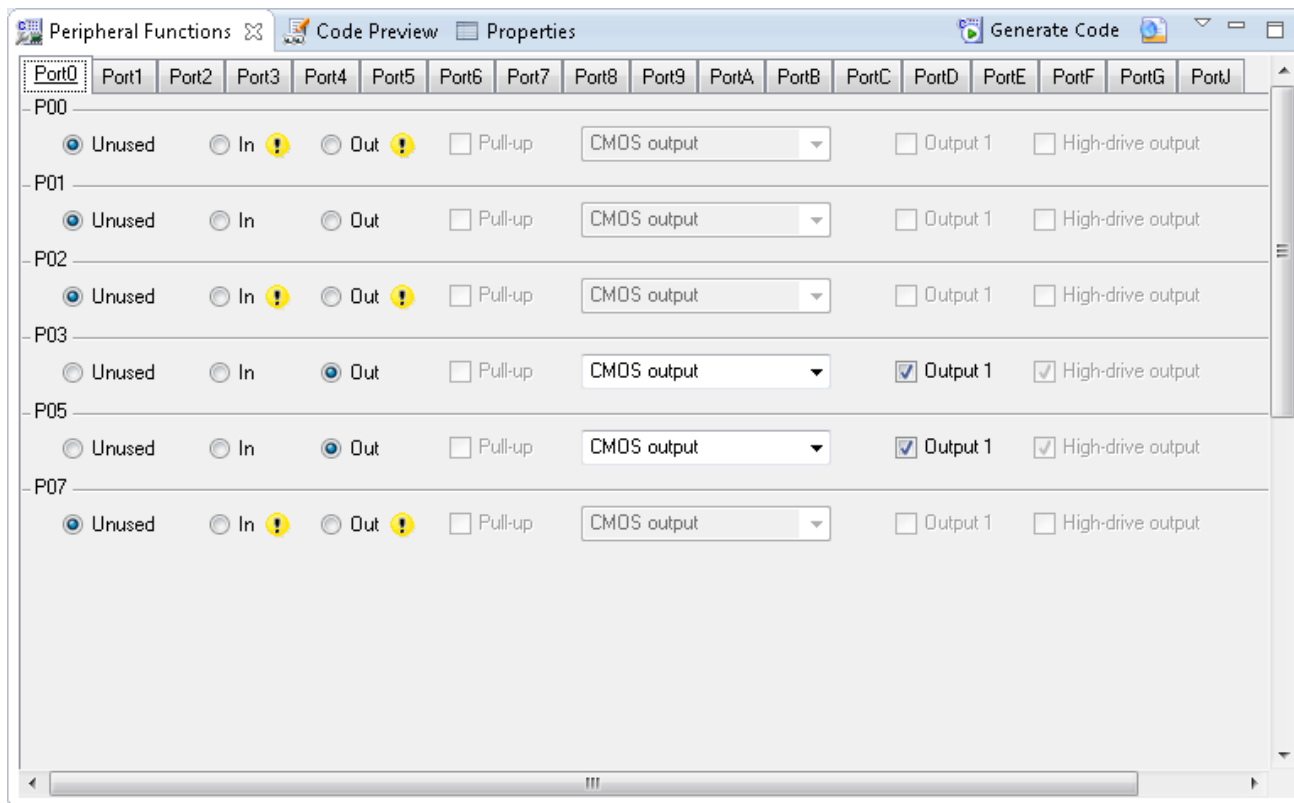
Figure 4-14 I/O ports – Port0
