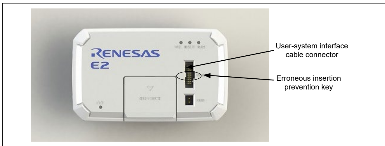
Figure 2.2 User-System Interface Cable Connector on the E2
