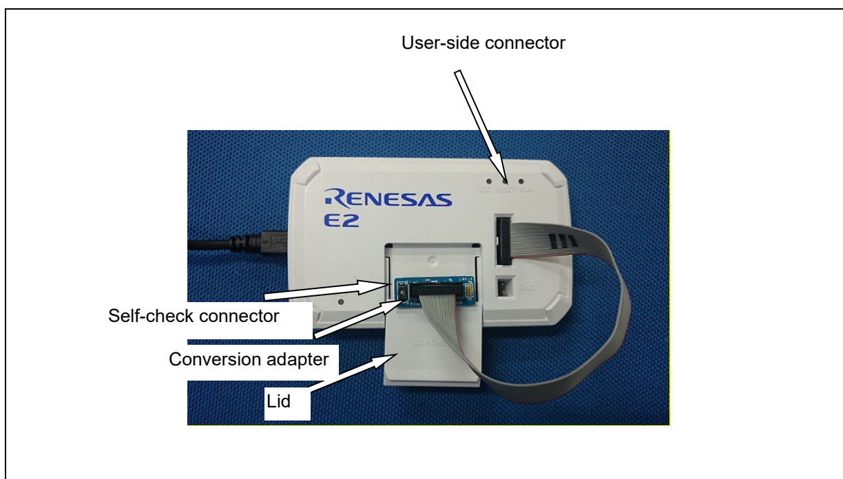
Figure A.1 Connecting the User-System Interface Cable during Executing the E2 SCP
