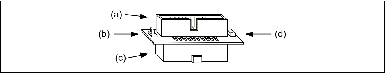
Figure 1.5 20-Pin (1.27-mm Pin Pitch) to 14-Pin (2.54-mm Pin Pitch) Connector Conversion Adapter
