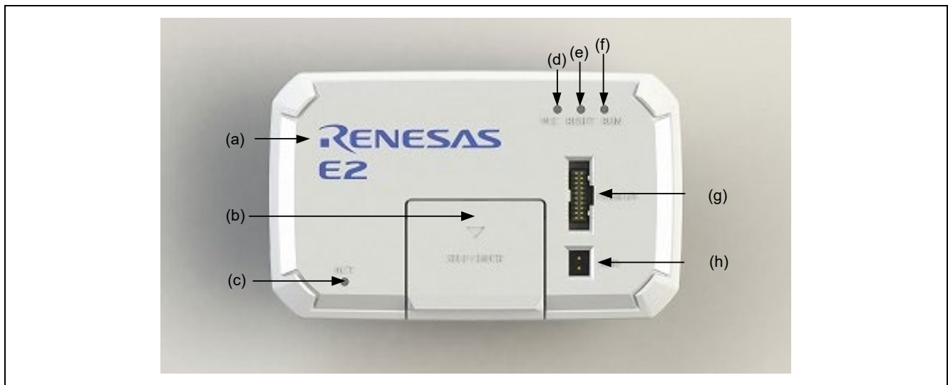
Figure 1.3 E2 Top View
