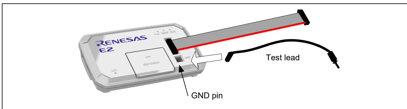
Figure 2.5 Connecting a User-System Interface Cable and a Test Lead on the E2
