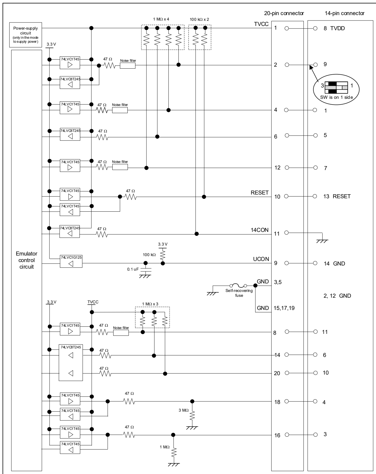
Figure C.2 Interface Circuits in the E2 Emulator (Rev. D or Later)
