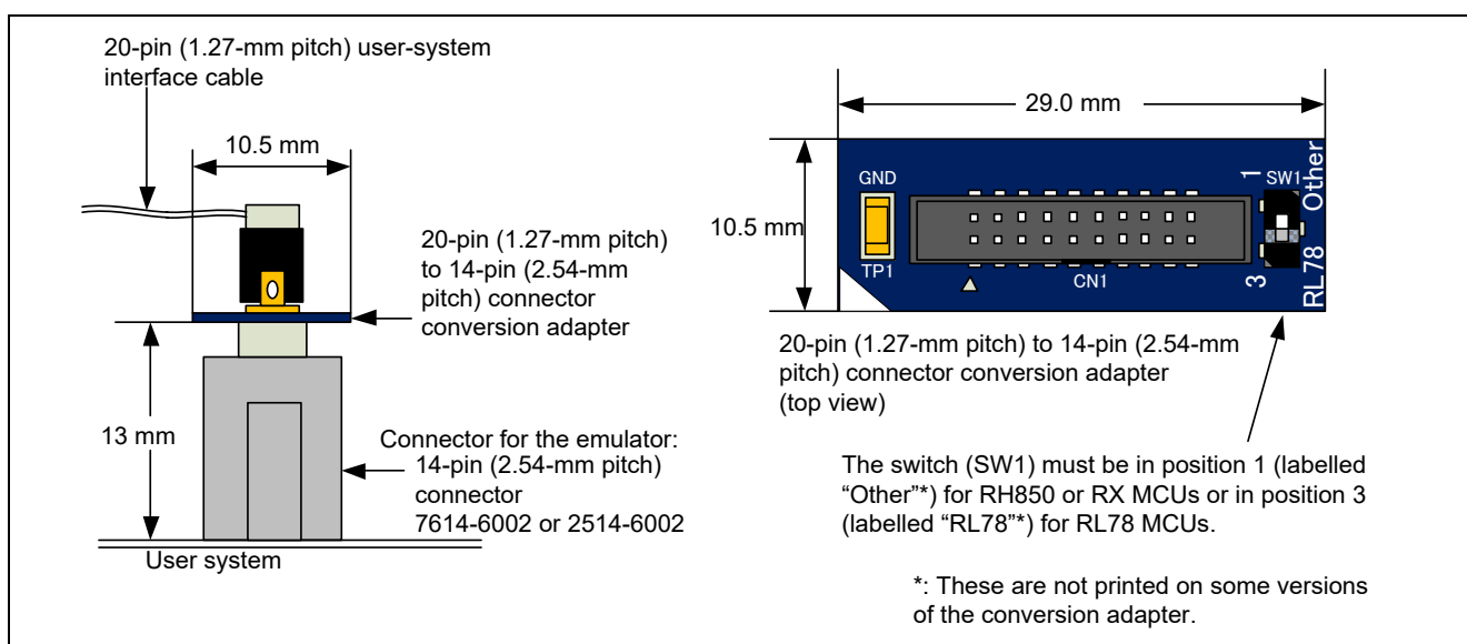
Figure 2.4 Connecting the User-System Interface Cable to the 14-Pin (2.54-mm Pitch) Connector on the User System
