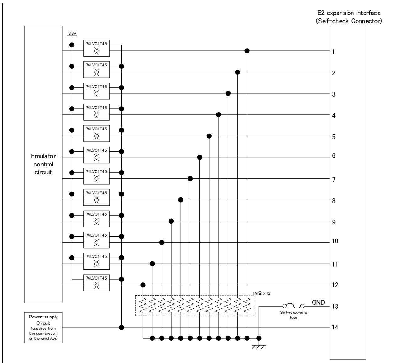
Figure B.2 Internal Circuits of the E2 Expansion Interface
