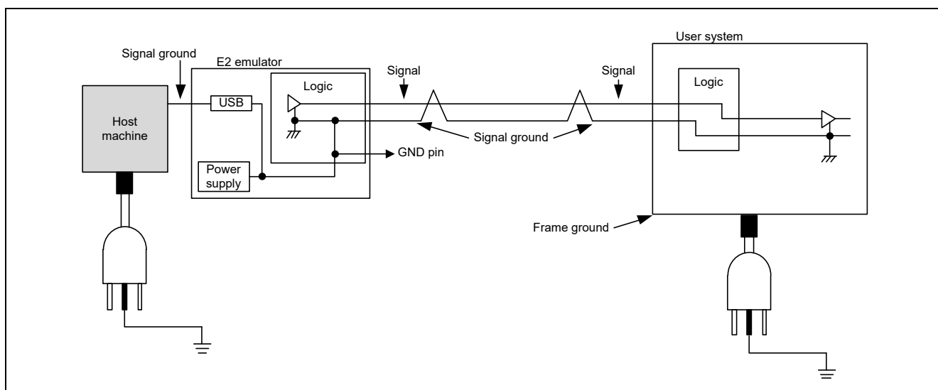
Figure 2.8 Connecting System Ground
