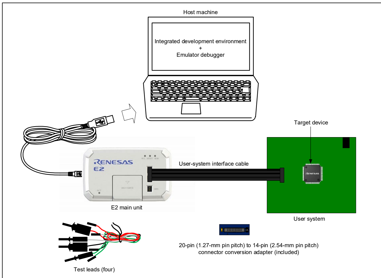
Figure 1.1 System Configuration of E2
