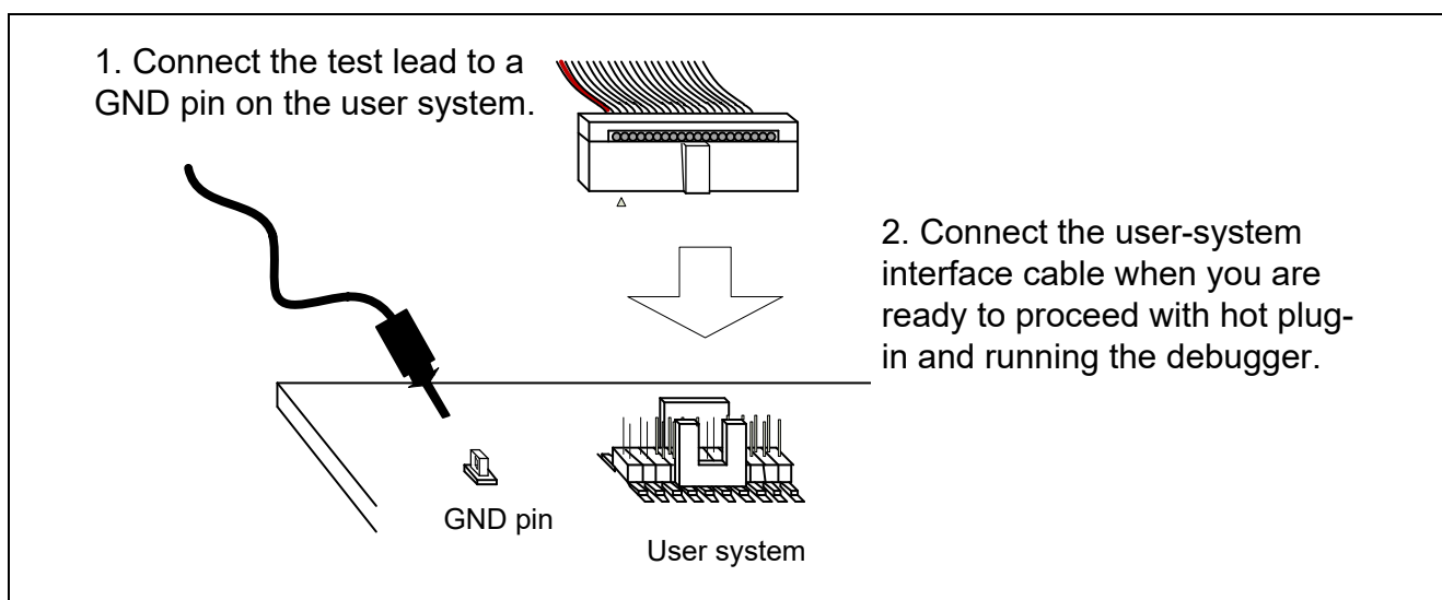
Figure 2.7 Hot Plug-in Connection (when the Conversion Adapter is not in Use)
