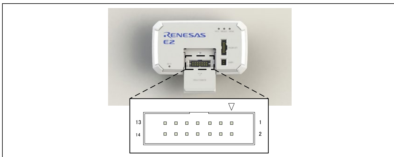
Figure B.1 Pin Alignment of the E2 Expansion Interface (Self-check) Connector
