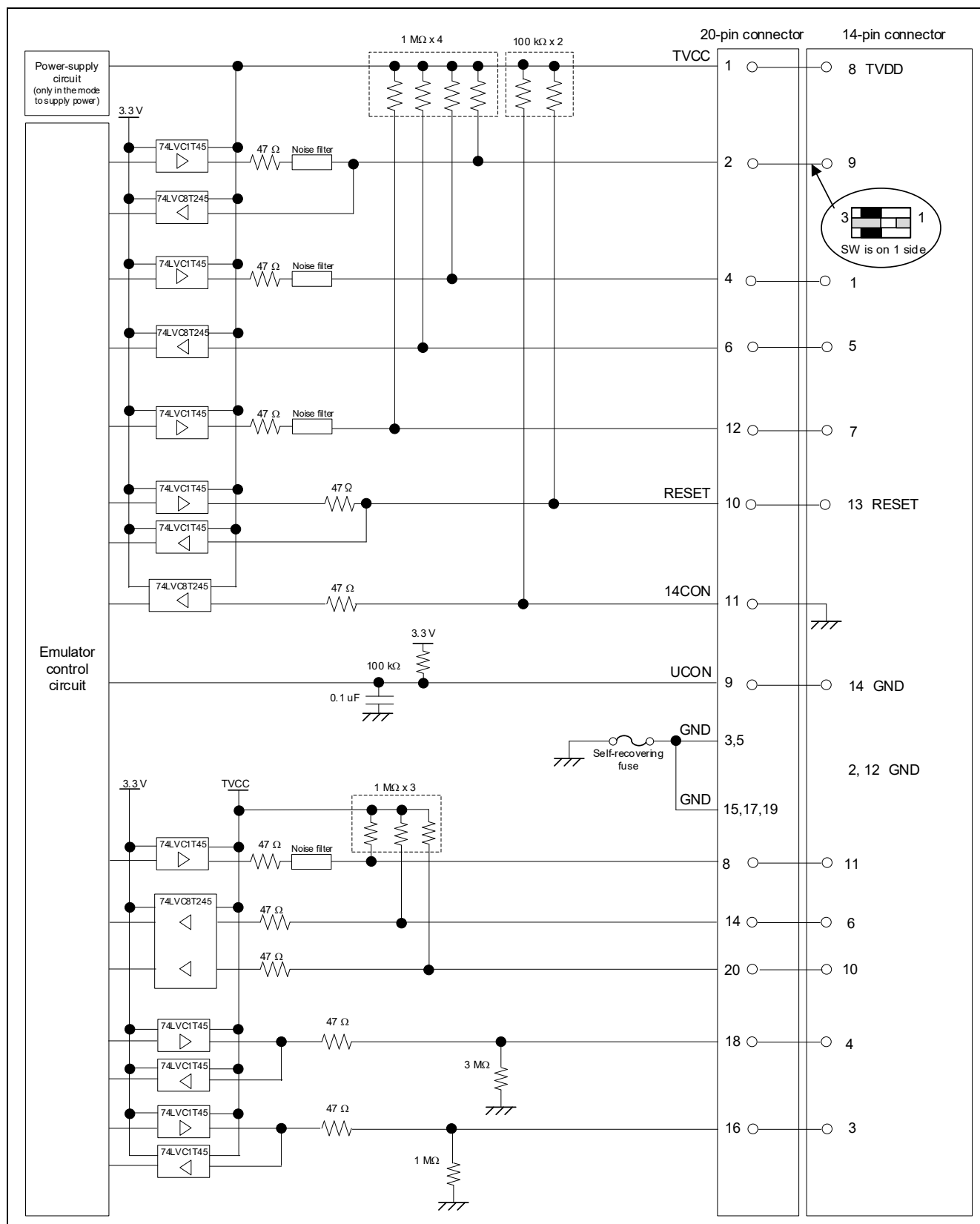
Figure C.1 Interface Circuits in the E2 Emulator (Rev. C)
