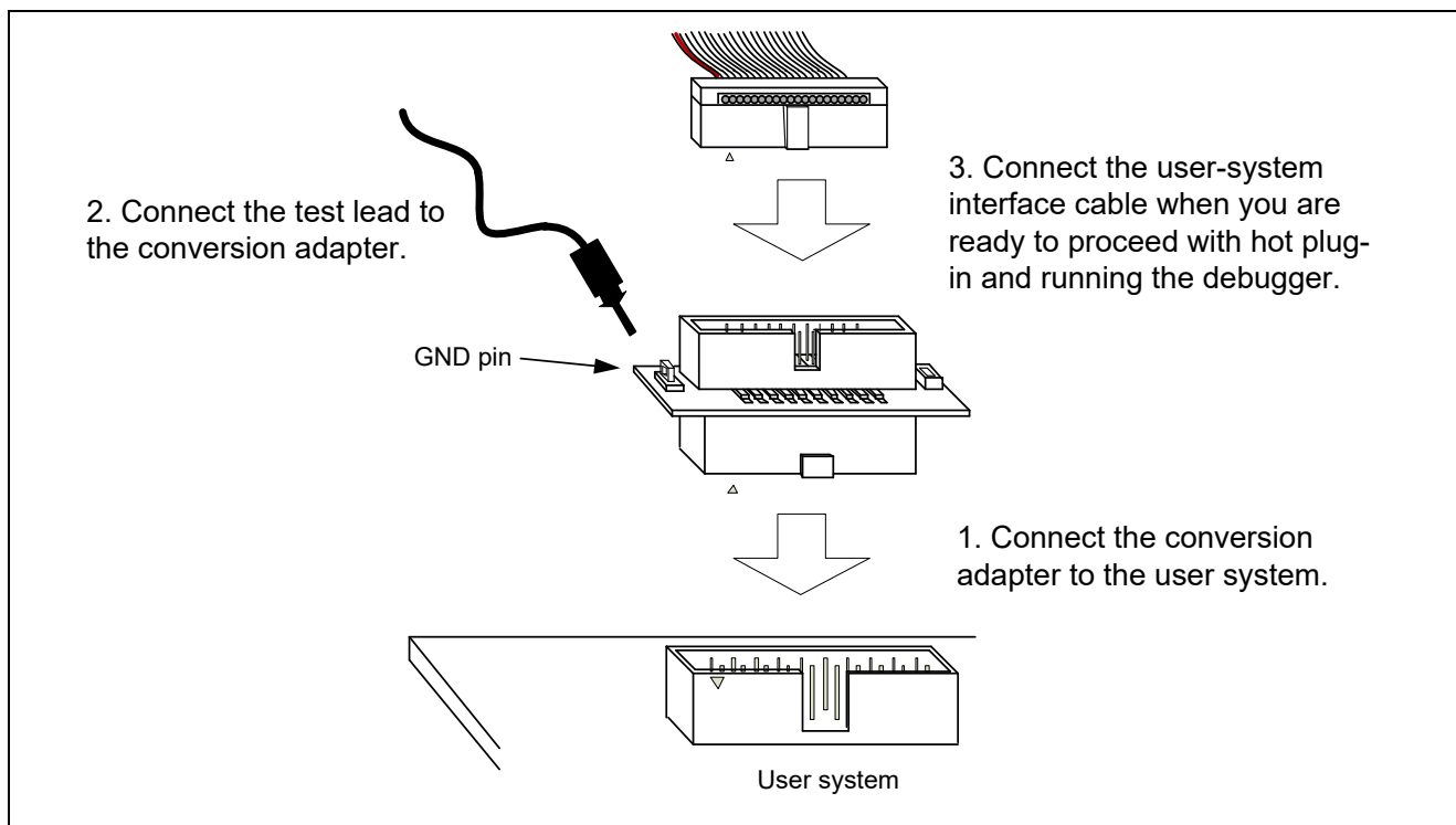
Figure 2.6 Hot Plug-in Connection
