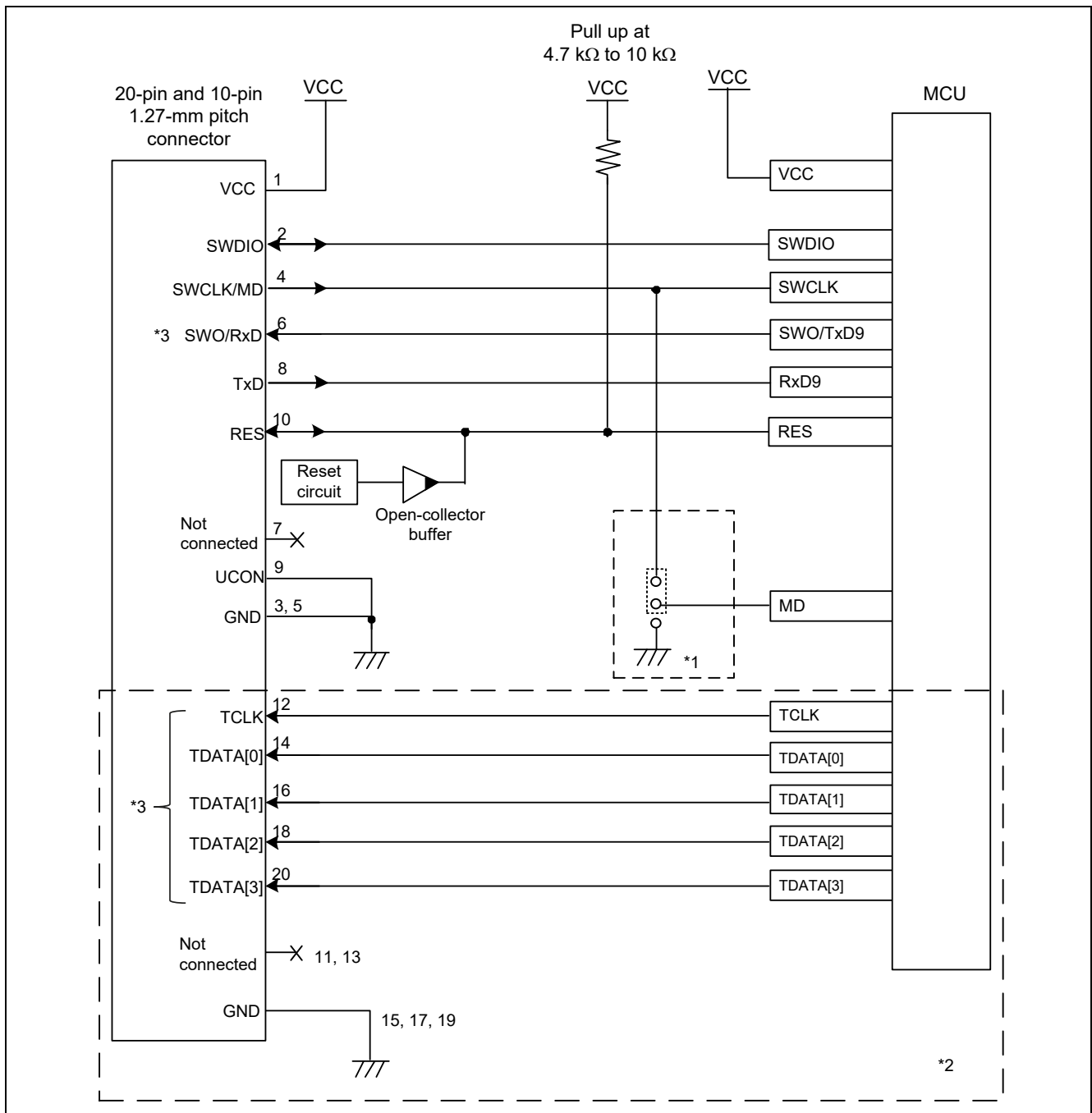
Figure 2.4 Example of a Connection through SWD and SCI Interfaces
