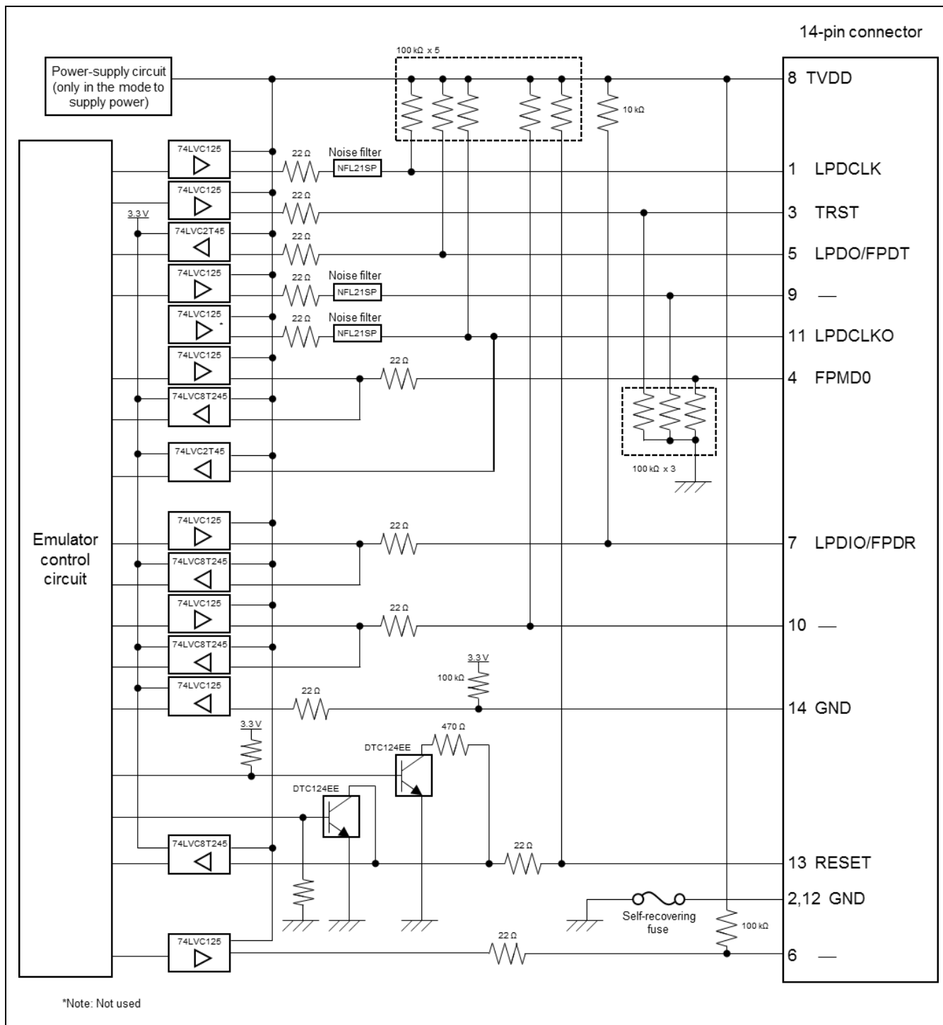
Figure 5-1 Interface Circuits in the E1 or E20 Emulator (4-Pin LPD, 2-Wire UART)
