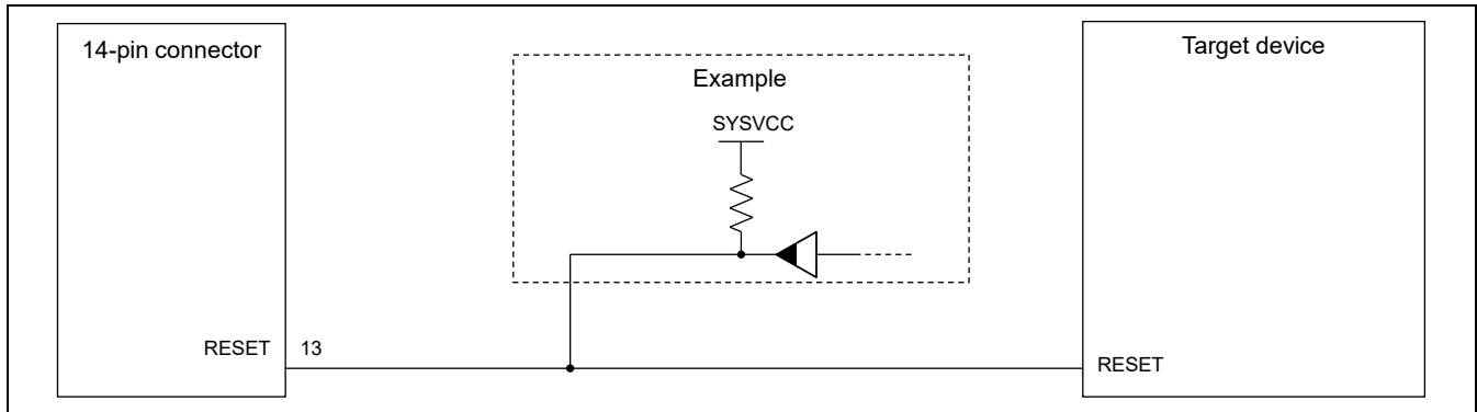
Figure 2-7 Example of Connecting a Reset Circuit
