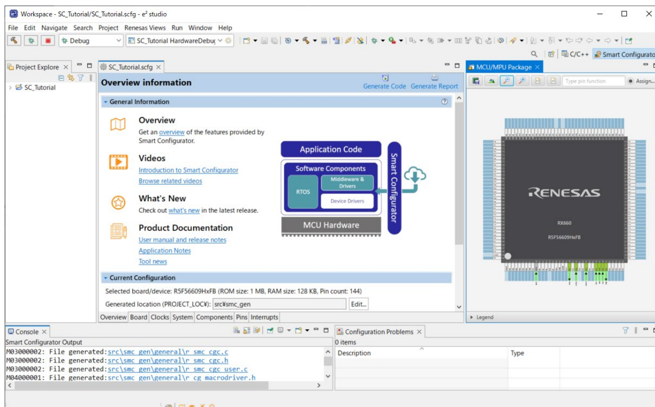
Figure 4-1 Overview page
