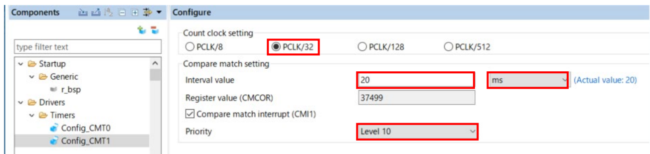
Figure 4-17 Config_CMT1 setting
