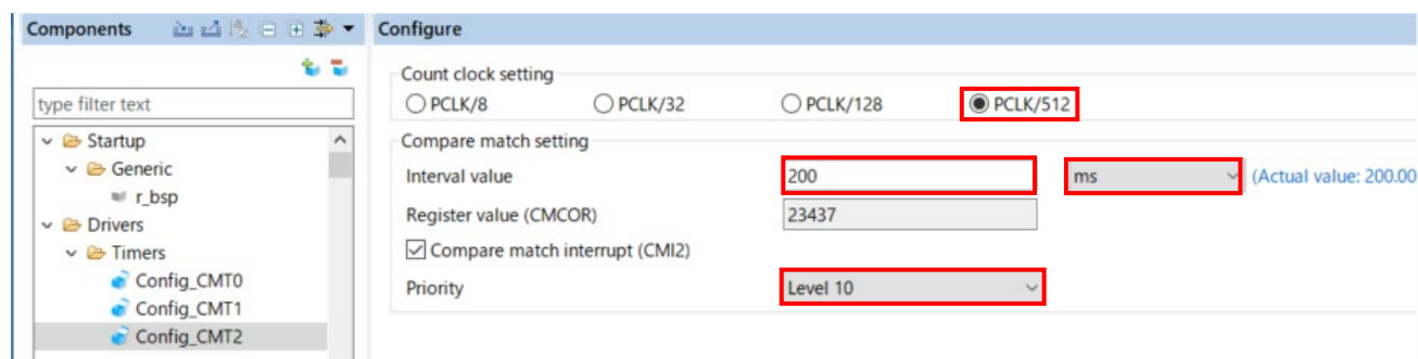
Figure 4-20 Config_CMT2 setting
