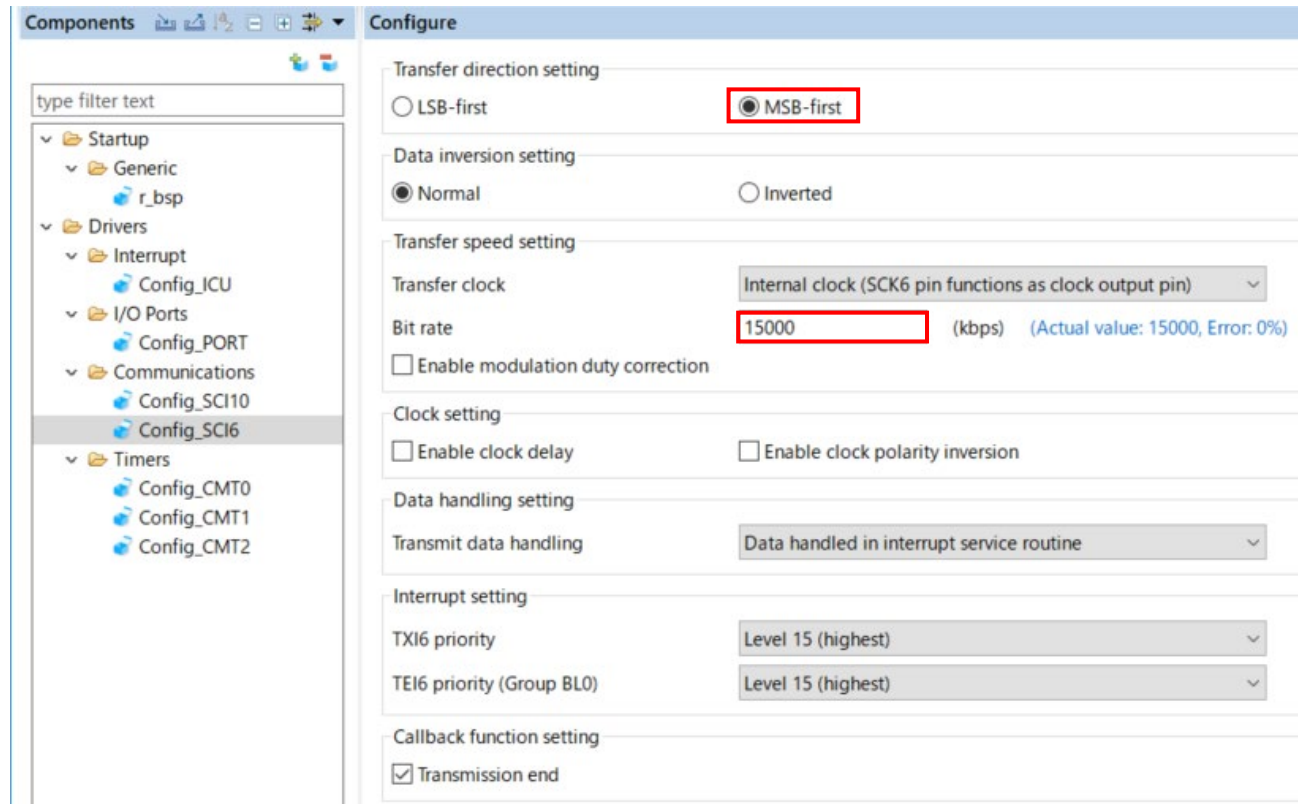
Figure 4-42 Config_SCI6 setting
