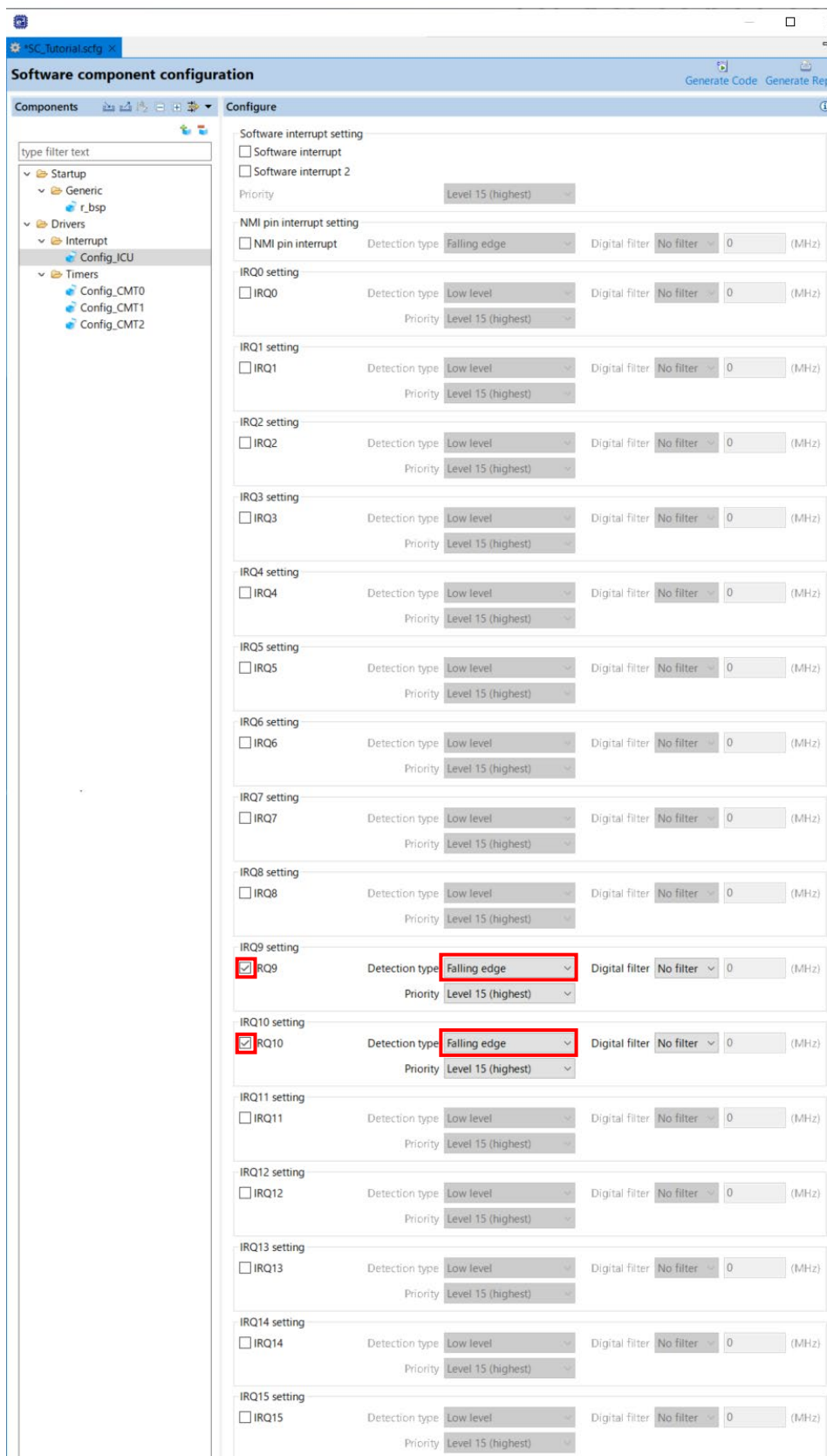
Figure 4-23 Config_ICU setting
