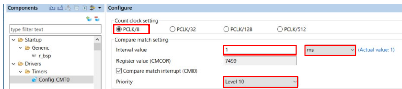
Figure 4-13 Config_CMT0 setting
