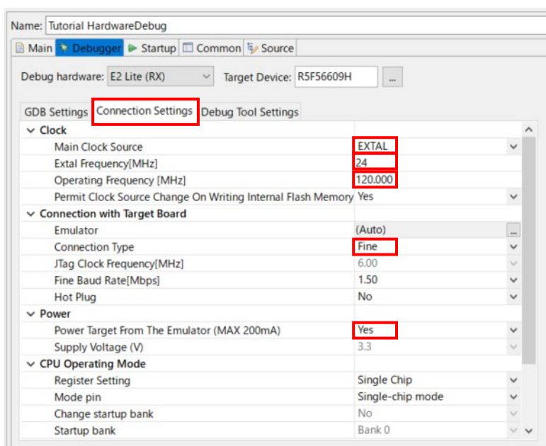
Figure 6-2 Connection Settings
