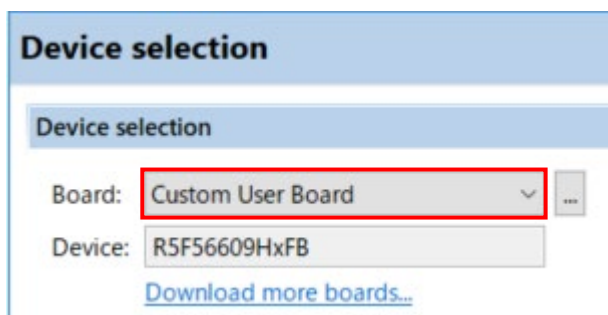
Figure 4-3 Select board
