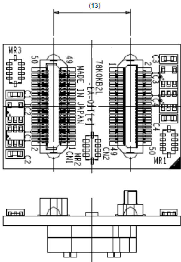
< Top view >
