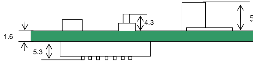
< Side view >
